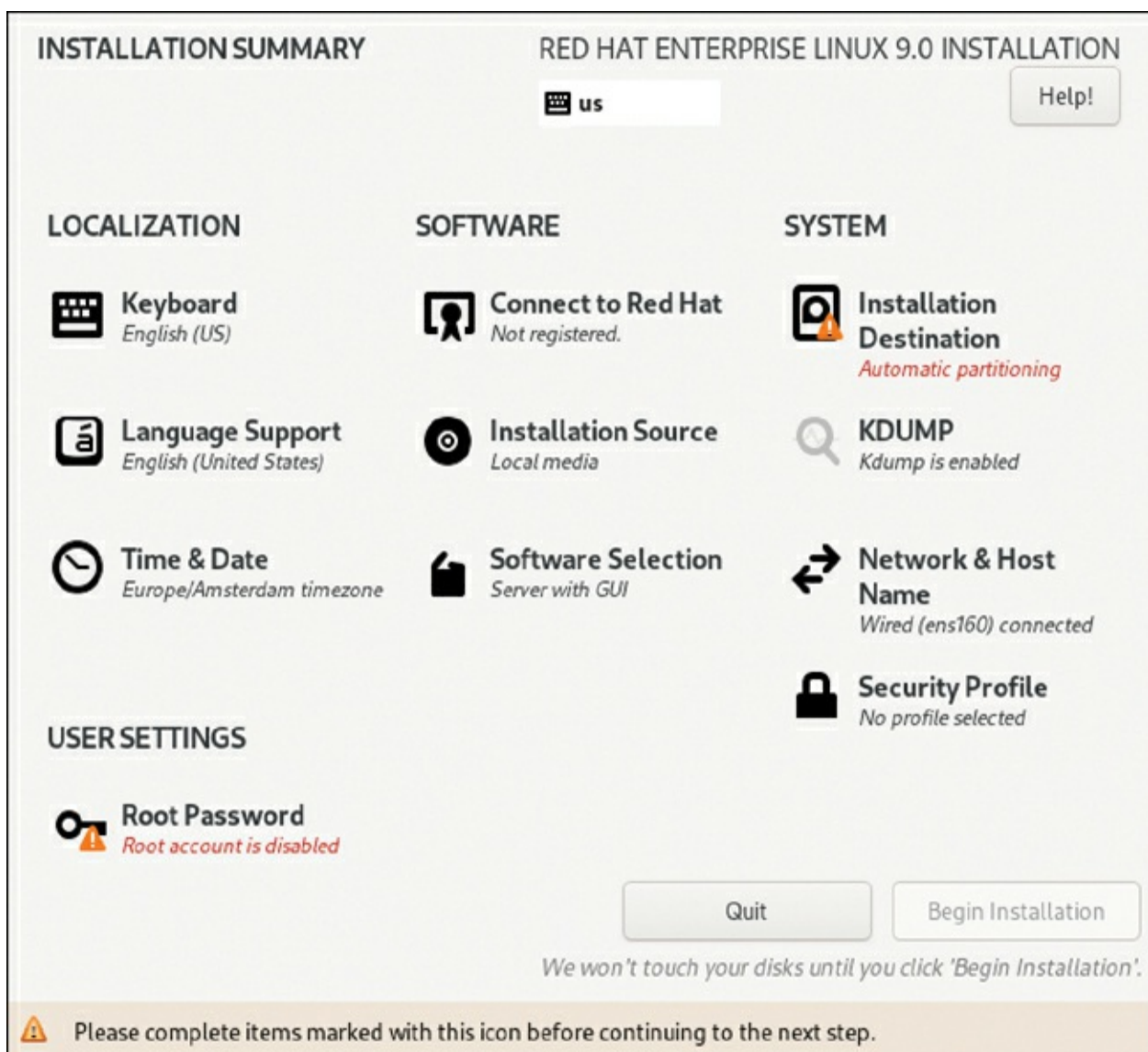
Figure 1-3 Specify the Complete Configuration of Your Server from the Installation
