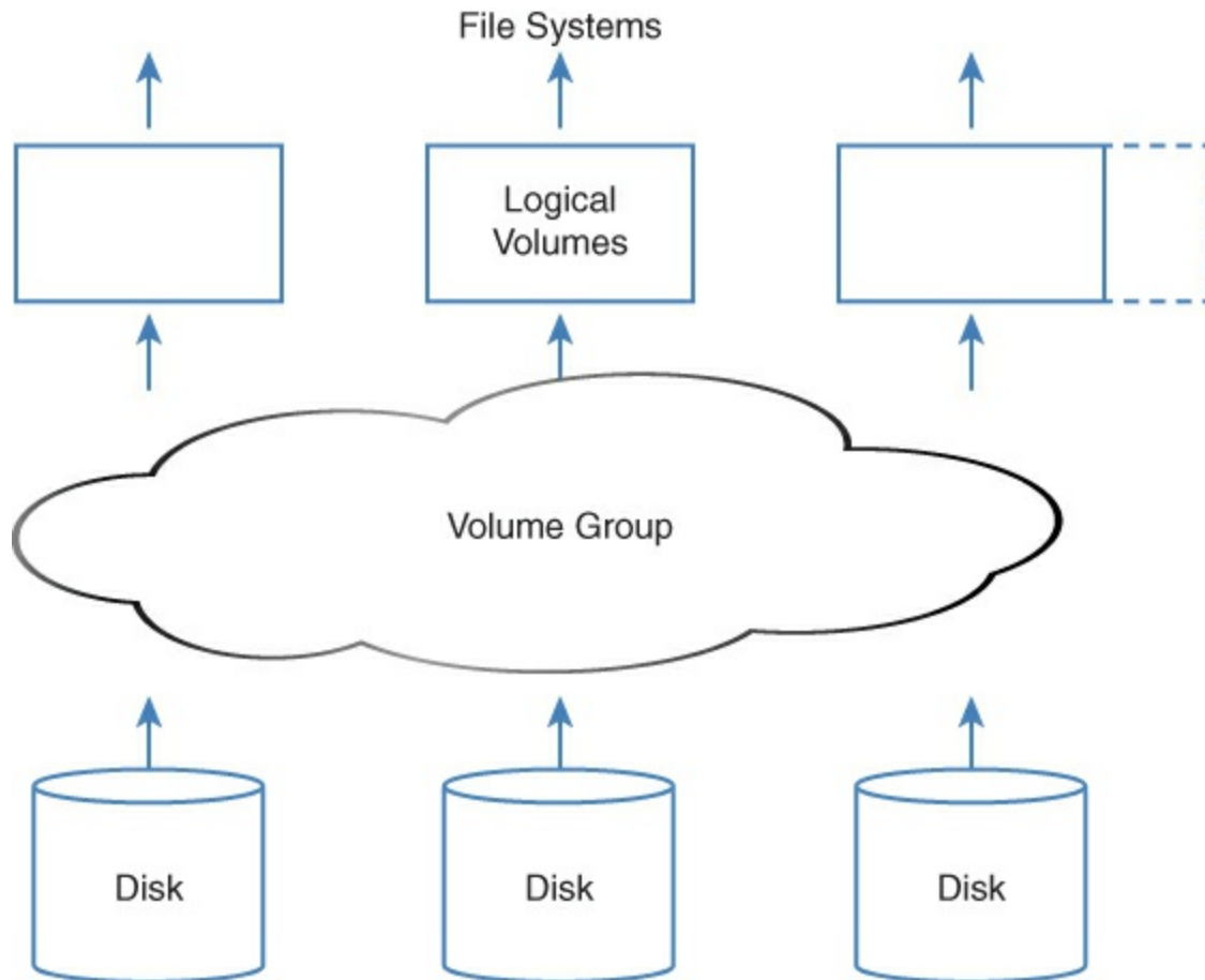
Figure 15-1 LVM Architecture Overview
