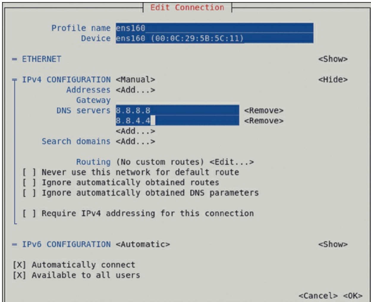
Figure 8-5 Setting DNS Servers from the nmtui Interface
