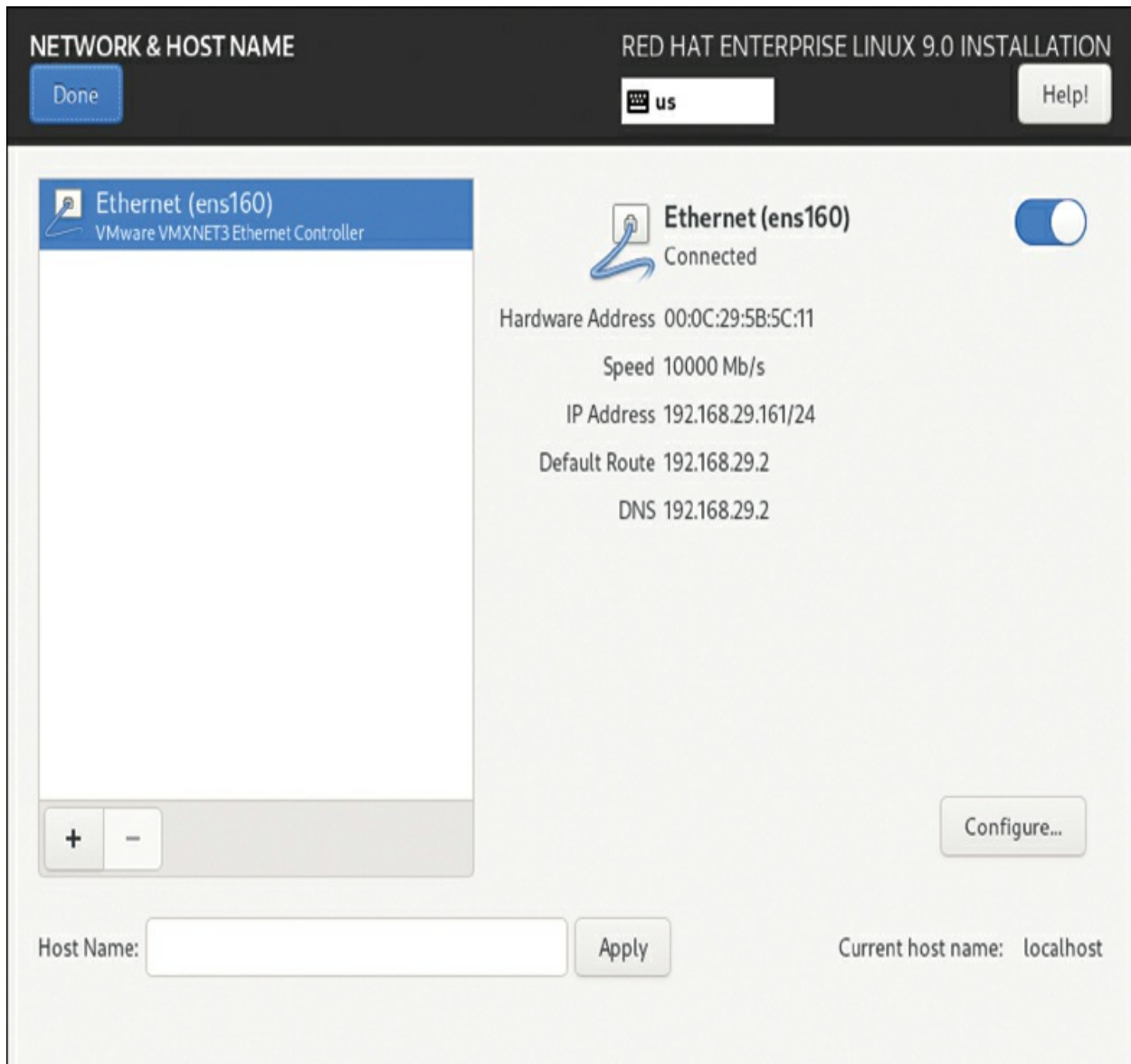
Figure 1-10 On the Network & Host Name Screen, Ensure the Network Card Is Connected
