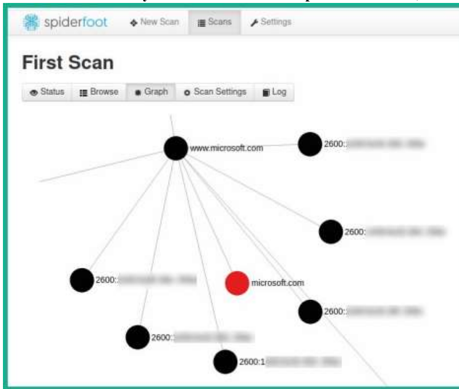
Figure 5.25 – Spiderfoot graph
