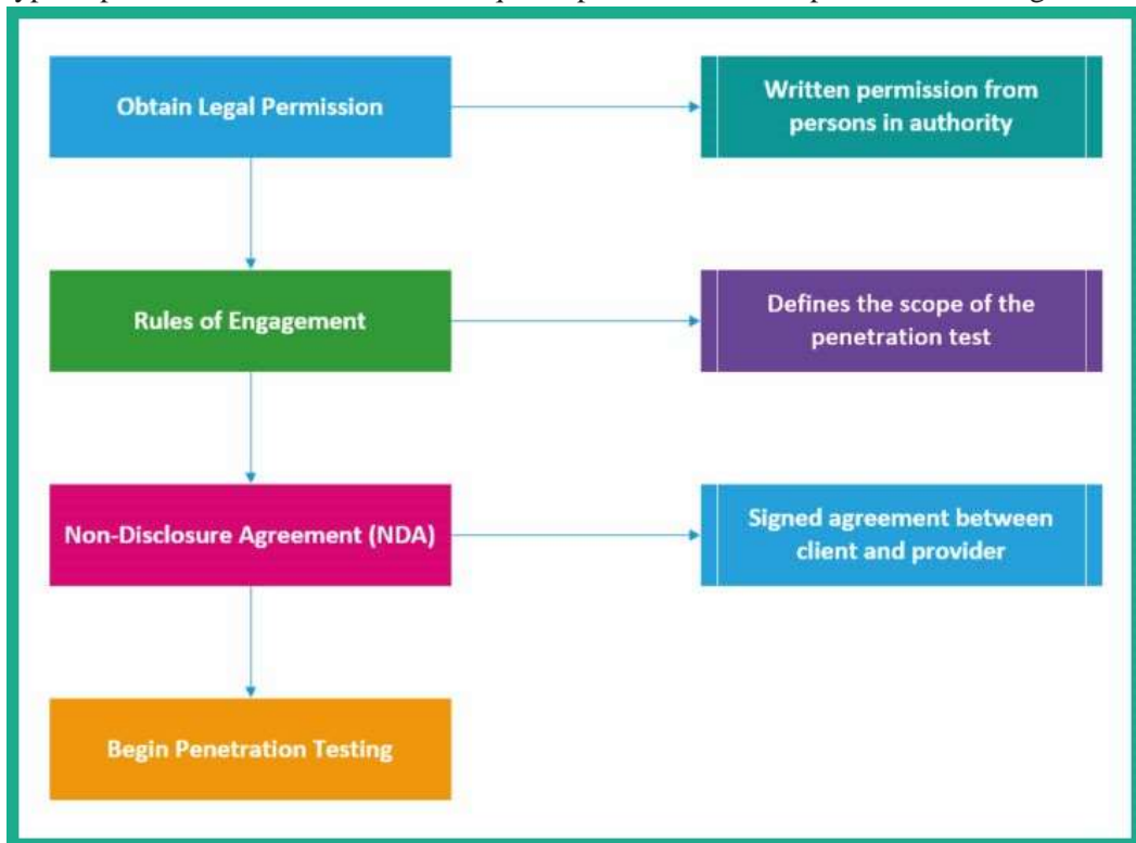
Figure 1.2 – Pre-engagement
