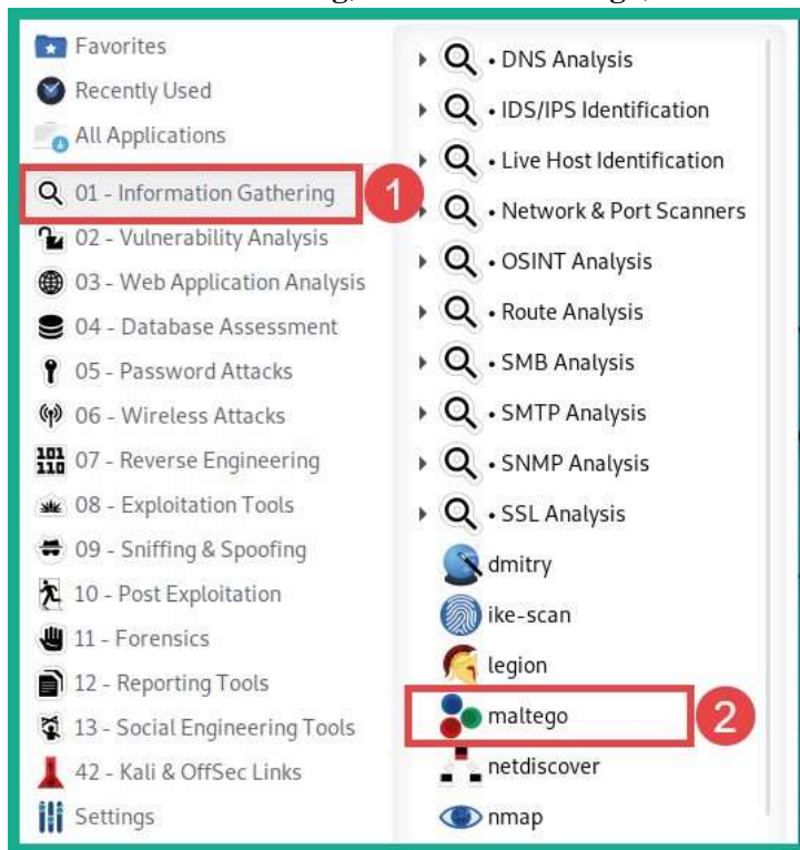
Figure 4.44 – Opening Maltego
