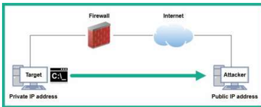
Figure 7.4 – Reverse shell
