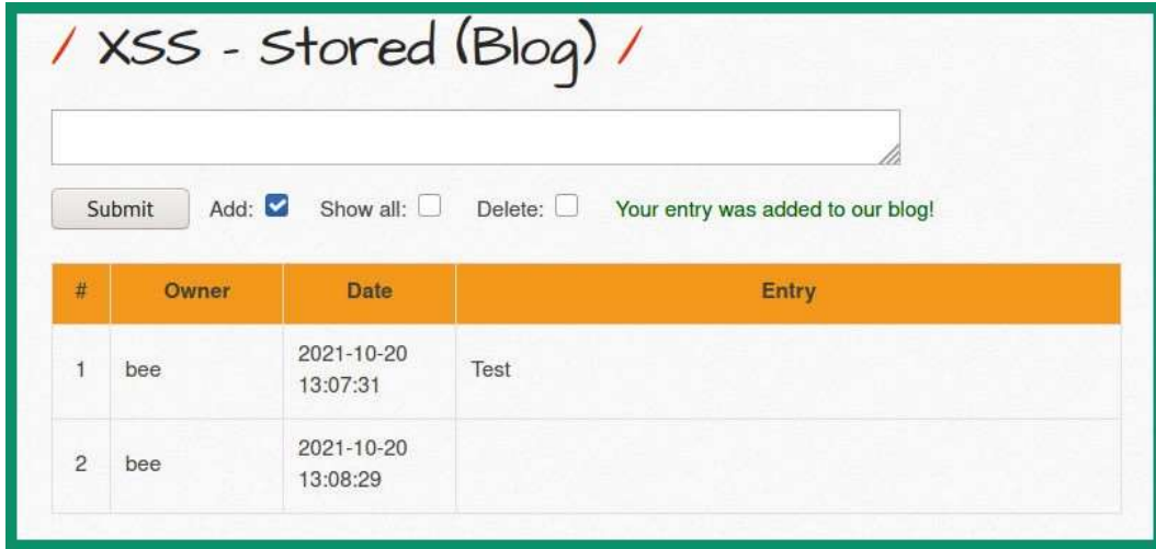
Figure 16.45 – Invisible entry
