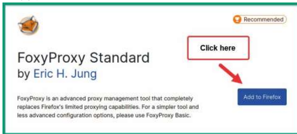
Figure 15.5 – FoxyProxy
