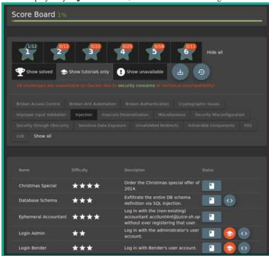
Figure 15.22 – Filtering challenges
