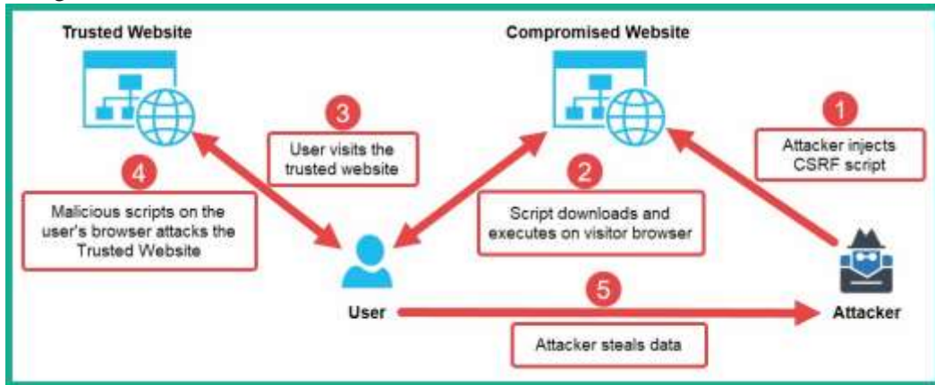
Figure 16.35 – CSRF attack
