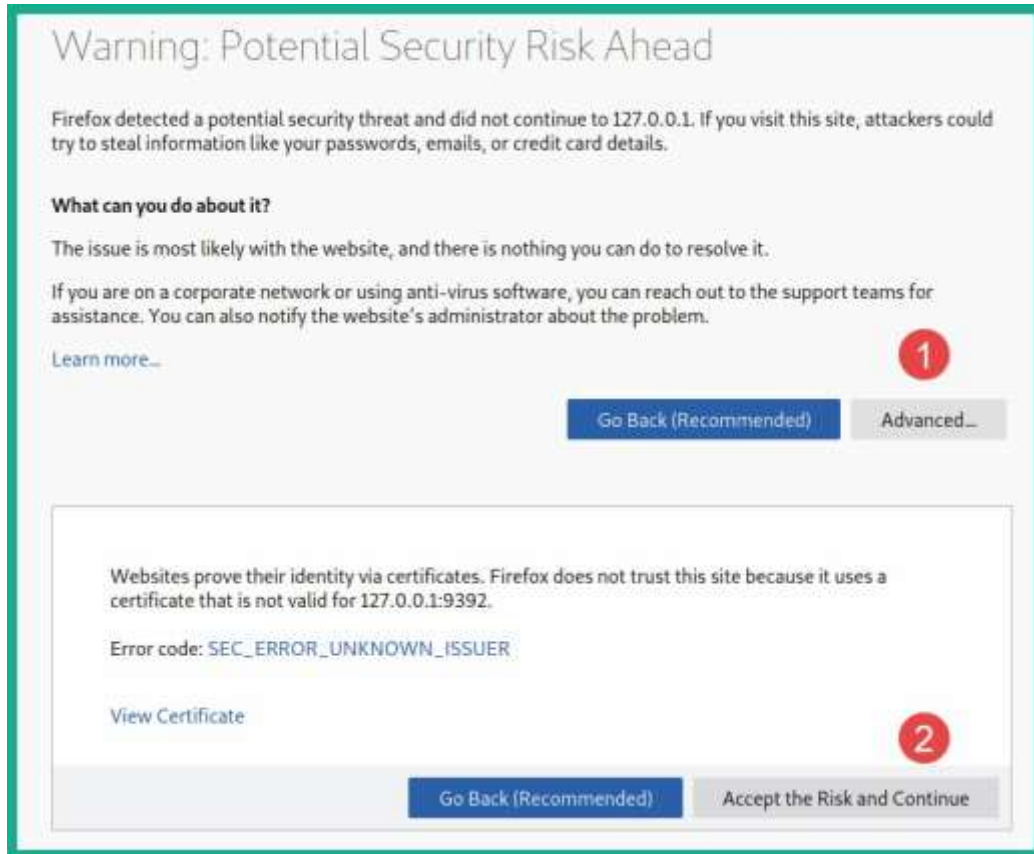
Figure 6.31 – Security warning
