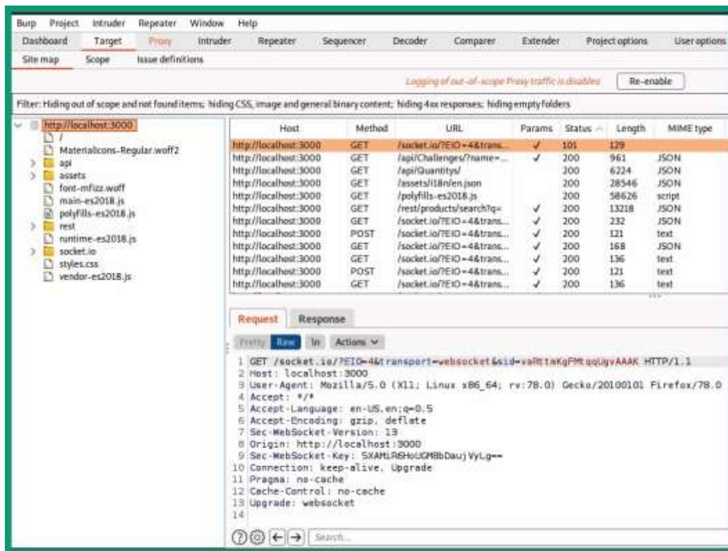
Figure 15.16 – Passive crawling
