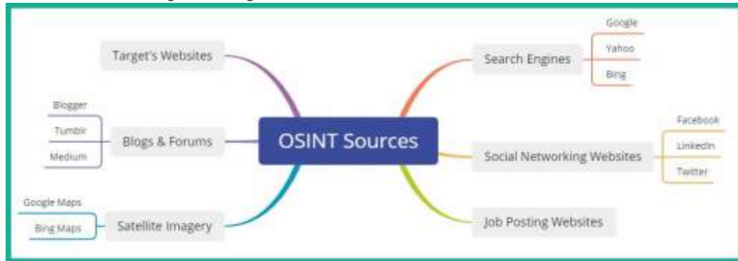
Figure 4.2 – OSINT sources
