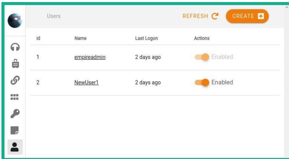
Figure 12.29 – User accounts
