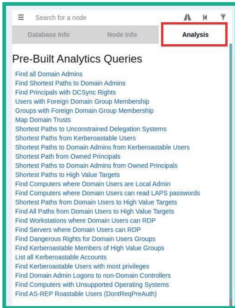
Figure 10.24 – Analytics templates
