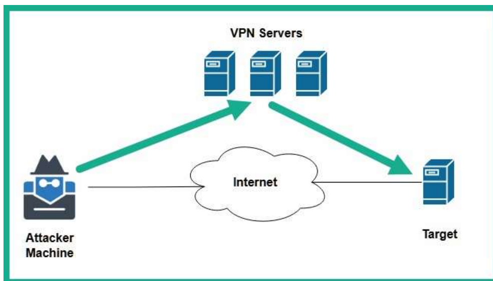
Figure 4.3 – VPN servers
