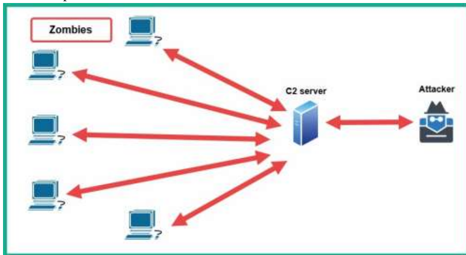
Figure 1.7 – C2 operations
