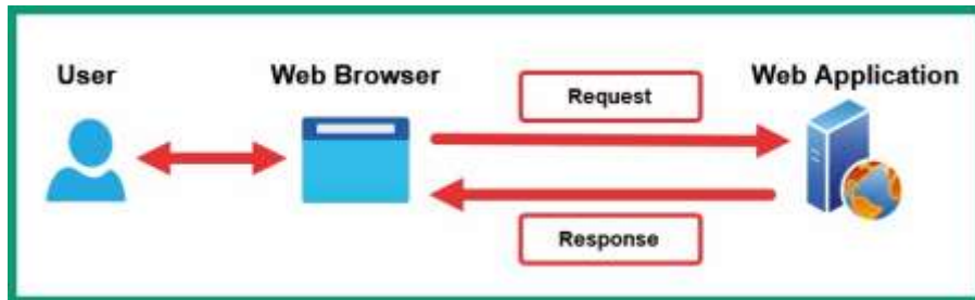
Figure 15.1 – Web application
