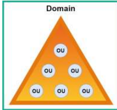
Figure 10.1 – Domain structure
