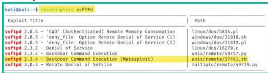
Figure 6.25 – Searchsploit
