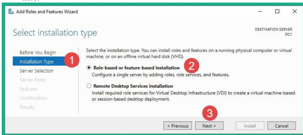
Figure 3.11 – Installation Type
