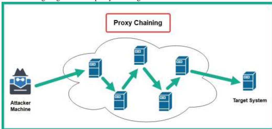
Figure 4.4 – Proxy chaining
