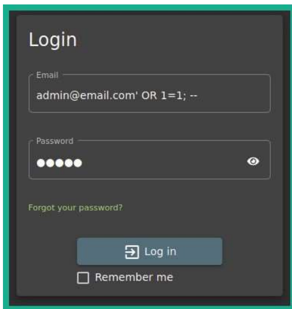
Figure 15.27 – SQL injection
