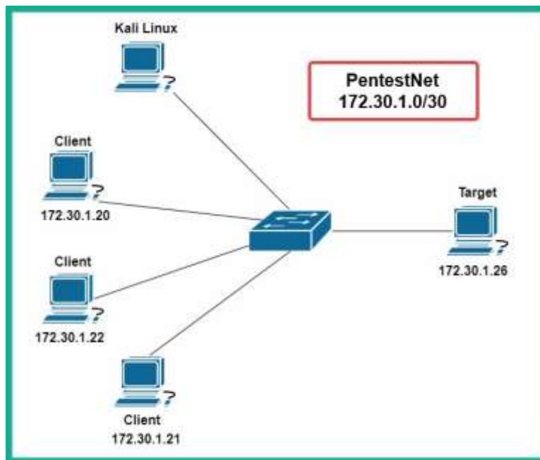
Figure 5.41 – Decoys
