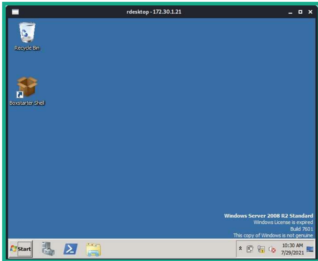
Figure 8.10 – RDP session
