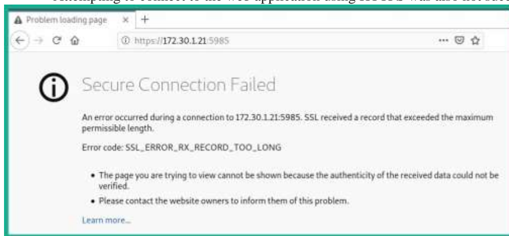
Figure 8.39 – Checking HTTPS
