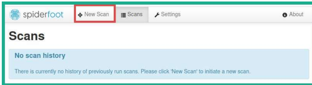
Figure 5.22 – New Scan
