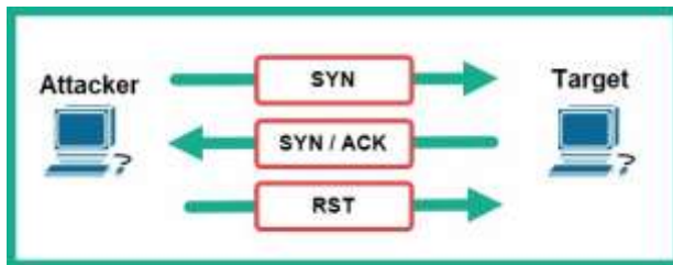
Figure 5.43 – Stealth scan
