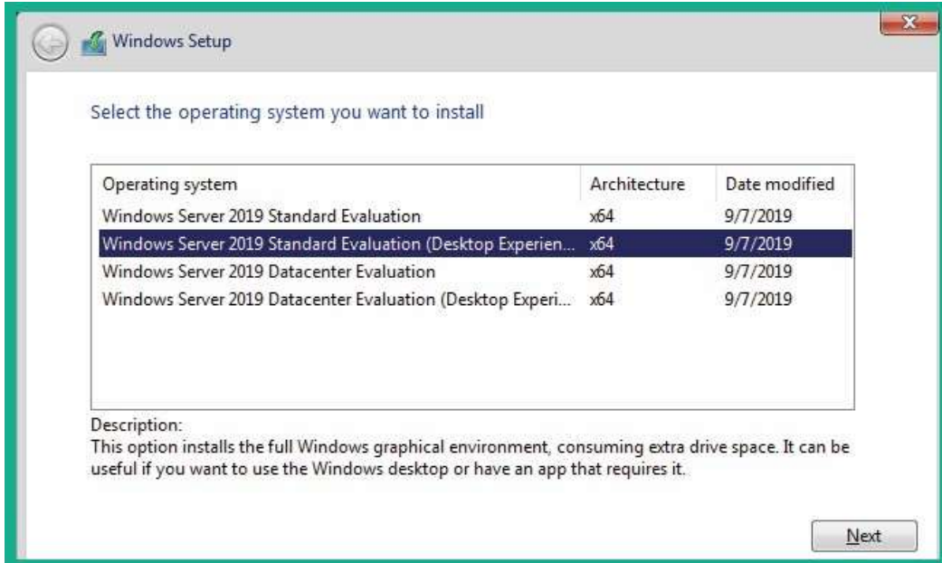
Figure 3.3 – Windows Setup
