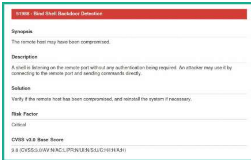
Figure 6.22 – Custom report
