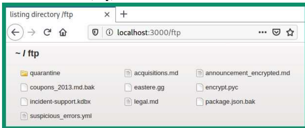
Figure 16.1 – Insecure directory
