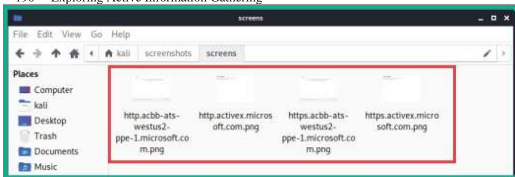
Figure 5.30 – Screenshots
