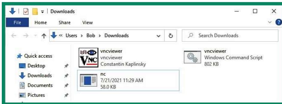
Figure 9.30 – Reassembled file
