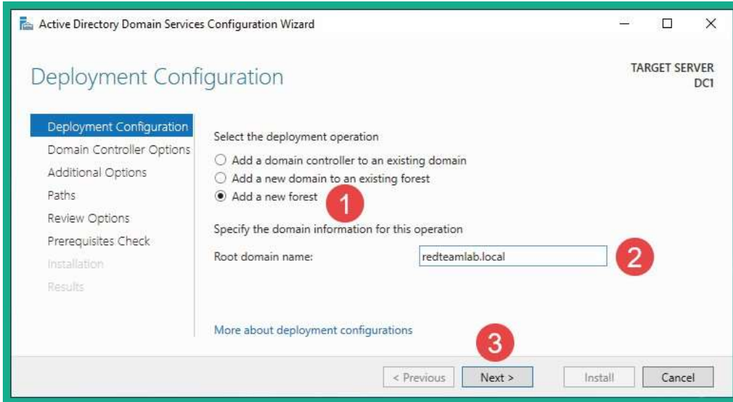
Figure 3.13 – Deployment Configuration
