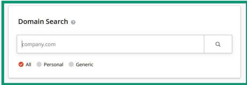
Figure 4.15 – Hunter.io
