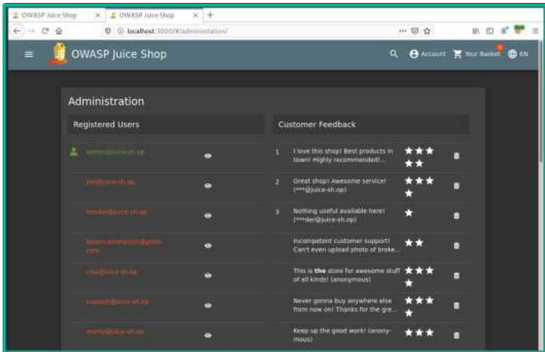
Figure 15.34 – Administration section
