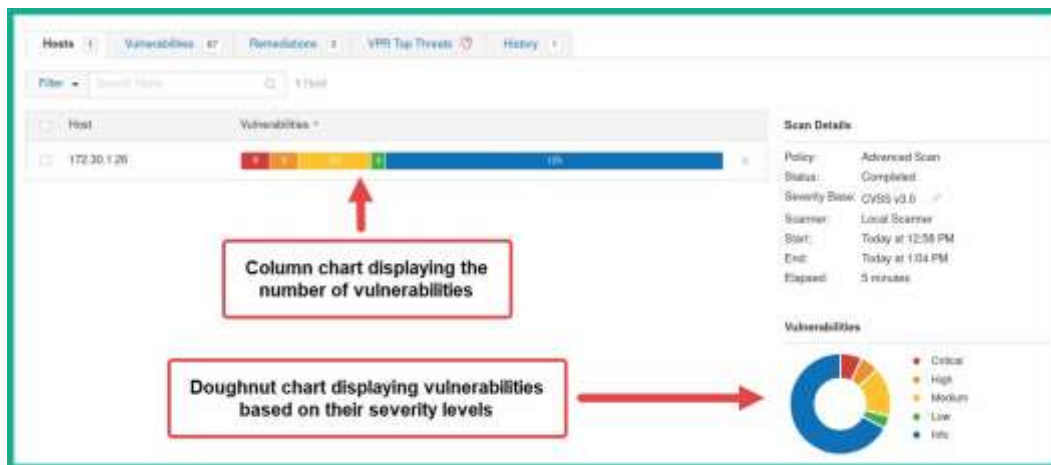
Figure 6.13 – Scan results
