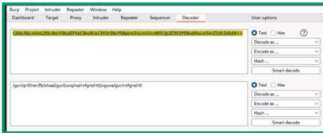
Figure 15.40 – Decoding Base64
