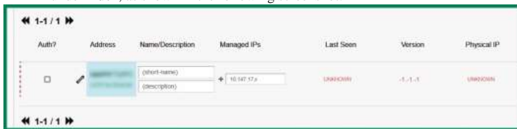
Figure 17.11 – Member
