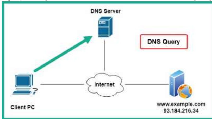
Figure 5.10 – DNS query
