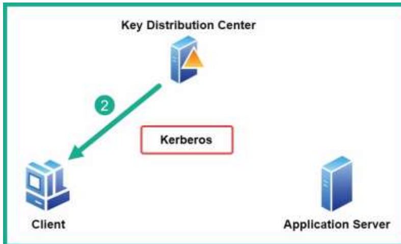
Figure 11.2 – Phase 2
