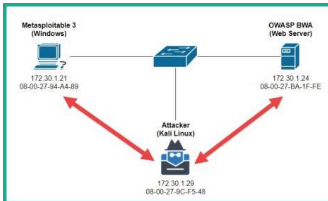
Figure 9.48 – MITM attack
