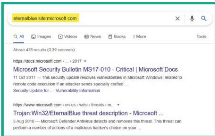
Figure 5.2 – Keyword search
