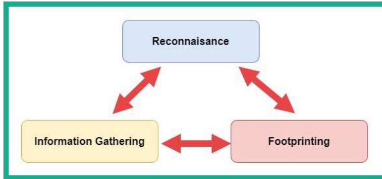
Figure 4.1 – Footprinting
