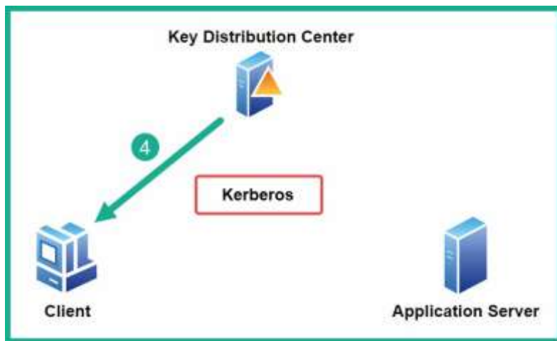
Figure 11.4 – Phase 4
