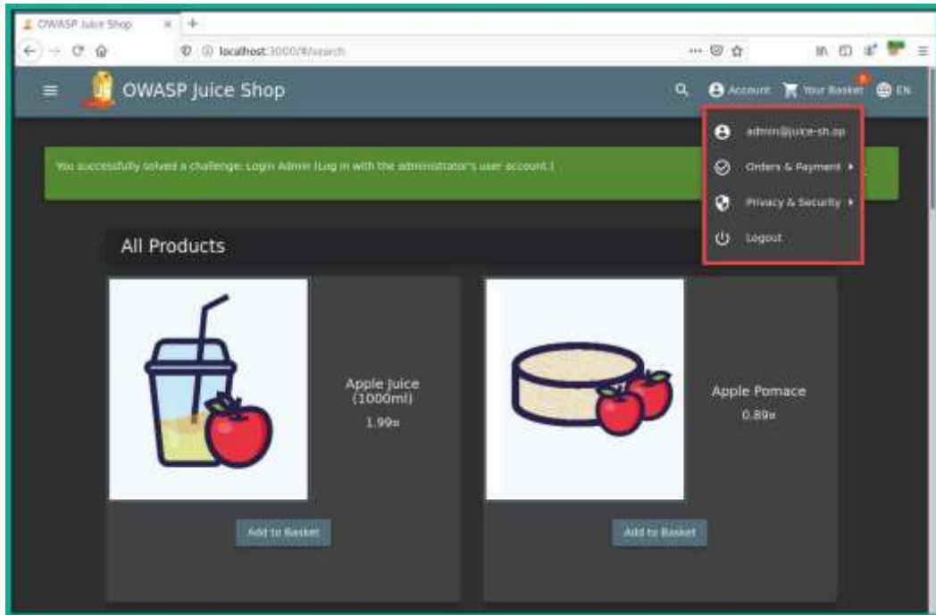
Figure 15.30 – Gaining access
