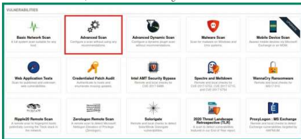
Figure 6.10 – Scanning templates
