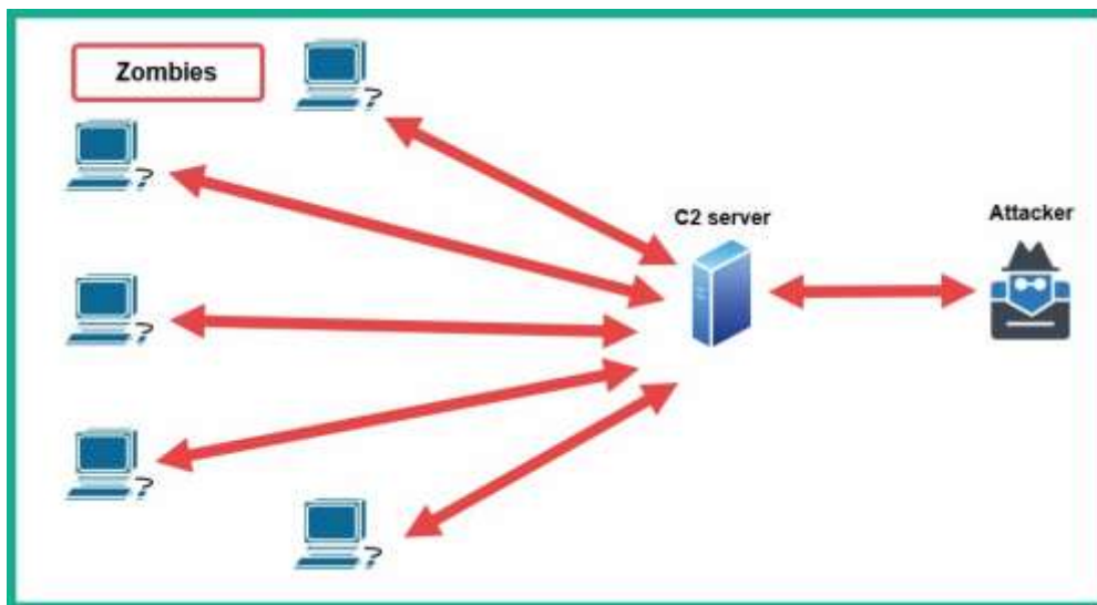
Figure 12.1 – C2 operations
