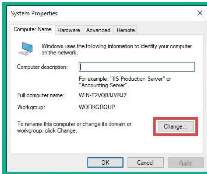
Figure 3.7 – System Properties
