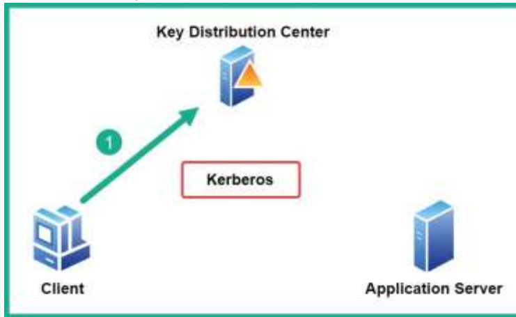
Figure 11.1 – Phase 1
