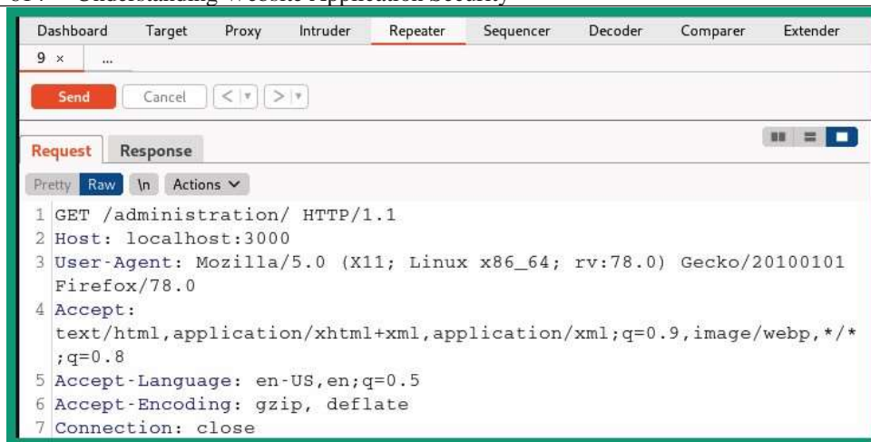
Figure 15.32 – Modifying headers
