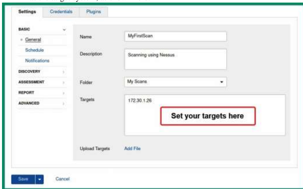
Figure 6.11 – Scan options
