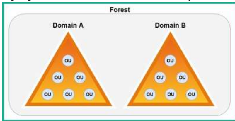
Figure 10.2 – Forest
