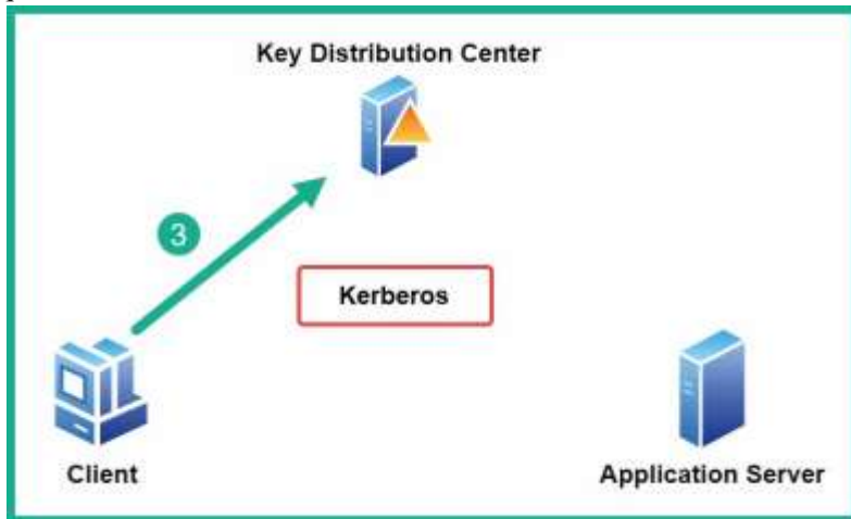
Figure 11.3 – Phase 3
