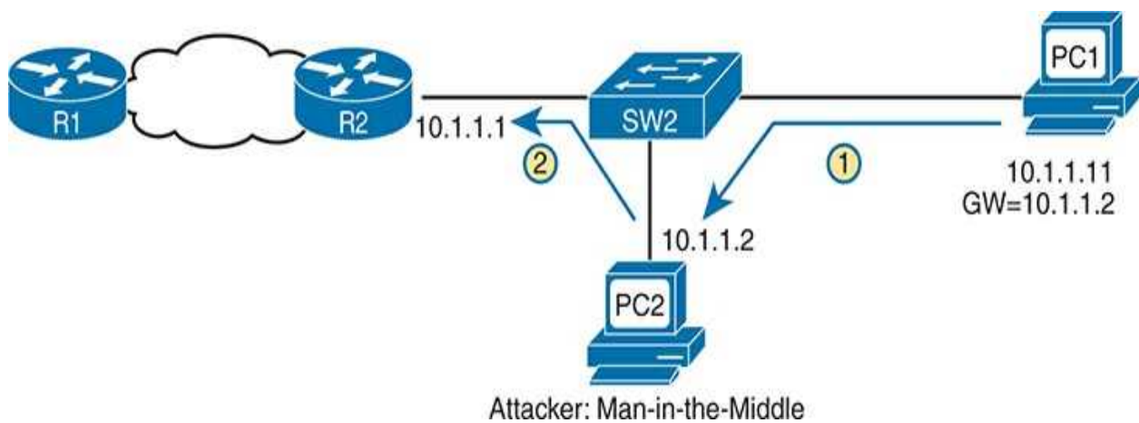
Figure 12-2 DHCP Attack Supplies Good IP Address but Wrong Default Gateway
