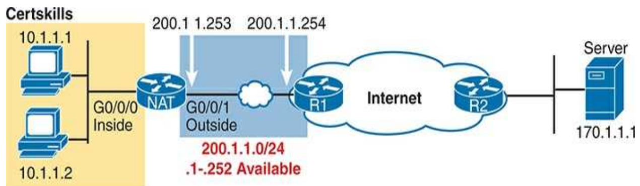
Static NAT Configuration
