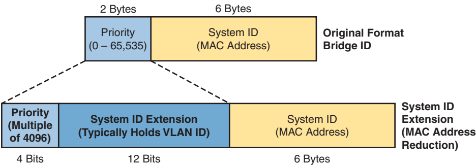
Figure 10-4 STP System ID Extension
