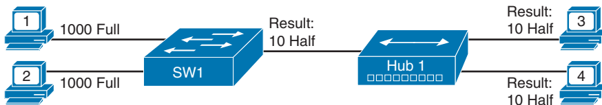
Figure 7-3 IEEE Autonegotiation with a LAN Hub
