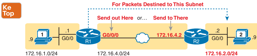
Figure 17-13 Static Route Configuration Concept
