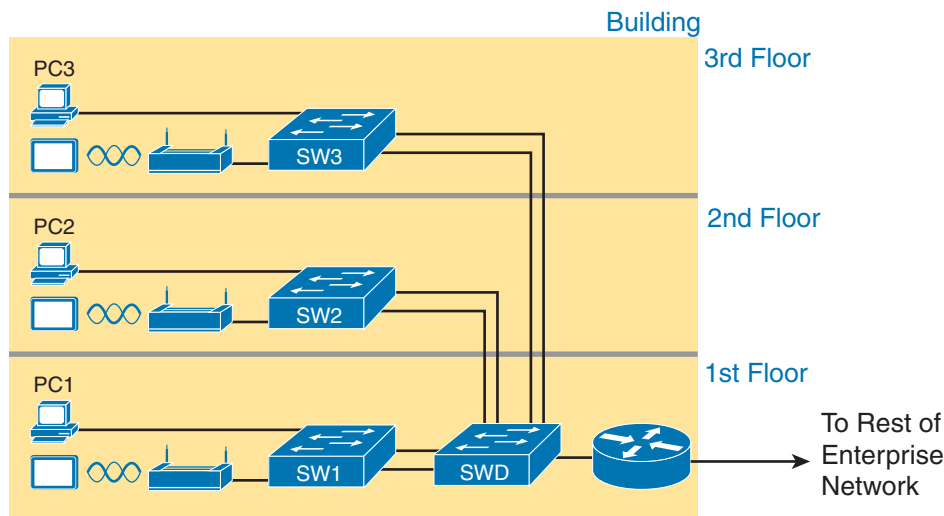
Figure 2-3 Single-Building Enterprise Wired and Wireless LAN
