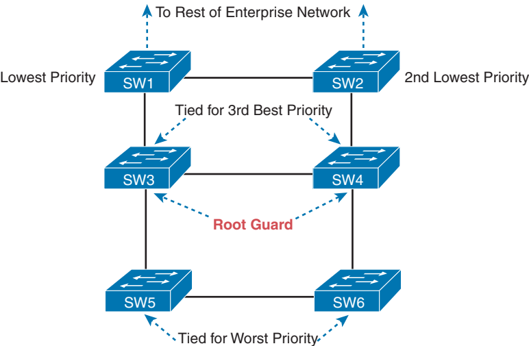
Figure 9-17 Larger LAN Showing Most and Least Likely Root Switches
