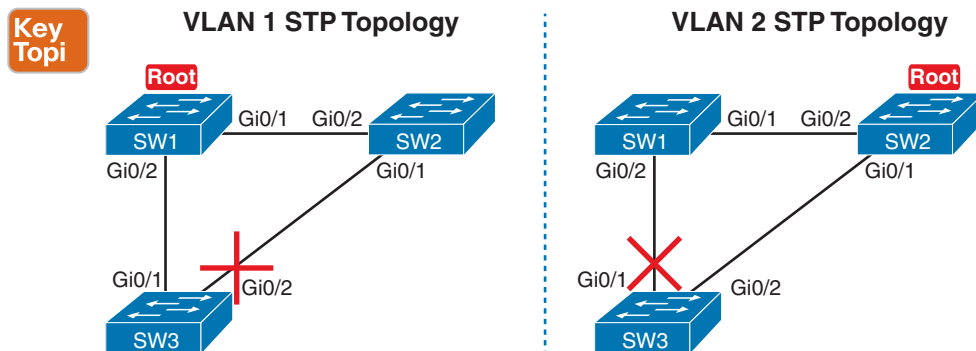
Figure 10-2 Load Balancing with One Tree for VLAN 1 and Another for VLAN 2
