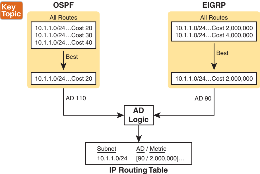
Figure 24-4 Logic: Choosing the Lowest AD Route Between OSPF and EIGRP Next, the routers need to learn routes from both companies. The EIGRP routers on the left need to learn the company B routes known to OSPF on the right, and vice versa. To do that, the networking staff uses a feature called route redistribution , in which a small set of routers run both routing protocols . Internal to those routers, the router redistributes (takes routes from one protocol and advertises into the other), taking OSPF routes and advertising those subnets using EIGRP, and vice versa.
