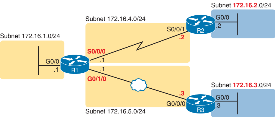
Figure 16-1 Generic Enterprise Network Diagram
