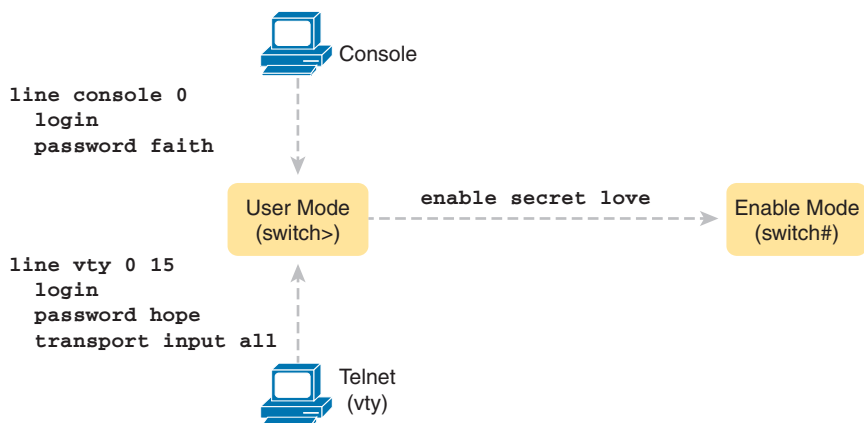
Figure 6-2 Simple Password Security Configuration
