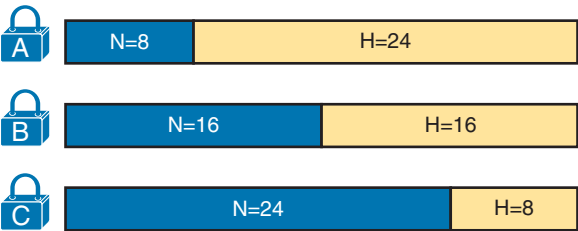
Figure 26-4 Classful View of Unsubnetted IPv4 Networks
