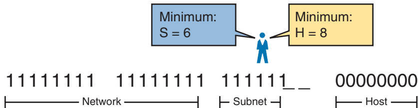
Figure 15-5 Incomplete Mask with N=16, S=6, and H=8
