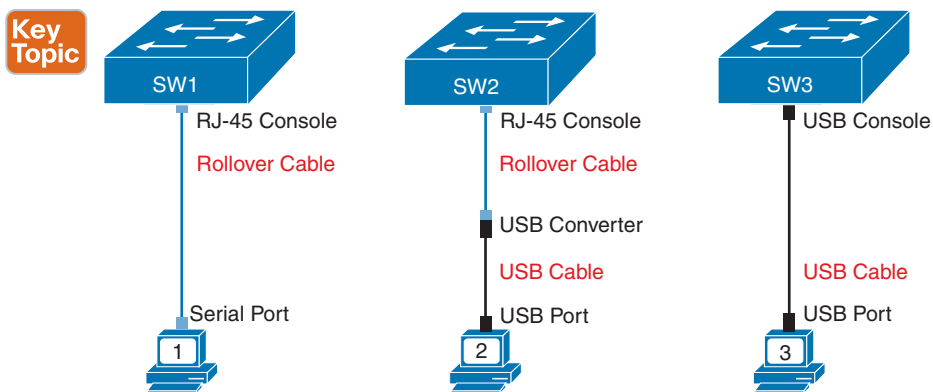
Figure 4-4 Console Connection to a Switch
