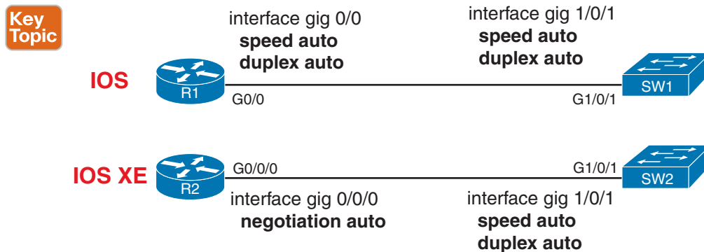
Figure 16-7 Default Ethernet Autonegotiation Configuration: IOS and IOS XE
