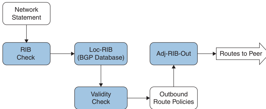
Figure 7-5 BGP Prefix Advertisement
