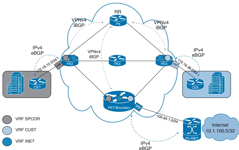
Figure 13-6 MPLS L3VPN Internet Access Option 3
