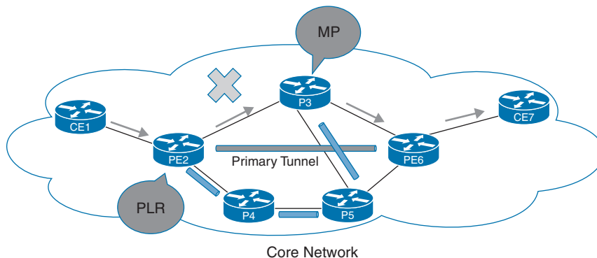
Figure 14-13 MPLS TE FRR: Traffic Rerouting
