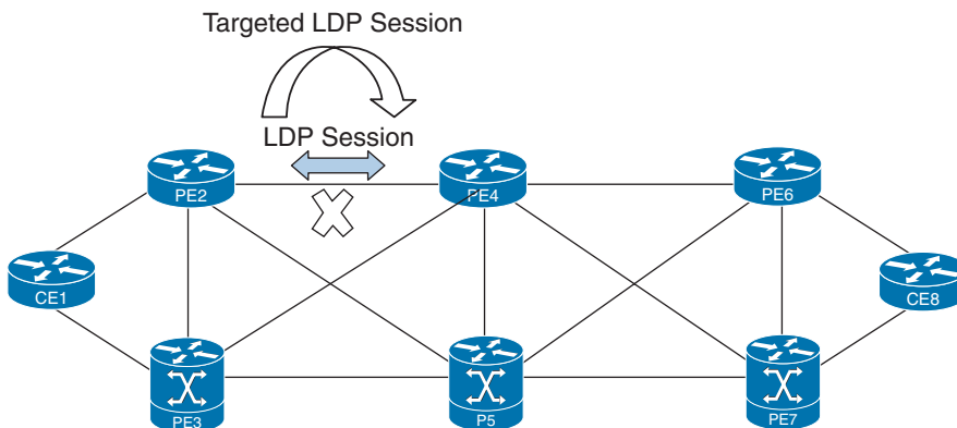
Figure 10-12 MPLS LDP Session Protection
