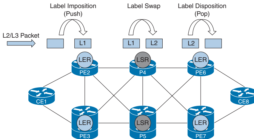
Figure 1-6 MPLS Basics
