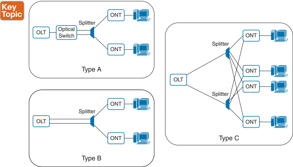
Figure 1-17 Network Protection Modes
