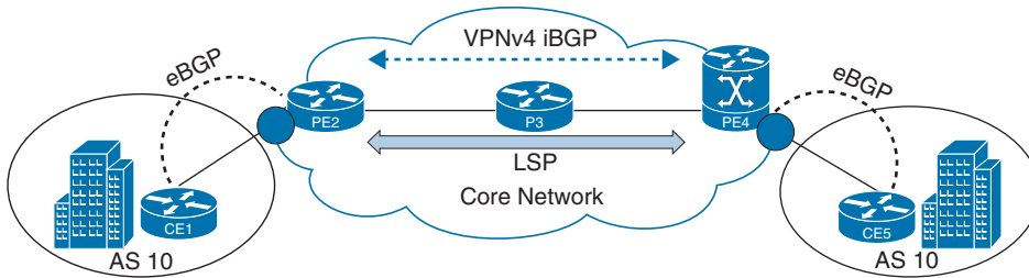
Figure 12-15 MPLS L3VPN, BGP PE-CE
