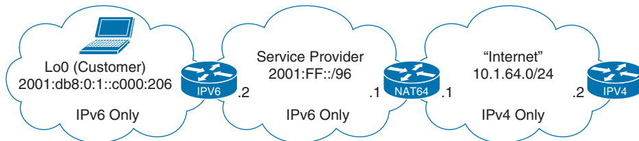
Figure 19-4 NAT64 Stateless
