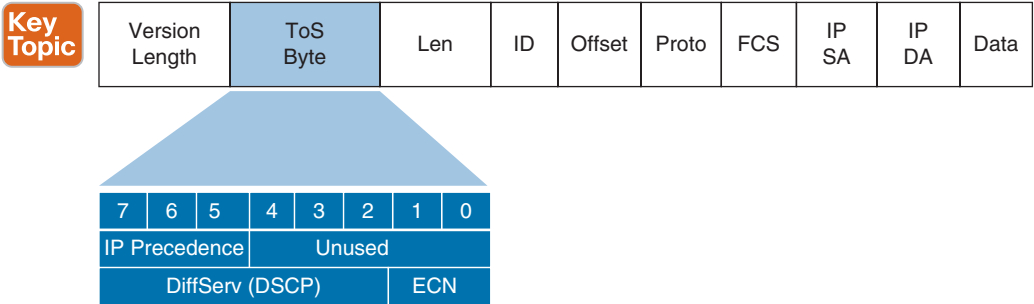
Figure 21-3 IP Precedence and DSCP
