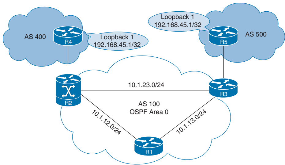
Figure 8-7 BGP Best External
