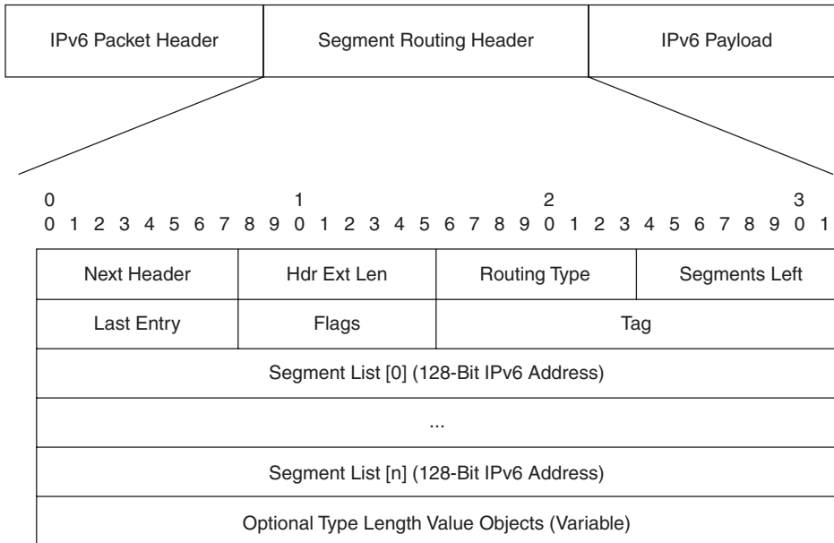
Figure 15-11 IPv6 Segment Routing Header Format
