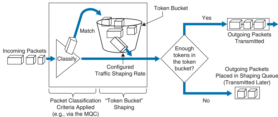
Figure 21-6 Traffic Shaping
