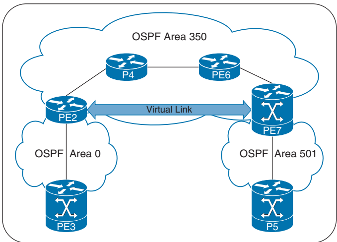
Figure 6-6 OSPF Virtual Link Topology
