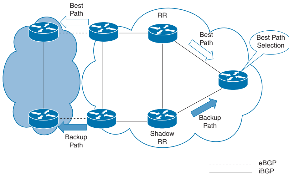
Figure 8-6 BGP Shadow Route Reflector
