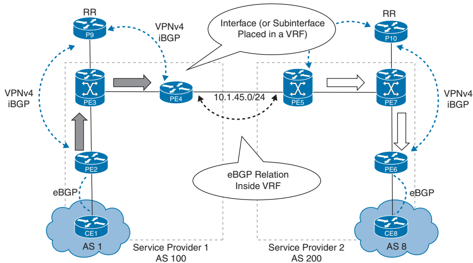
Figure 13-8 MPLS L3VPN Inter-AS Option A
