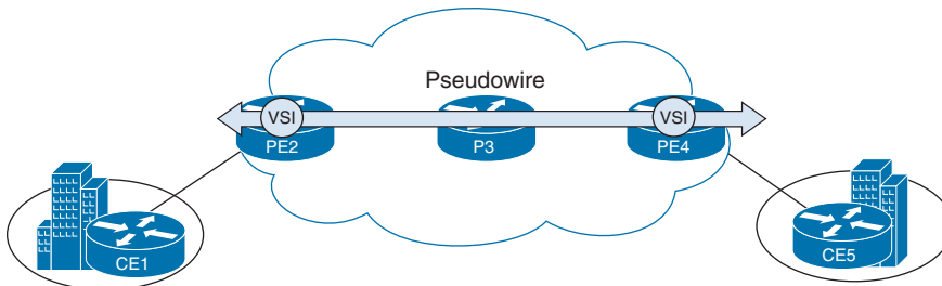
Figure 11-10 VPLS with Manual LDP
