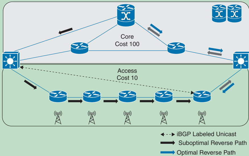
Figure 7-15 BGP AIGP Attribute Use Case
