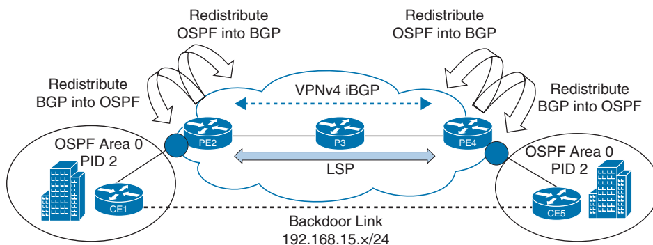
Figure 12-8 OSPF as PE-CE Routing Protocol
