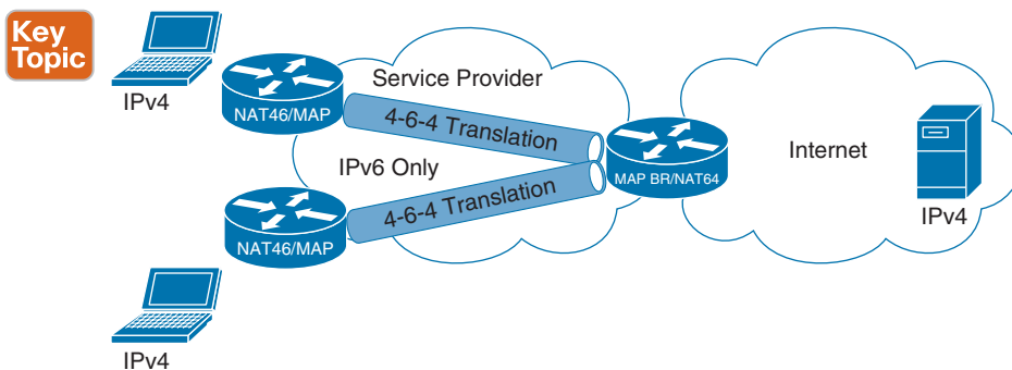
Figure 19-8 MAP-T
