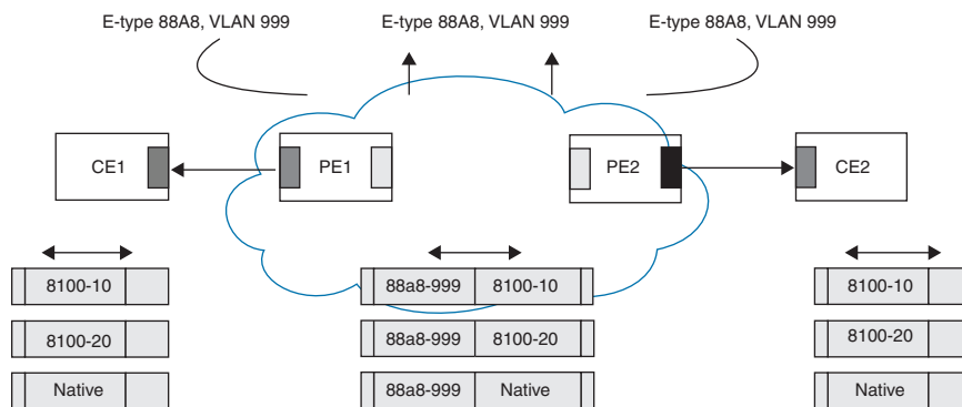
Figure 11-22 Layer 2 PDU Tunneling
