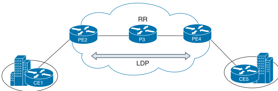
Figure 11-28 EVPN Example
