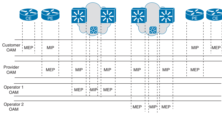
Figure 11-18 Maintenance Association
