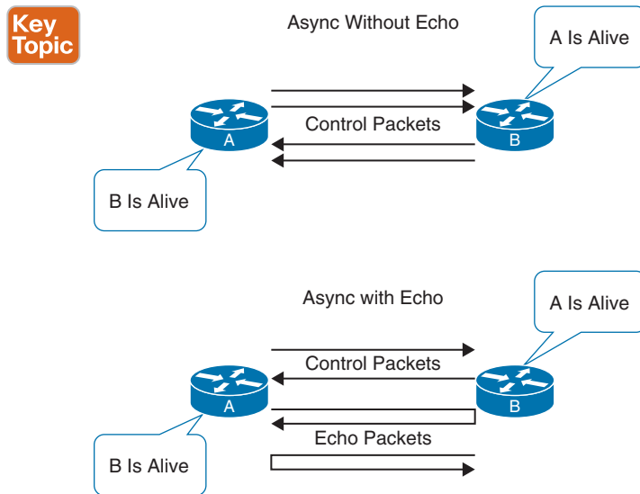
Figure 20-1 BFD Modes on IOS XR
