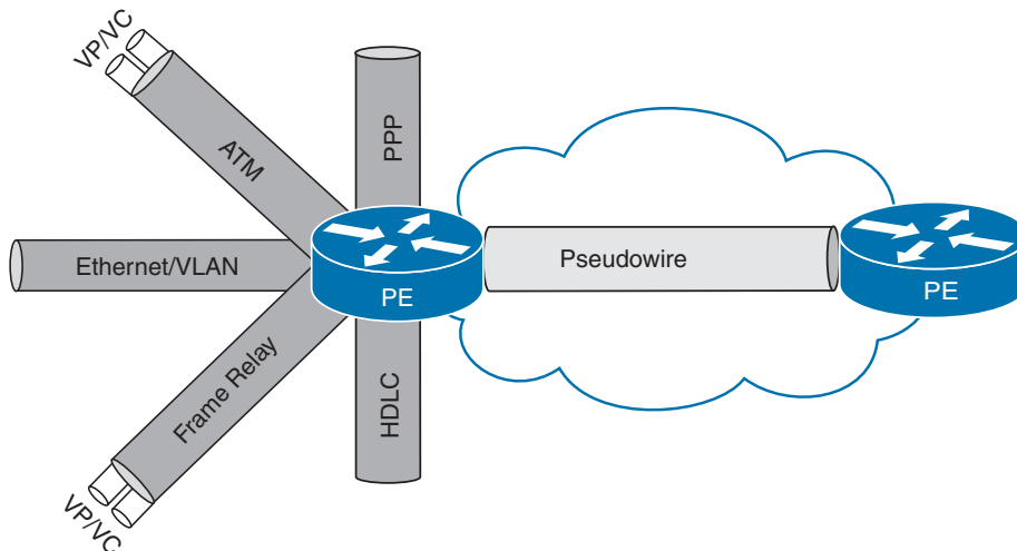
Figure 11-5 AToM
