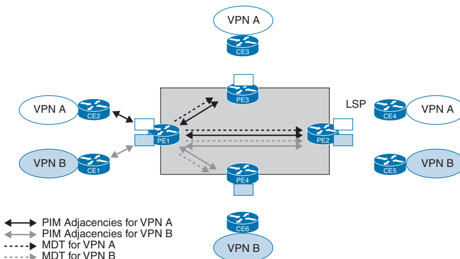
Figure 12-20 PIM/GRE mVPN: Routing Information Distribution
