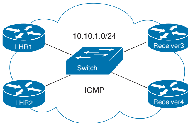
Figure 9-2 IGMP Reference Diagram
