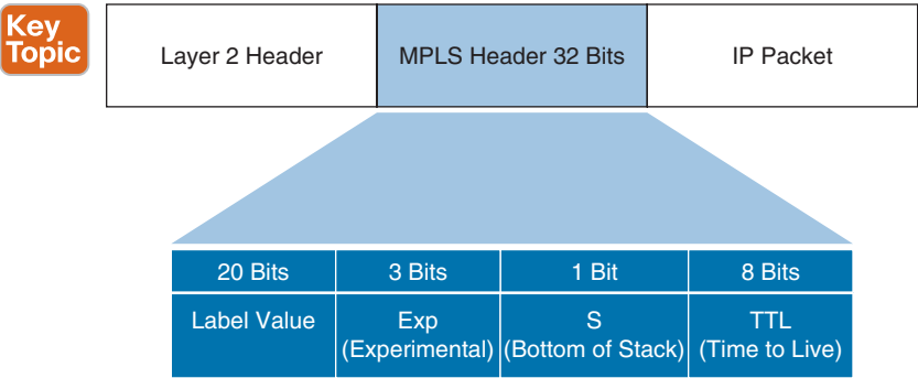
Figure 21-4 MPLS EXP Field
