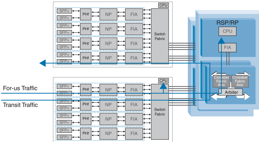
Figure 16-2 LPTS Architecture
