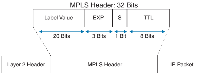
Figure 1-5 IP Packet Header Structure with MPLS Encapsulation
