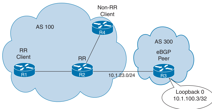
Figure 7-24 BGP Route Reflection Rule #3
