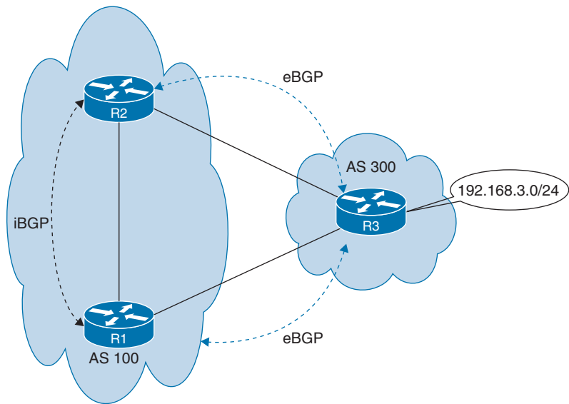
Figure 7-10 BGP AS-PATH Prepending
