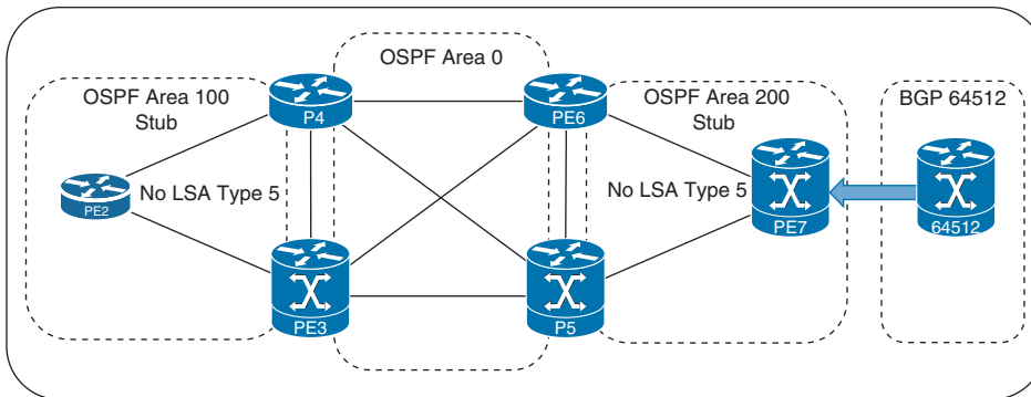
Figure 6-4 How Would You Import BGP Routes into Stub?
