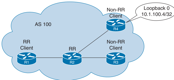
Figure 7-21 Topology for BGP Route Reflection Rule #1
