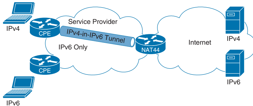
Figure 19-6 DS-Lite
