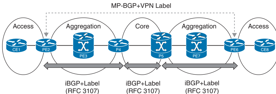
Figure 1-8 RFC 3107 Prescribed Architecture
