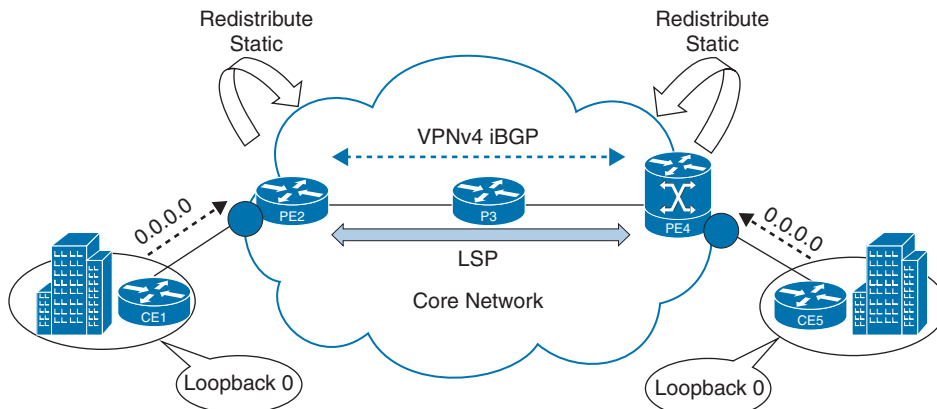
Figure 12-6 MPLS L3VPN Static PE-CE, Redistribution Process
