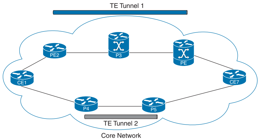
Figure 14-7 MPLS Traffic Engineering Forwarding Adjacency
