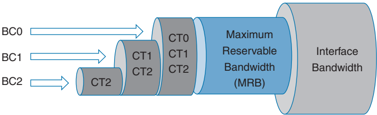
Figure 14-19 Russian Dolls Model
