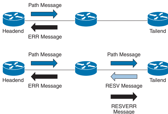
Figure 14-4 RSVP Error Message
