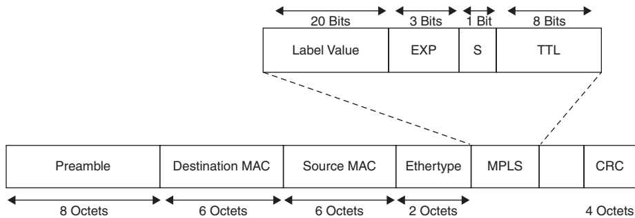
Figure 10-1 MPLS Header
