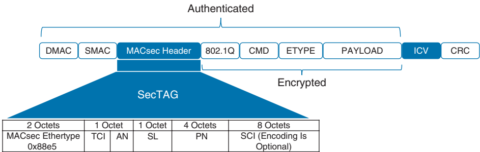
Figure 18-5 MACsec Tags Added to Ethernet Frames
