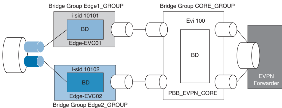
Figure 11-23 Provider Edge Router
