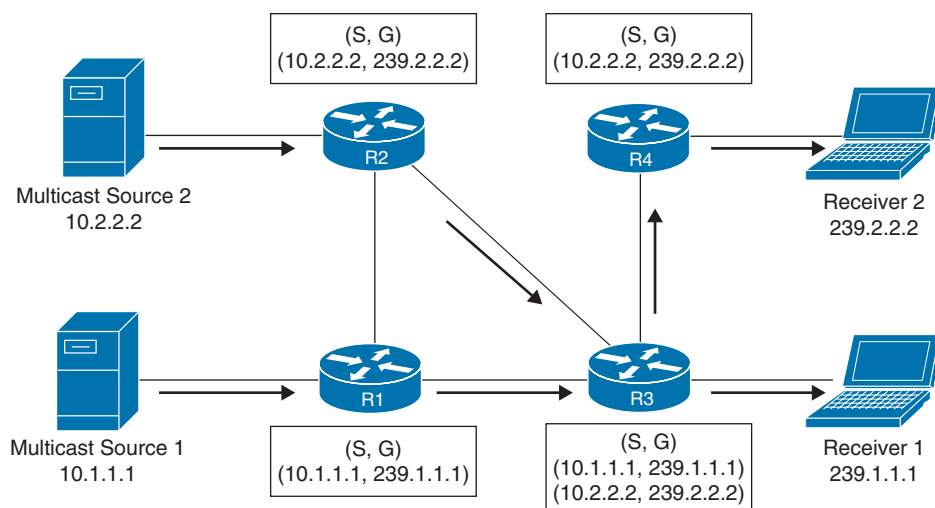
Figure 9-5 Example of a Multicast Source-Based Tree with Multiple Sources and Receivers
