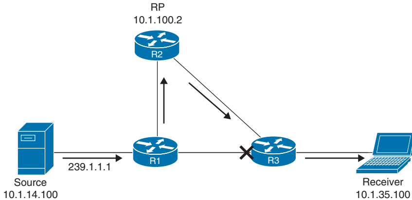
Figure 9-7 Building a Shared RP-Based Multicast Tree
