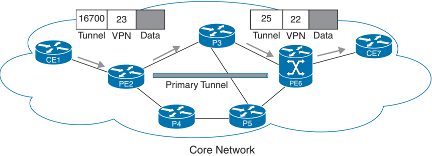
Figure 14-15 MPLS TE FRR Labels
