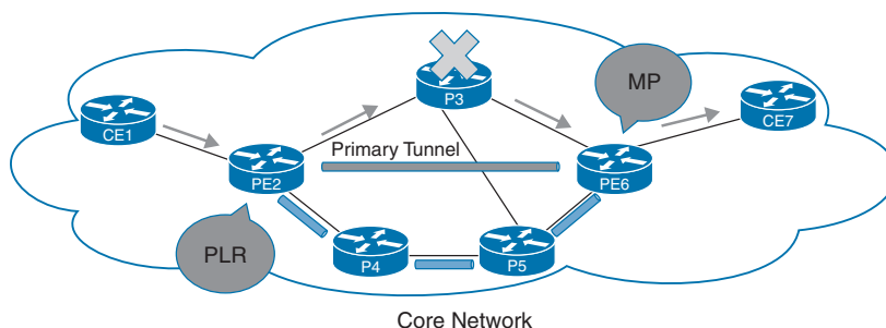
Figure 14-12 MPLS TE FRR: Node Protection
