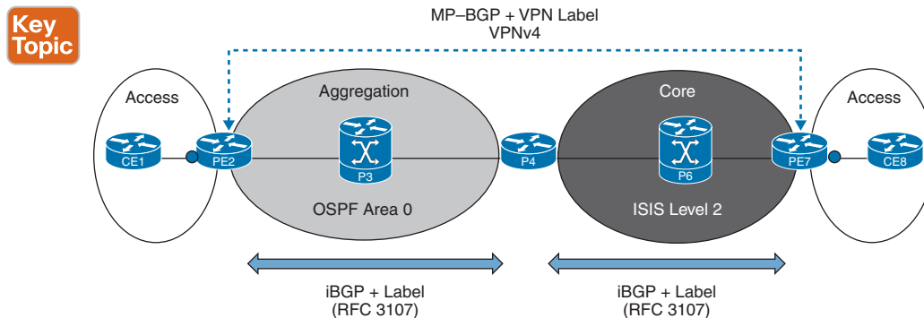
Figure 13-1 Unified MPLS Structure
