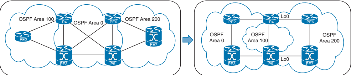
Figure 6-5 Multi-Area Adjacency Topology
