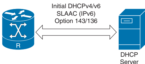
Figure 22-10 Secure ZTP DHCP Server Communications
