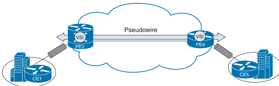
Figure 11-11 VPLS with Manual LDP, IOS XR
