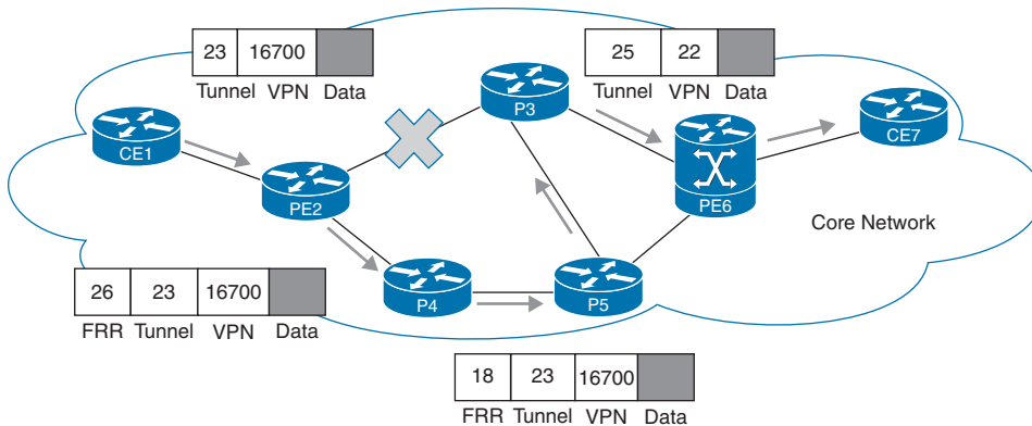
Figure 14-16 MPLS TE FRR, Label Stacking
