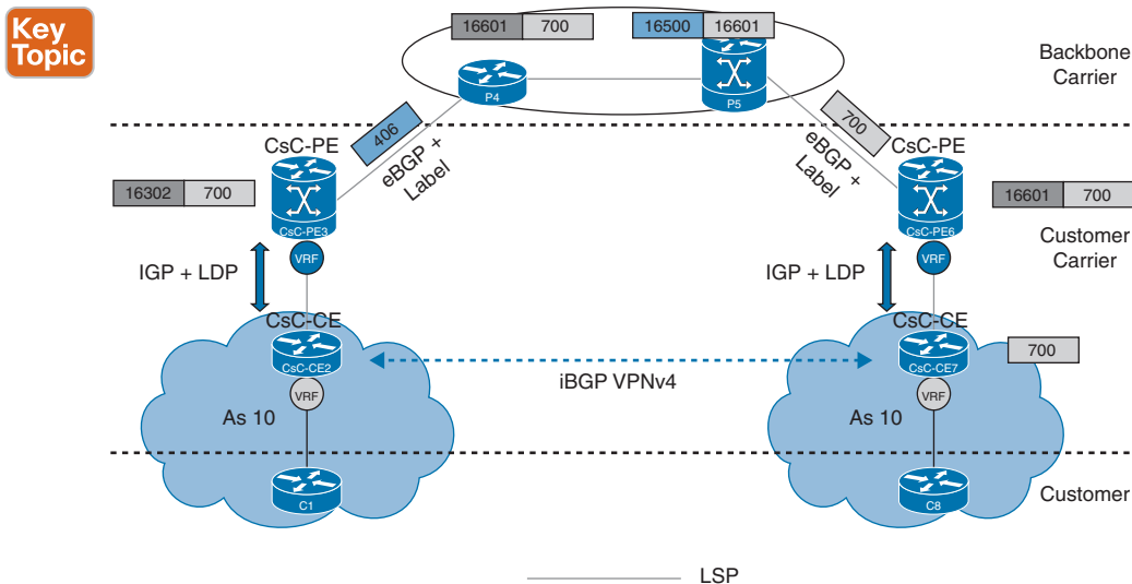
Figure 13-14 MPLS Carrier Supporting Carrier (CsC)
