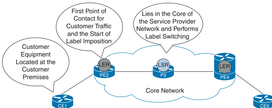
Figure 12-1 MPLS Main Devices
