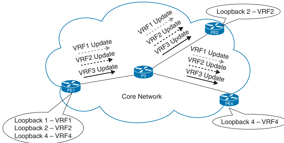
Figure 12-18 Route Target Constraint
