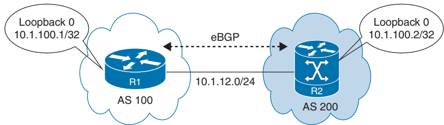
Figure 7-8 BGP Prefix Advertisement Process
