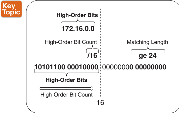
Figure 4-1 Prefix Matching
