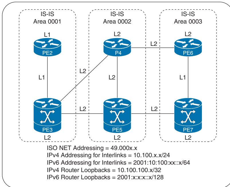
Figure 5-1 Base IS-IS Topology
