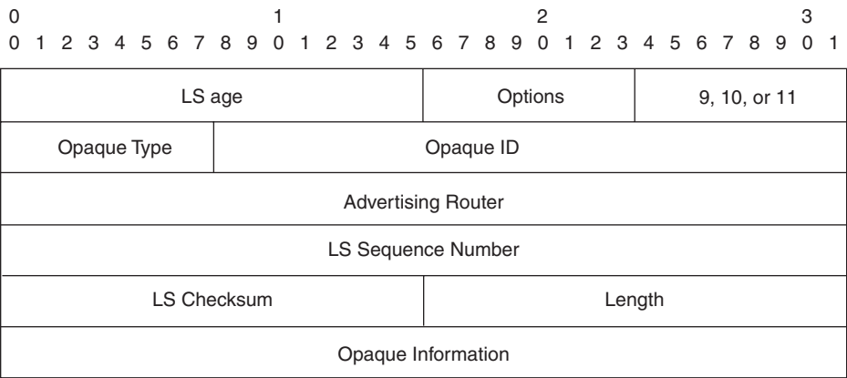
Figure 15-8 Opaque LSA Format
