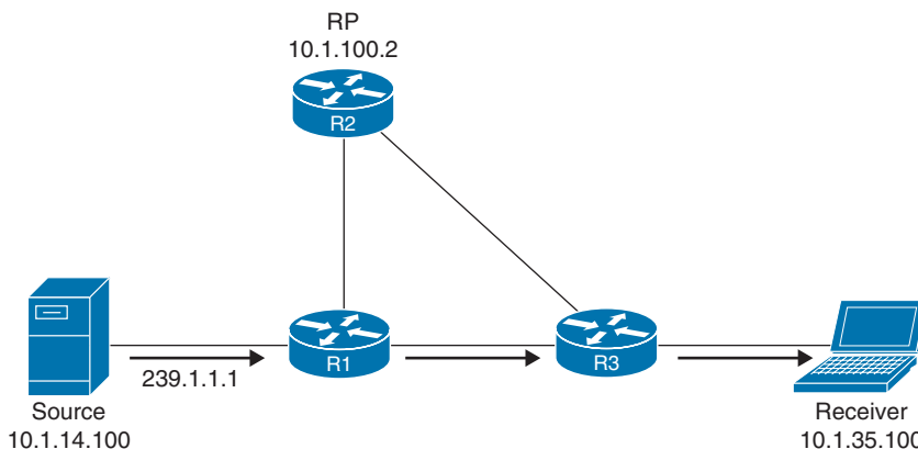
Figure 9-8 PIM SPT Switchover
