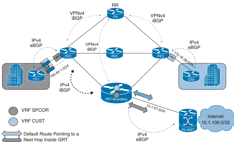
Figure 13-5 MPLS L3VPN Internet Access Option 2
