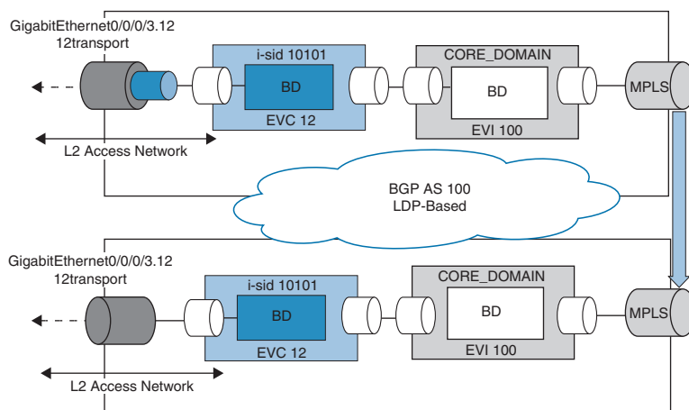
Figure 11-24 Provider Backbone Bridging Example
