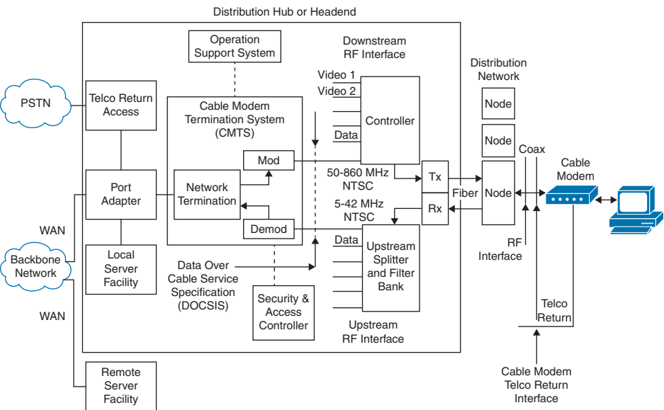
Figure 1-10 DOCSIS Architecture
