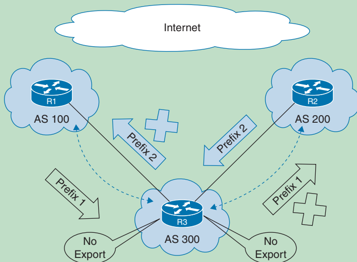
Figure 7-19 BGP Transit AS, no-export community
