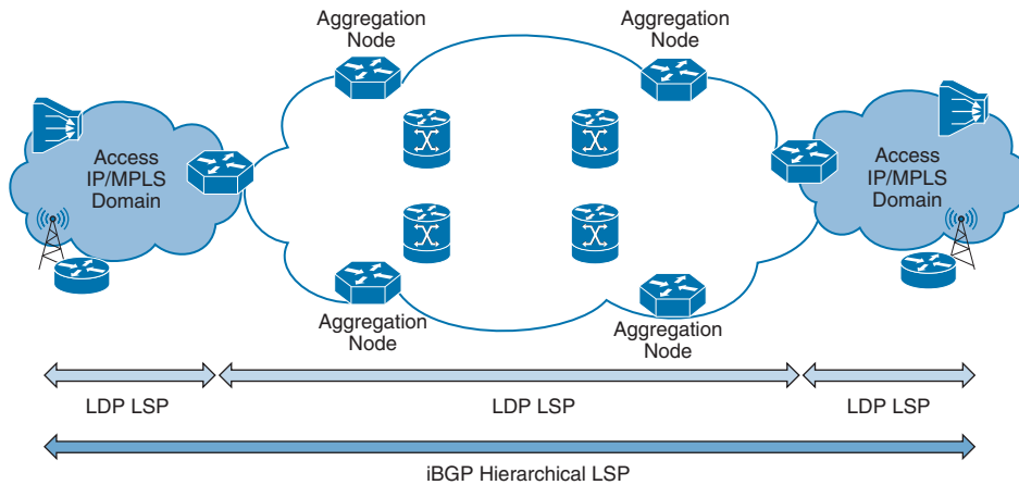
Figure 13-3 Unified MPLS Use Case
