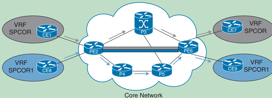
Figure 14-8 Per-VRF MPLS TE Tunnels
