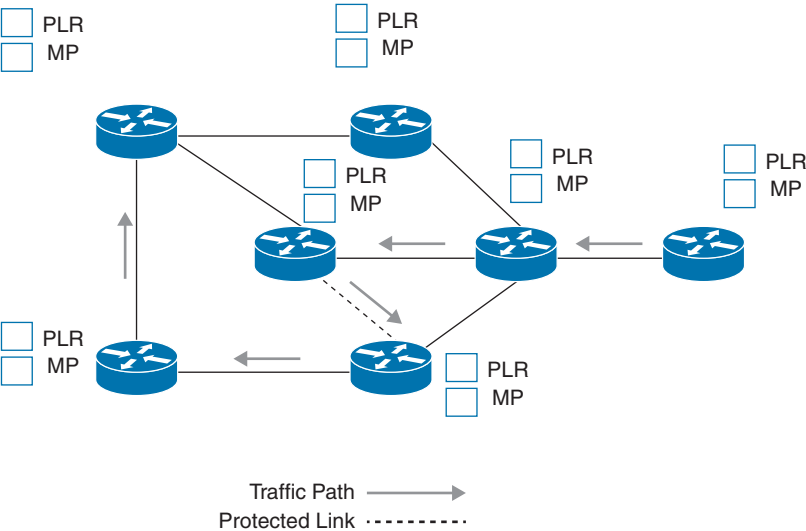
Figure 14-17a Brainstorm: MPLS TE FRR Roles, Solution
