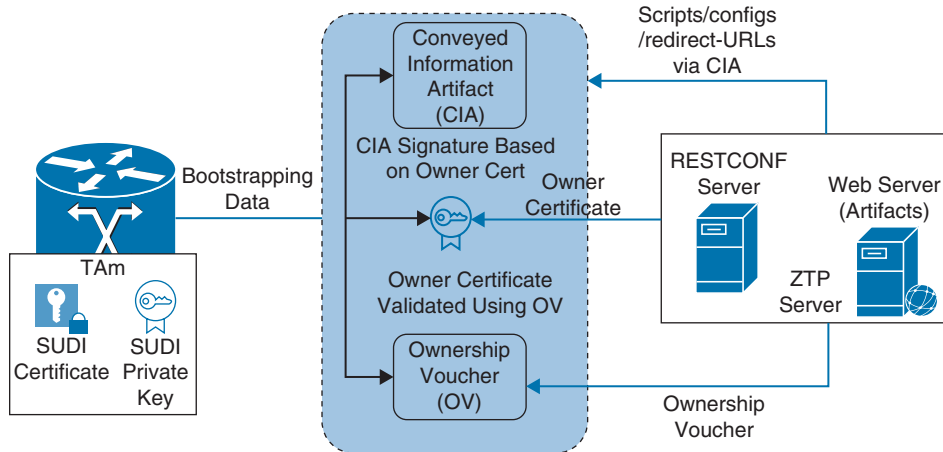
Figure 22-12 Secure ZTP Server Validation
