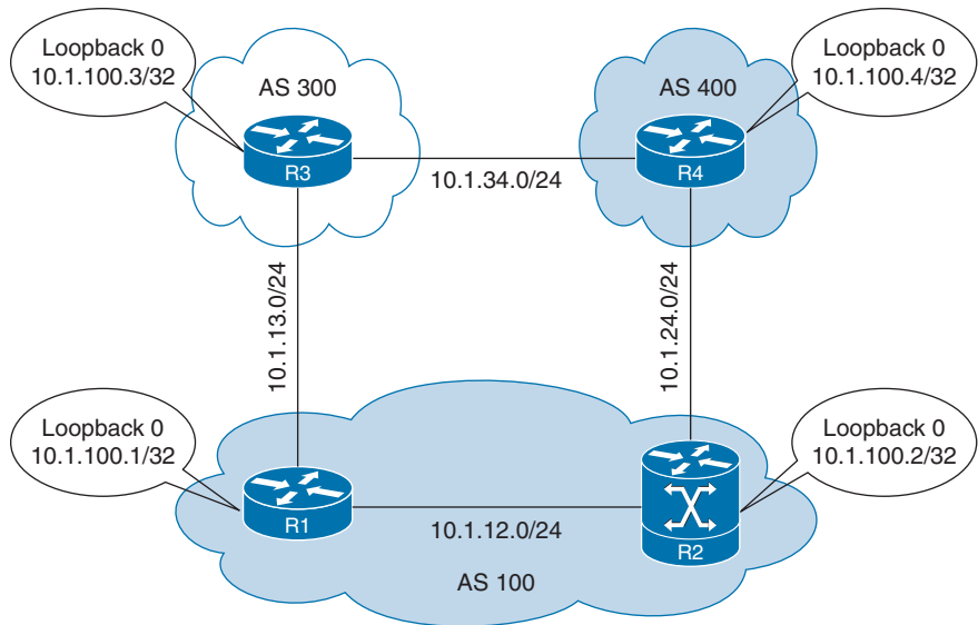
Figure 7-9 BGP Path Attributes Demonstration Example
