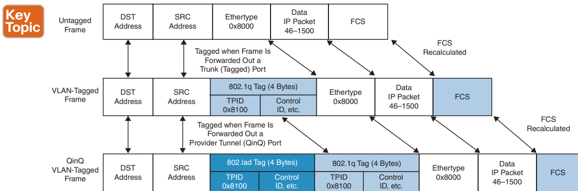
Figure 11-21 Ethertypes and Frame Tagging
