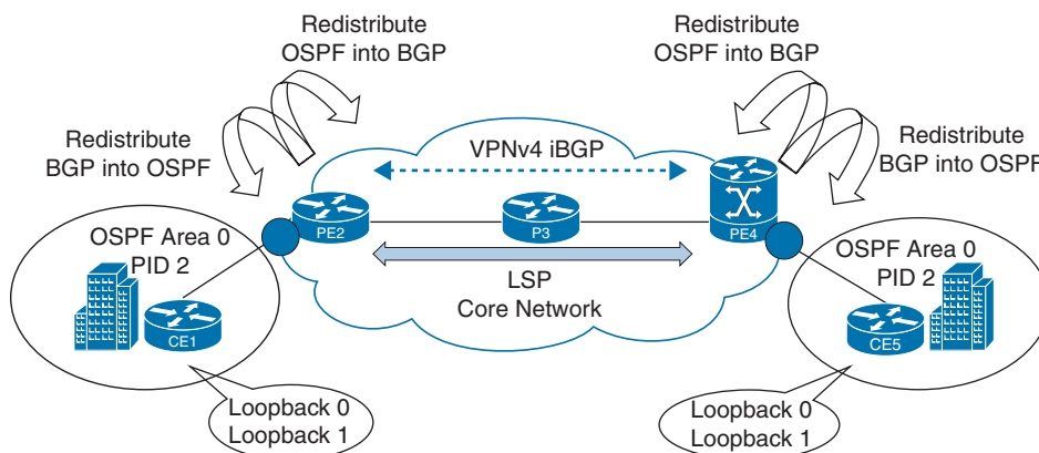
Figure 12-17 Route Target Filtering
