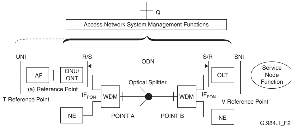
Figure 1-15 GPON Reference Diagram
