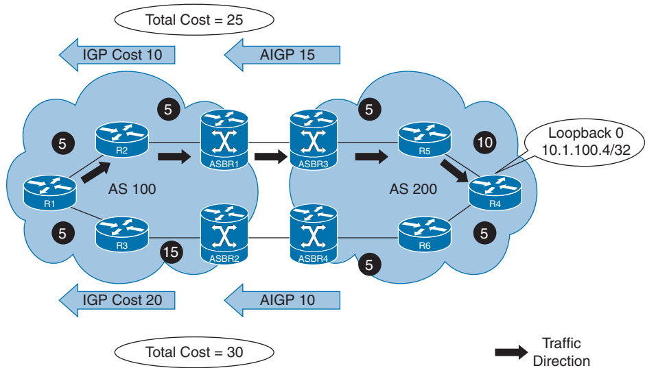
Figure 7-14 BGP AIGP Demonstration Example #2
