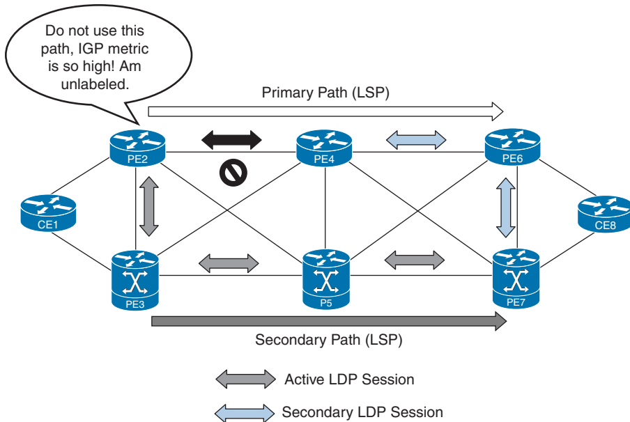
Figure 10-14 MPLS LDP IGP Synchronization Traffic Redirection
