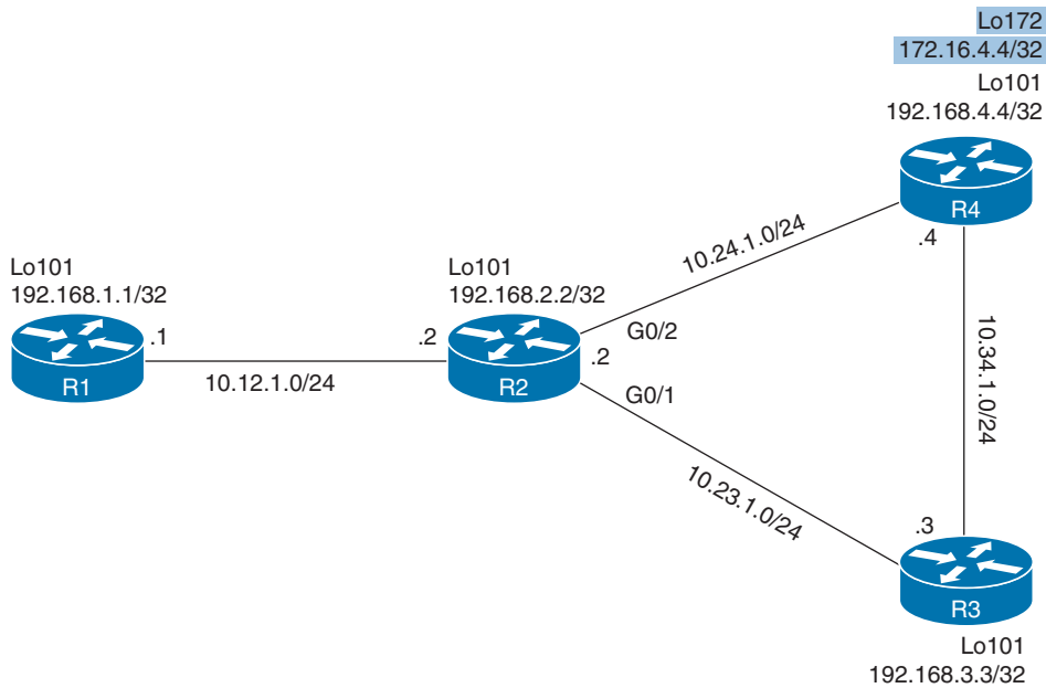
Figure 18-3 uRPF Strict Mode: Modified Setup
