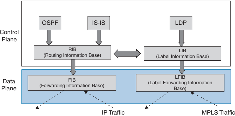
Figure 10-7 Data Plane and Control Plane
