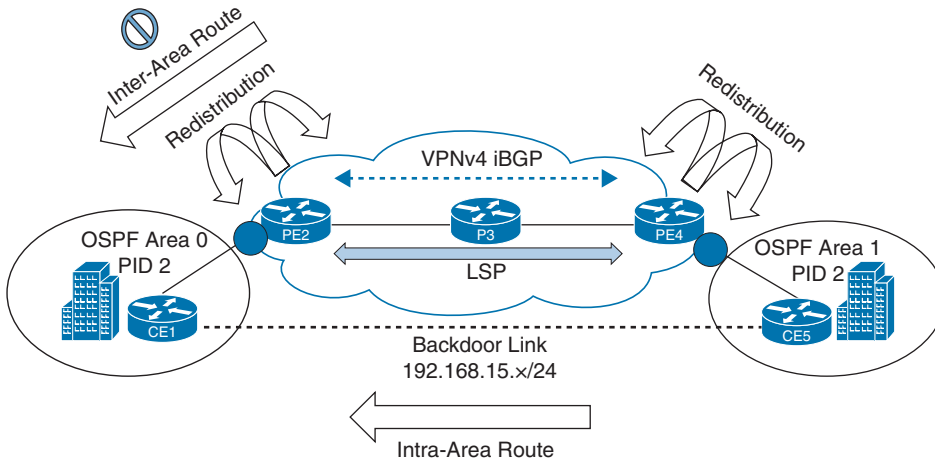
Figure 12-11 OSPF Backdoor Link Intra-Area Routes
