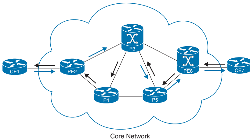
Figure 14-5 MPLS Traffic Engineering Example
