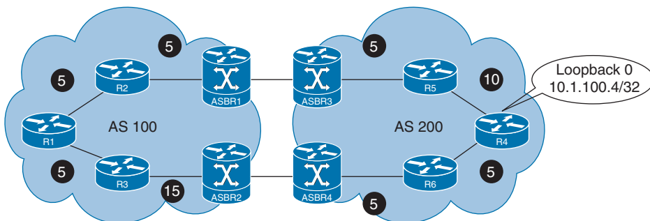
Figure 7-12 BGP AIGP Demonstration Example #1
