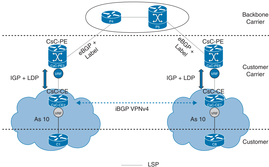
Figure 13-15 MPLS CsC Label Operation
