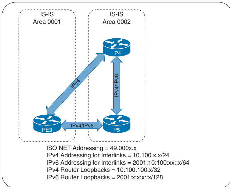
Figure 5-2 Single-Topology Dual-Stack Network
