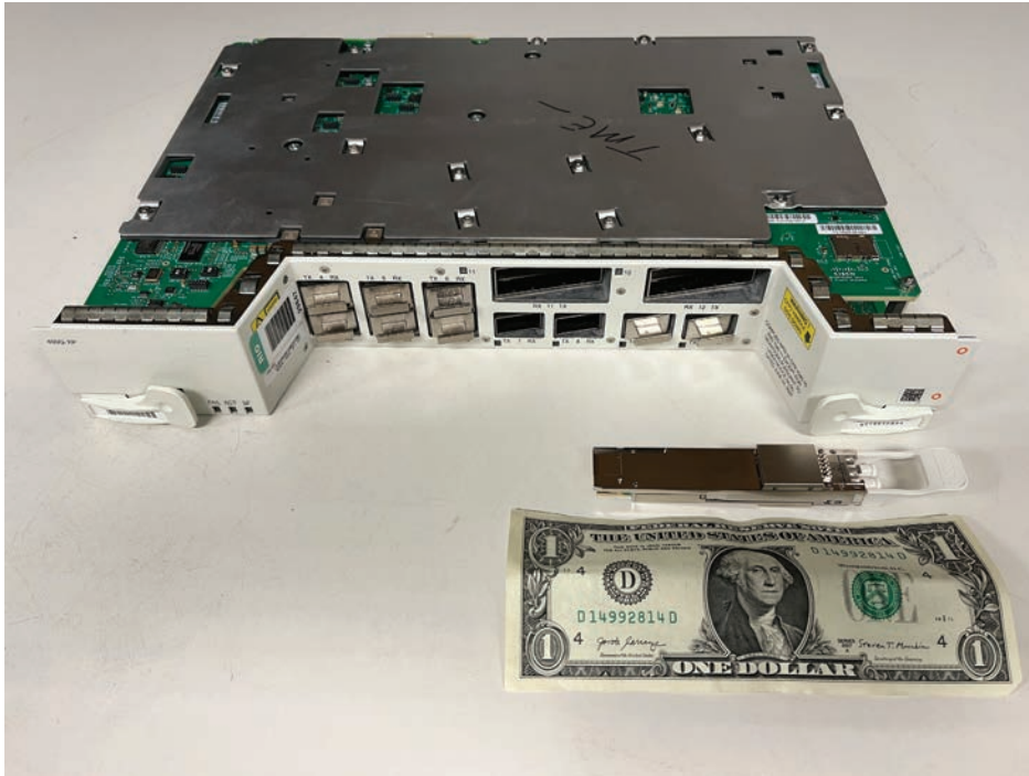
Figure 1-20 Intelligent DWDM Pluggables Used in Routers
