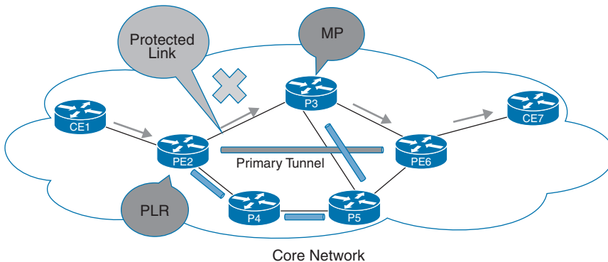
Figure 14-14 MPLS TE FRR: Link Protection, IOS XR
