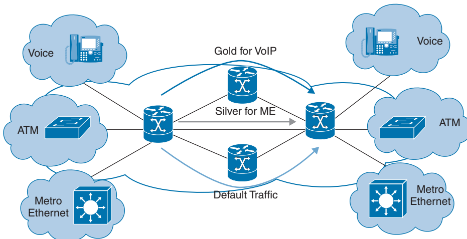
Figure 14-22 Policy-Based Tunnel Selection Deployment Examples
