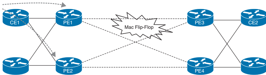
Figure 11-27 VPLS Limitation: MAC Flip-Flopping
