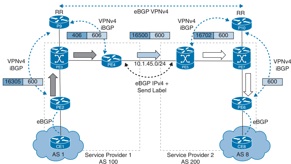
Figure 13-11 Inter-AS Option C VPN Label Assignment
