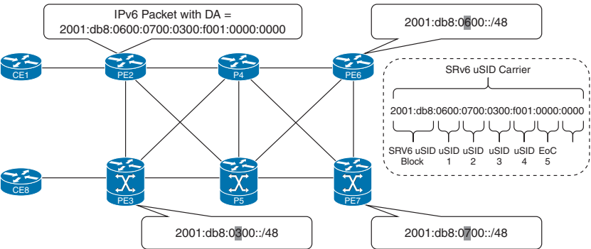
Figure 15-13 uSID in Action
