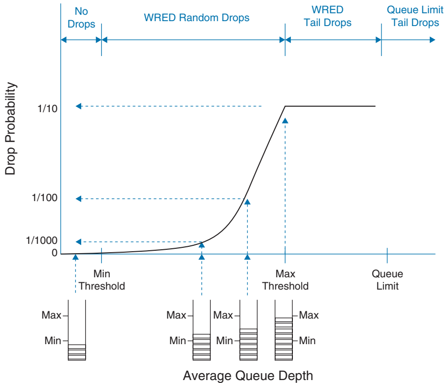
Figure 21-8 WRED Drop Probabilities
