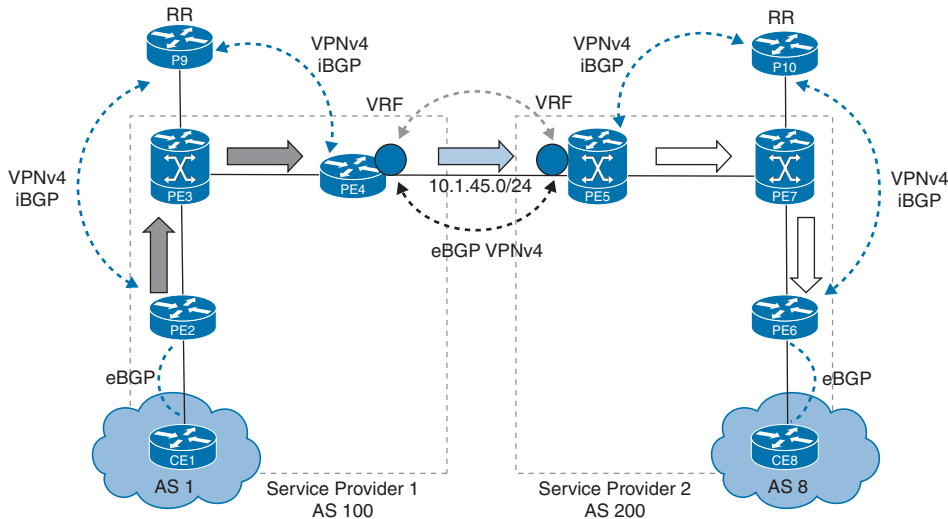
Figure 13-12 MPLS L3VPN Inter-AS Option D (AB)
