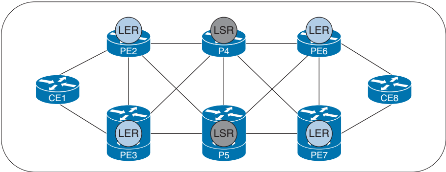
Figure 10-3 MPLS Main Components
