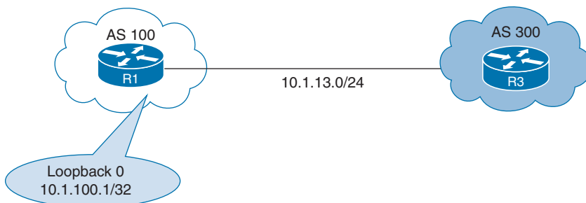
Figure 8-3 BGP Dampening Example
