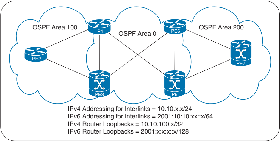
Figure 6-2 OSPF Topology
