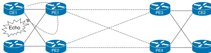
Figure 11-25 VPLS Limitation: Per-flow Redundancy
