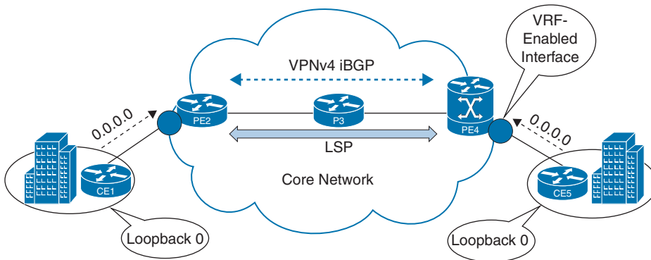
Figure 12-5 MPLS L3VPN Static PE-CE
