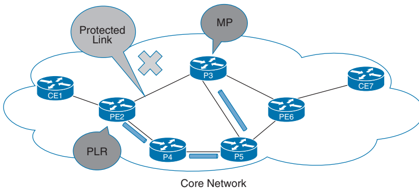
Figure 14-11 MPLS TE FRR: Link Protection
