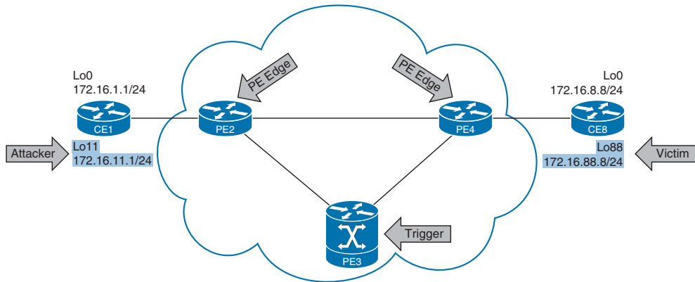
Figure 18-4 RTBH Reference Diagram
