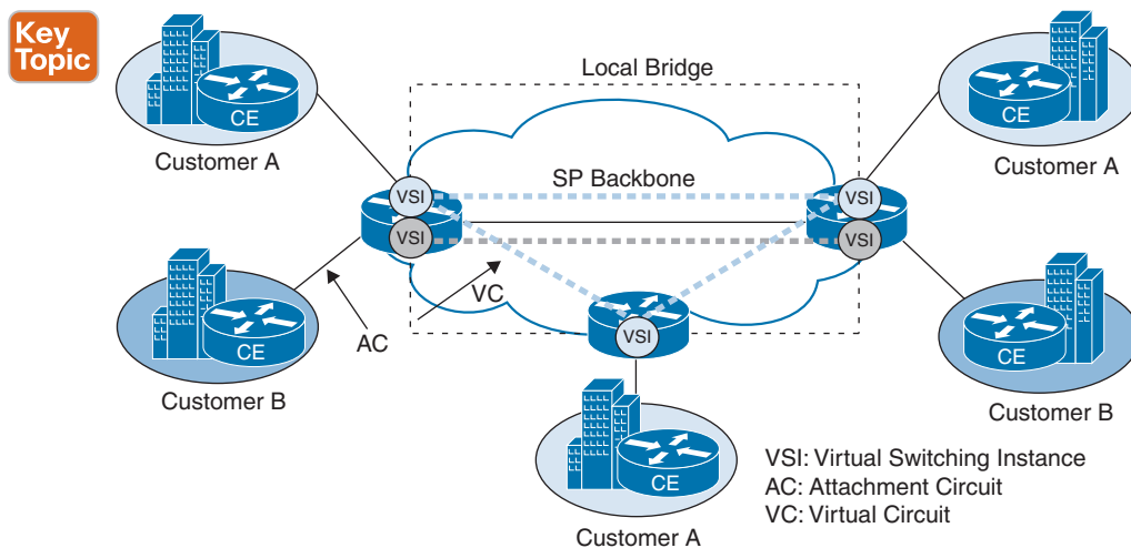
Figure 11-8 VPLS Architecture
