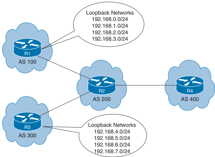
Figure 7-16 BGP Aggregate Address Configuration Example
