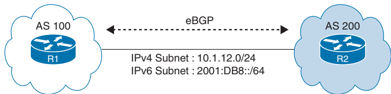
Figure 7-4 BGP Messages Exchange, IPv4 and IPv6 Address Families
