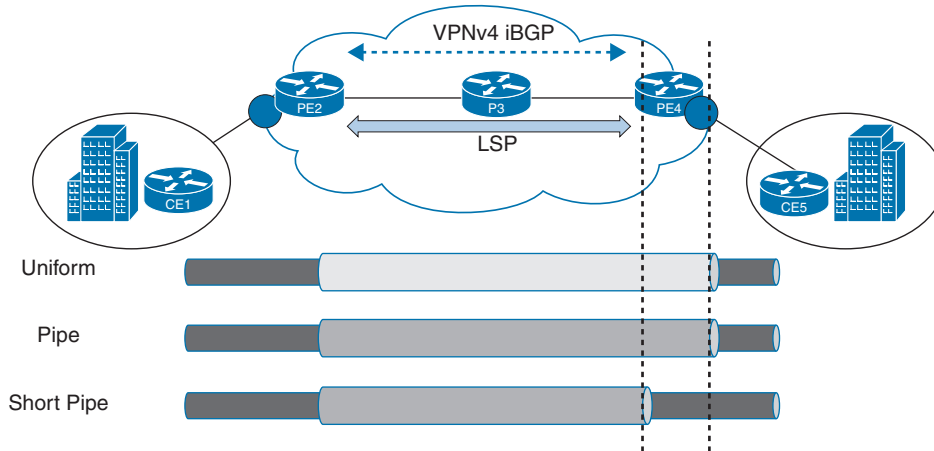
Figure 13-16 MPLS QoS Models
