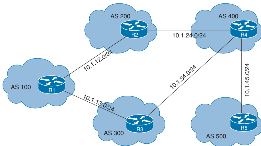
Figure 8-5 BGP Additional Paths on eBGP Topology
