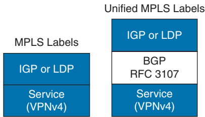
Figure 1-9 Additional Unified MPLS BGP Label
