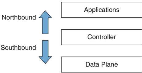
Figure 22-1 Basic SDN Architecture and API Interaction
