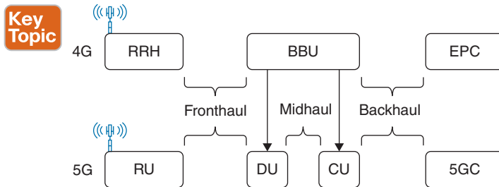
Figure 1-23 xHaul Segments
