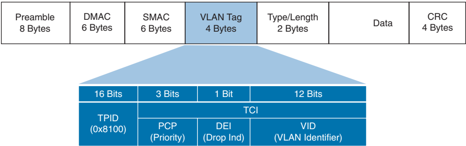
Figure 21-2 802.1Q VLAN Tag Fields
