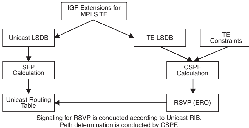
Figure 14-2 RSVP Operation in MPLS TE
