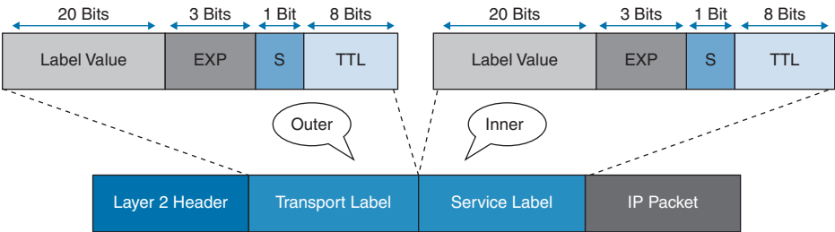
Figure 12-4 MPLS Labels
