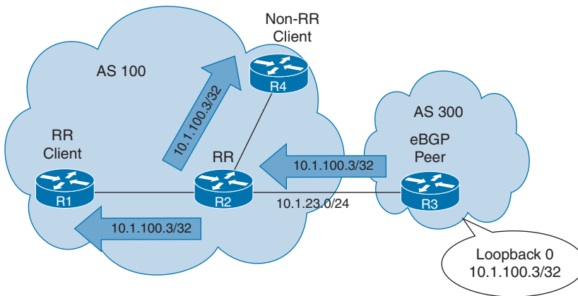
Figure 7-25 BGP Route Reflection Rule #3
