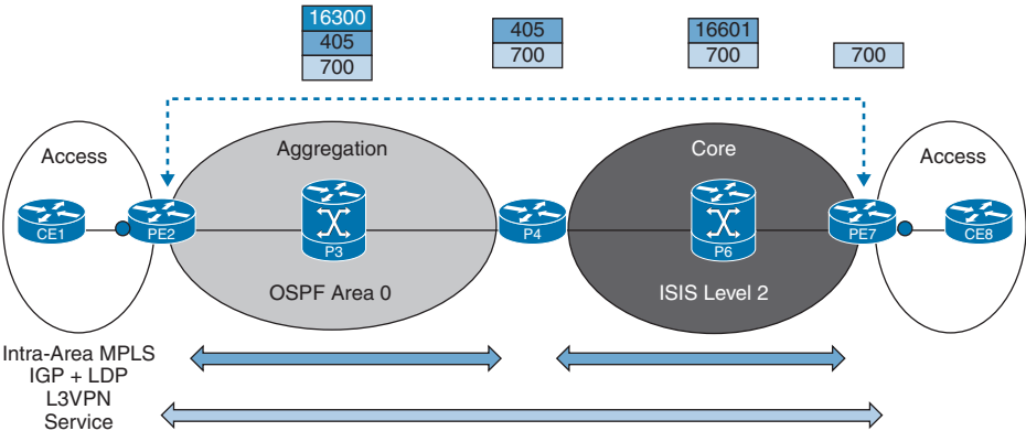
Figure 13-2 Unified MPLS Label Operation
