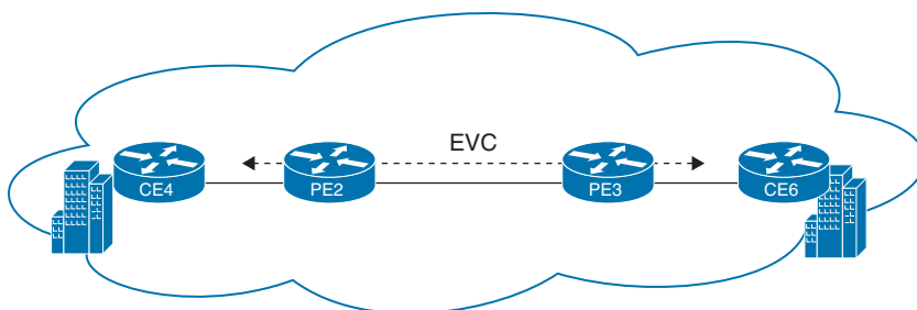
Figure 11-20 CFM over VPWS Connection
