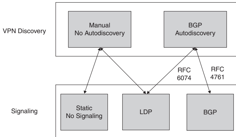
Figure 11-9 VPLS Discovery and Signaling
