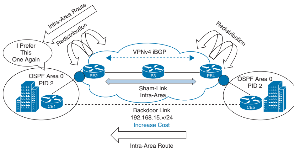
Figure 12-12 OSPF Backdoor
