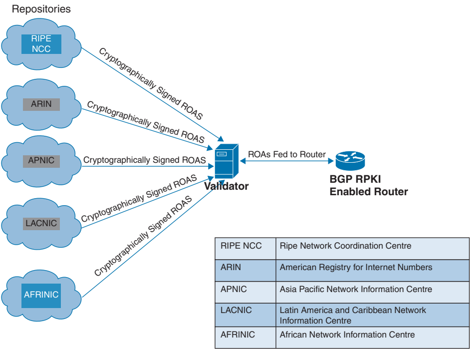
Figure 16-6 RPKI Architecture
