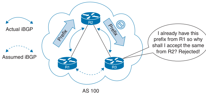
Figure 7-20 BGP Route Reflection
