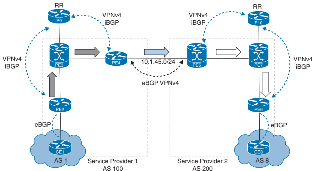
Figure 13-9 MPLS L3VPN Inter-AS Option B
