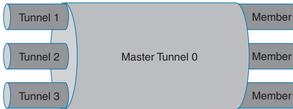
Figure 14-20 CBTS Master Tunnel and Tunnel Members
