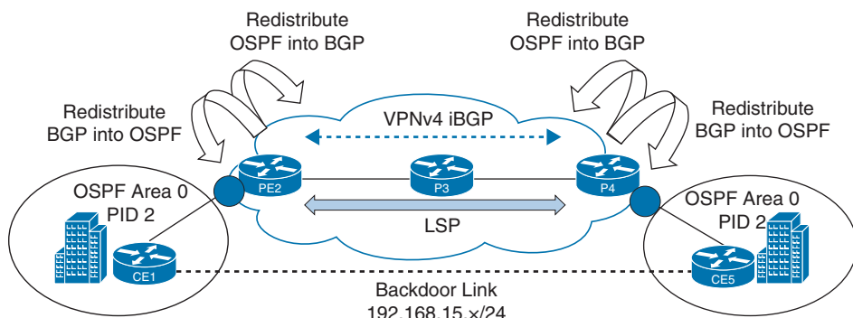
Figure 12-10 MPLS PE-CE OSPF, Backdoor Link
