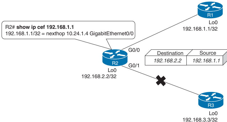
Figure 18-2 uRPF Strict Mode
