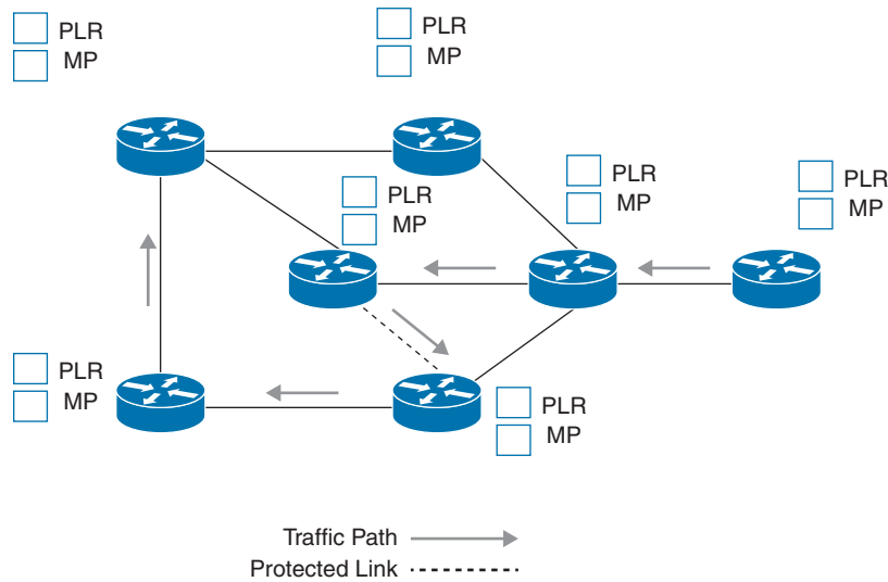
Figure 14-17 Brainstorm: MPLS TE FRR Roles
