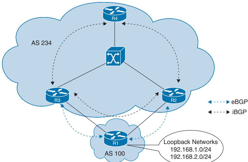
Figure 7-18 BGP Cost Community Demonstration Example
