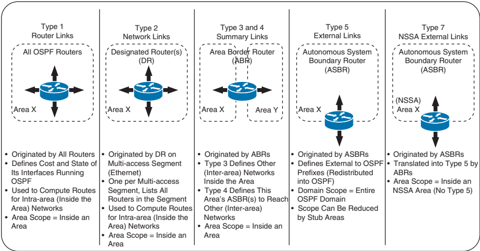
Figure 6-1 OSPF LSA Types
