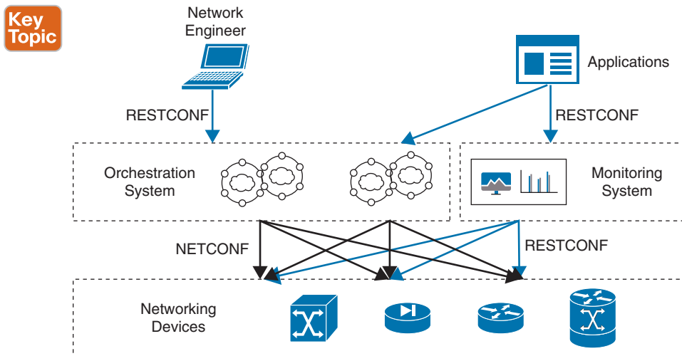
Figure 22-4 Model-Driven Programmability Architecture
