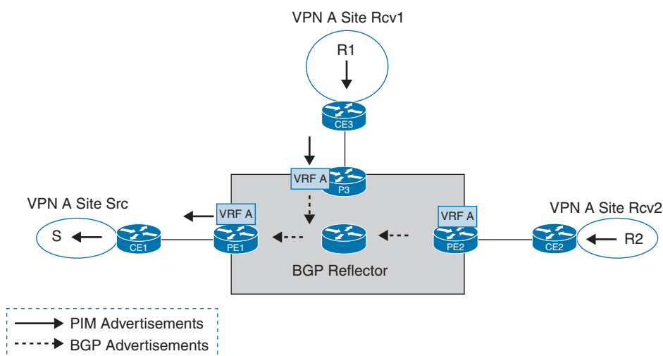
Figure 12-21 BGP/MPLS mVPN
