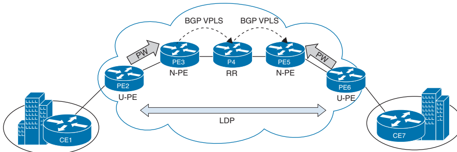
Figure 11-13 H-VPLS
