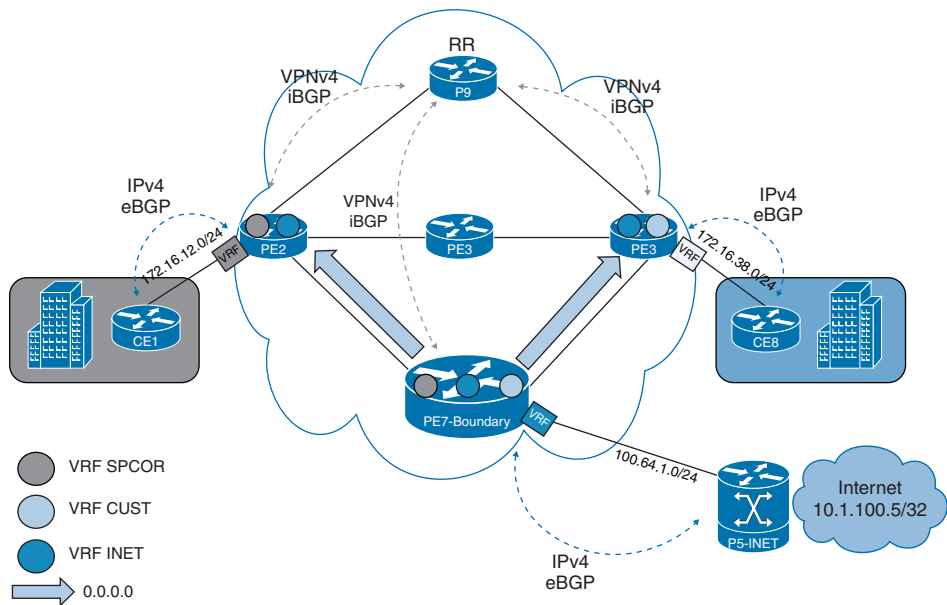
Figure 13-7 MPLS L3VPN Internet Access Option 4
