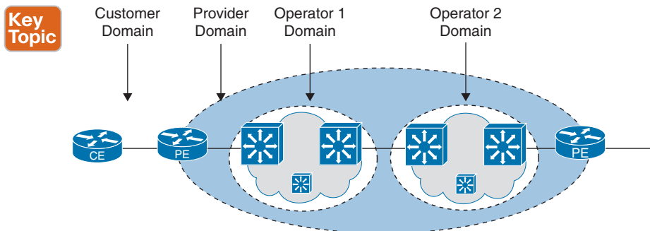
Figure 11-19 CFM Terminology
