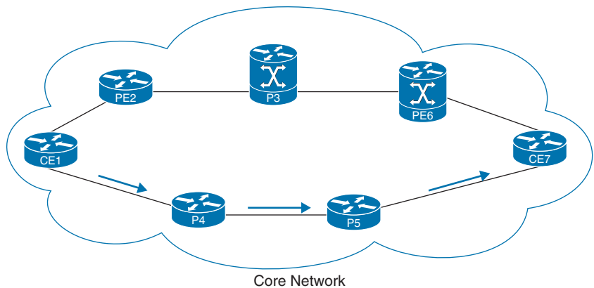
Figure 14-6 MPLS TE Forwarding Adjacency
