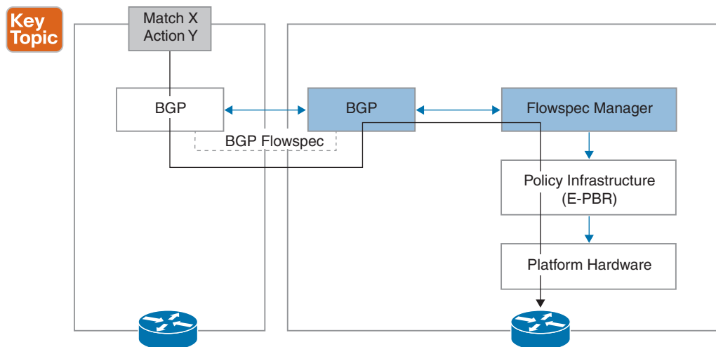
Figure 16-8 Flowspec Logical Flow Diagram
