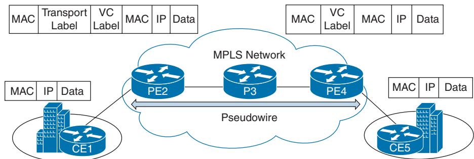
Figure 11-6 AToM Example
