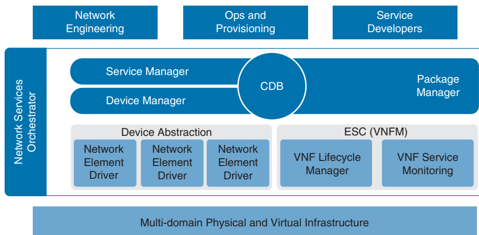
Figure 22-9 NSO Architecture
