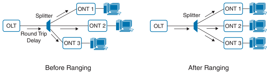
Figure 1-16 PON Ranging
