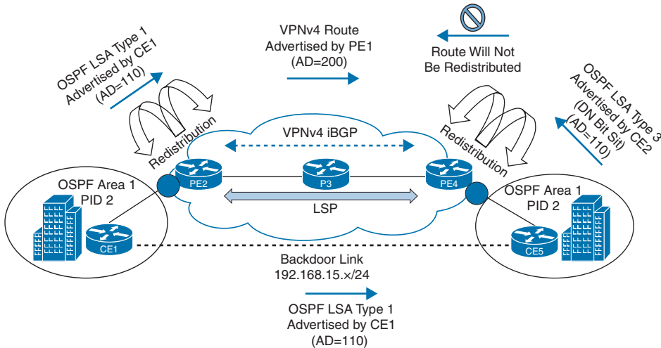
Figure 12-13 OSPF MPLS L3VPN, Down Bit
