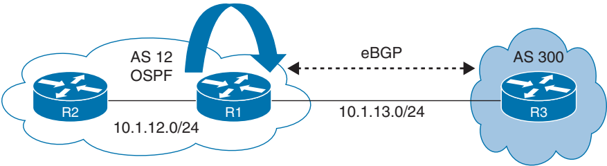
Figure 7-17 BGP Redistribution Example
