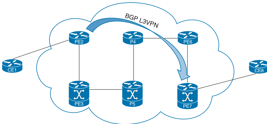
Figure 16-3 Service and Transport Labels on a Service Provider Network
