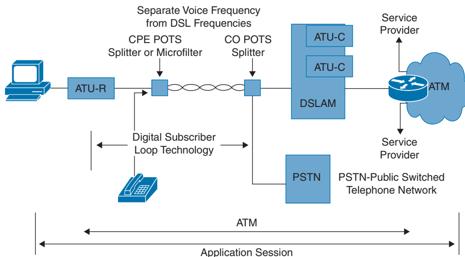
Figure 1-11 Basic DSL Architecture
