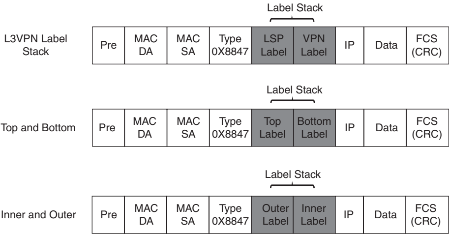
Figure 10-4 MPLS Label Types
