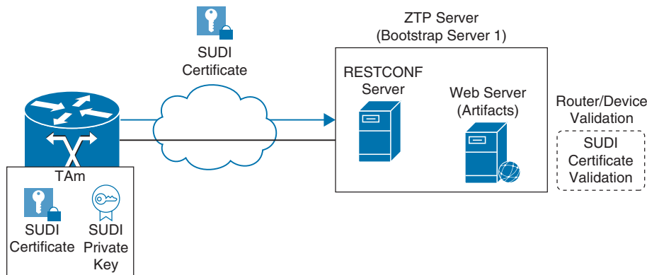
Figure 22-11 Secure ZTP Router Validation
