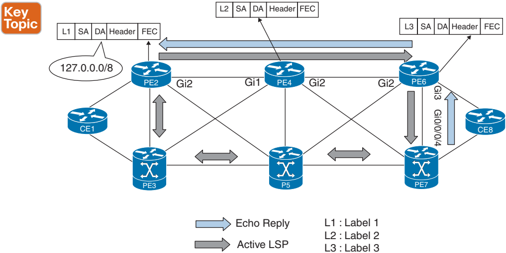
Figure 10-15 MPLS OAM Operation
