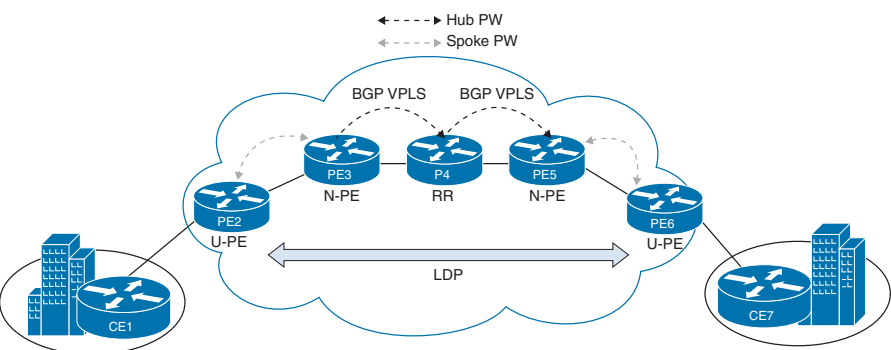
Figure 11-14 H-VPLS Architecture
