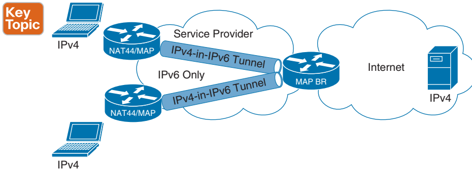
Figure 19-7 MAP-E
