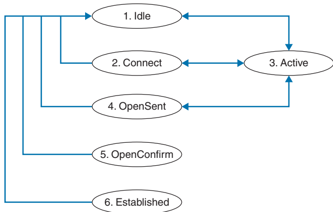
Figure 7-3 BGP Neighbor States
