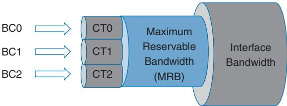
Figure 14-18 Maximum Allocation Model
