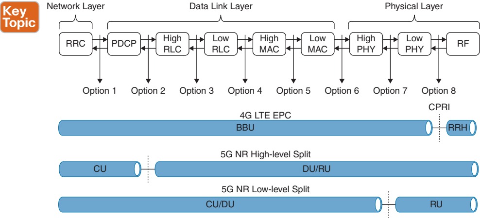
Figure 1-24 Functional Split Options
