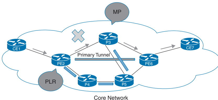
Figure 14-10 MPLS TE FRR Demonstration Example
