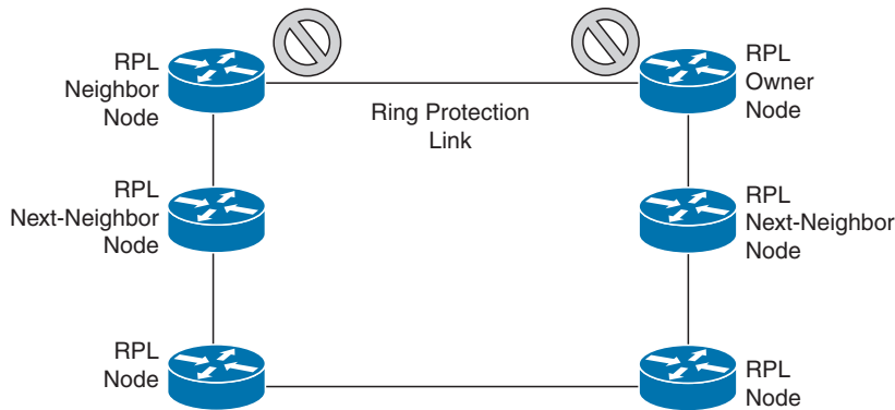
Figure 11-15 G.8032 Ethernet Ring
