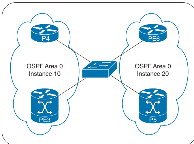
Figure 6-7 OSPF Virtual Link Topology
