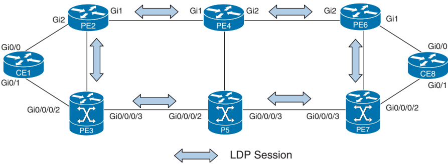
Figure 10-8 MPLS Domain
