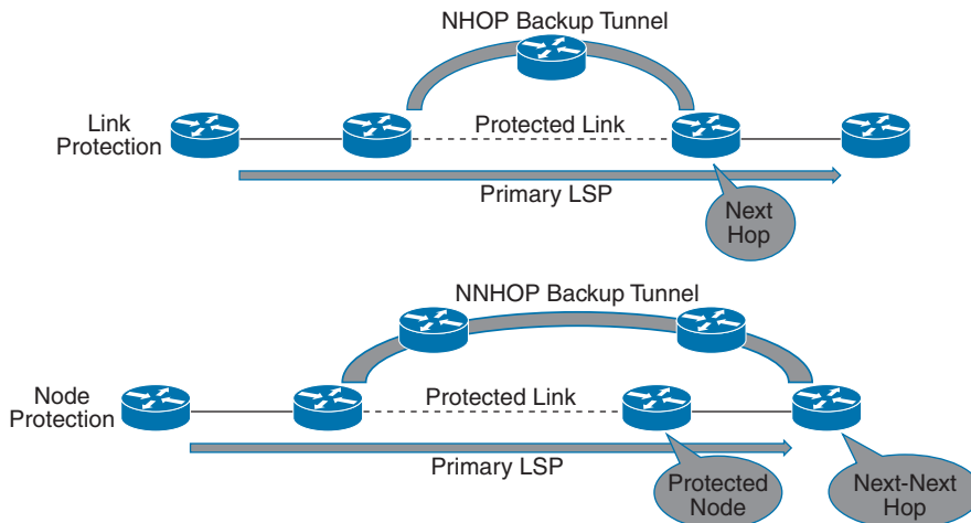
Figure 14-9 MPLS TE FRR: Link and Node Protection
