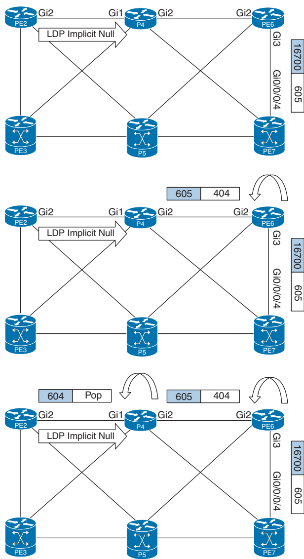
Figure 10-10 MPLS PHP
