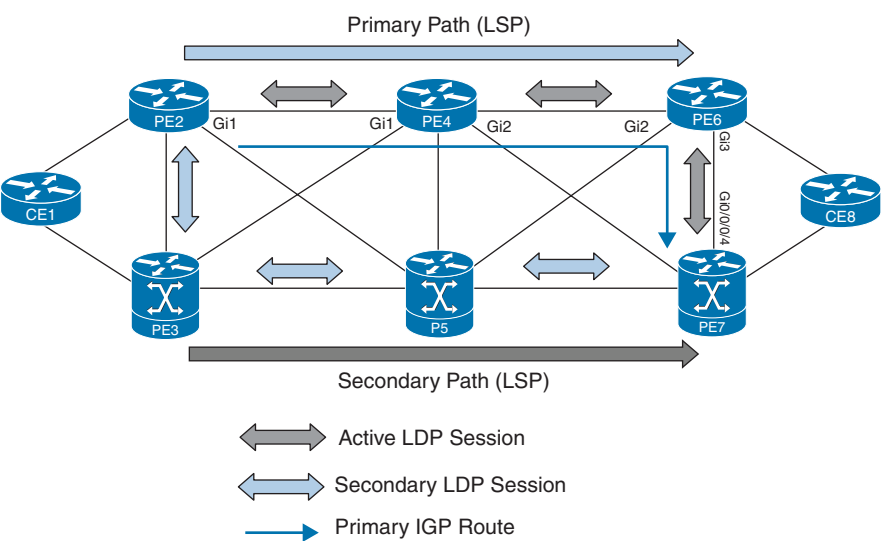
Figure 10-13 MPLS LDP IGP Synchronization
