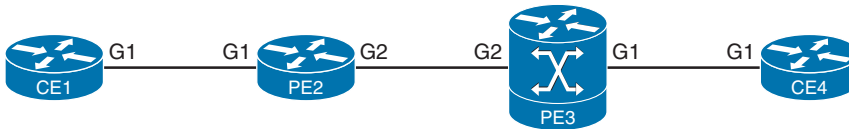
Figure 21-5 QoS Topology
