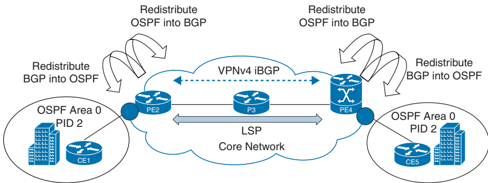
Figure 12-9 MPLS L3VPN OSPF PE-CE, IOS XR
