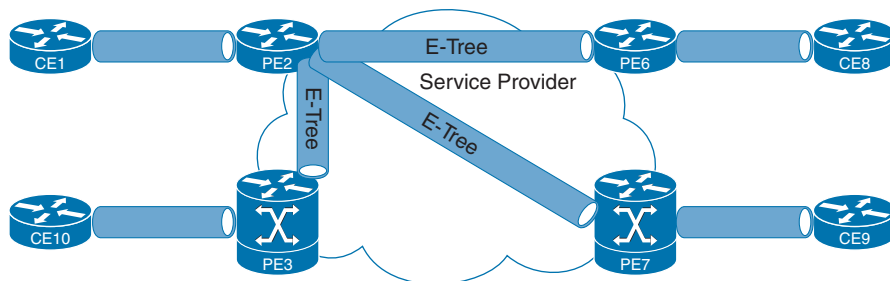
Figure 1-4 E-Tree Metro Point-to-Multipoint Ethernet Services
