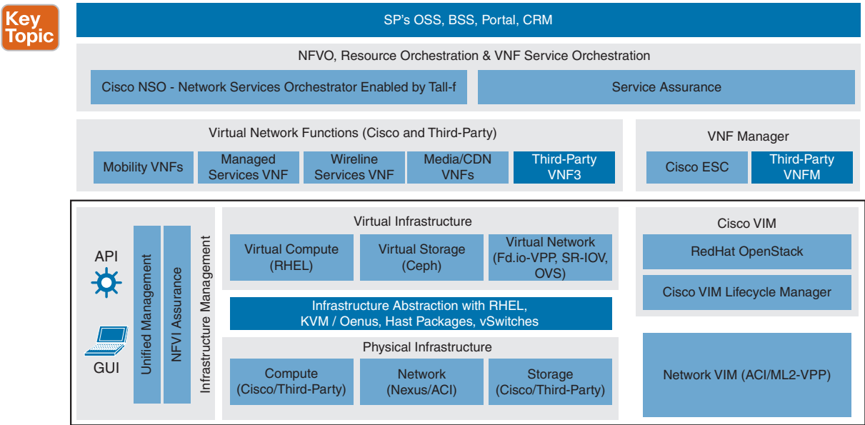
Figure 3-1 Scope of Cisco NFVI Solution
