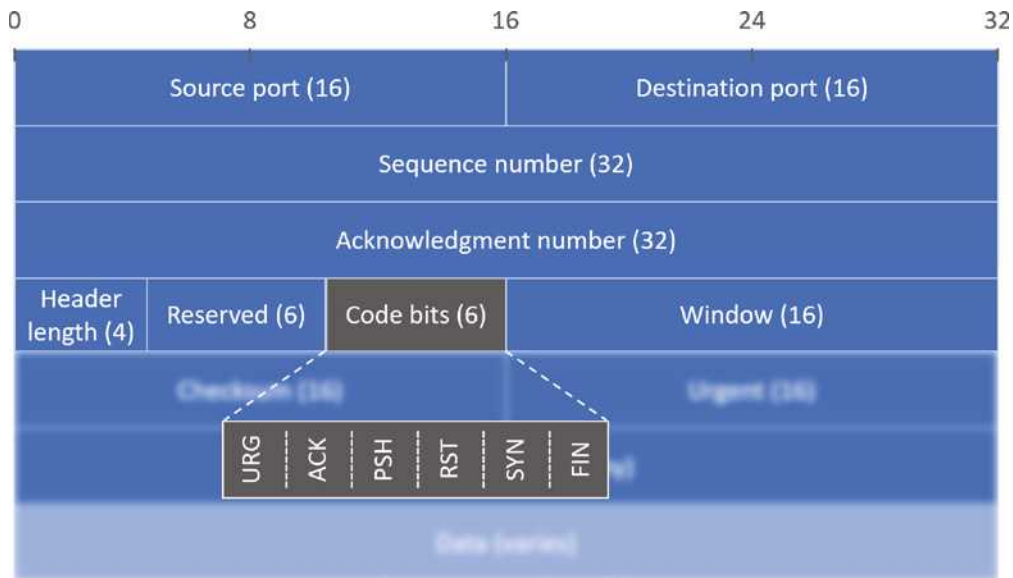
FIGURE 19.5 TCP flags
