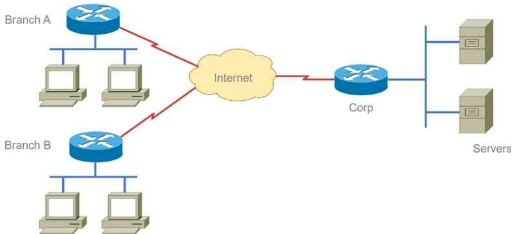
FIGURE 1.5 An internetwork
