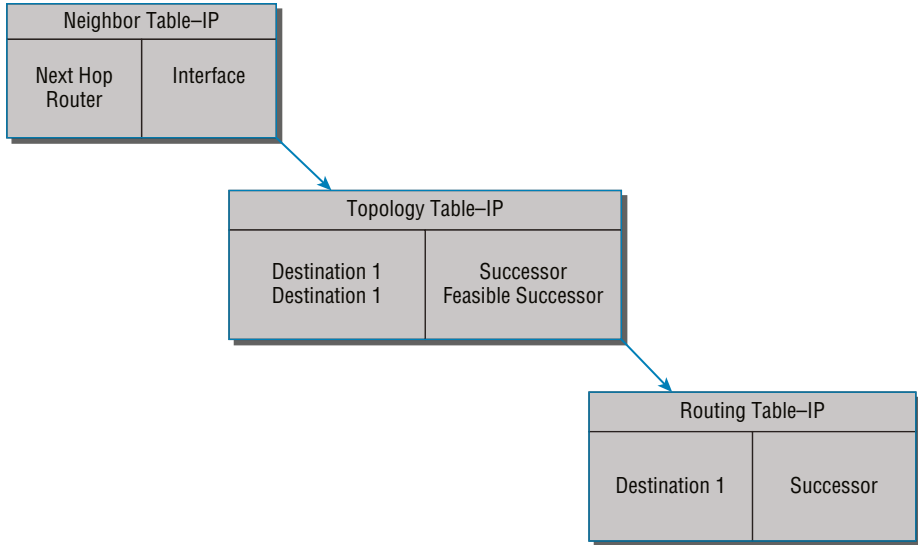
FIGURE 10.7 EIGRP tables
