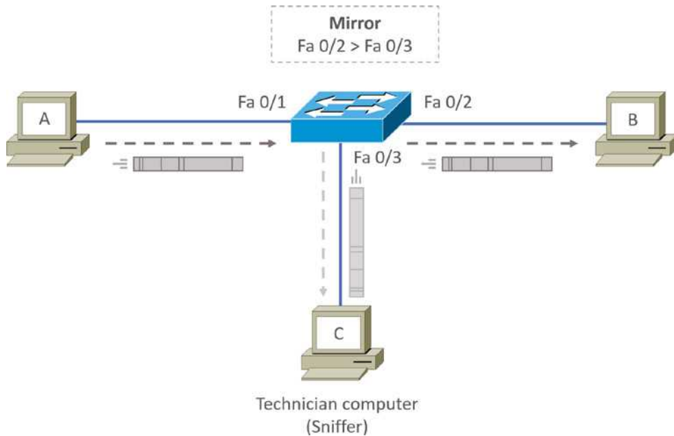
FIGURE 11.31 Port spanning/mirroring
