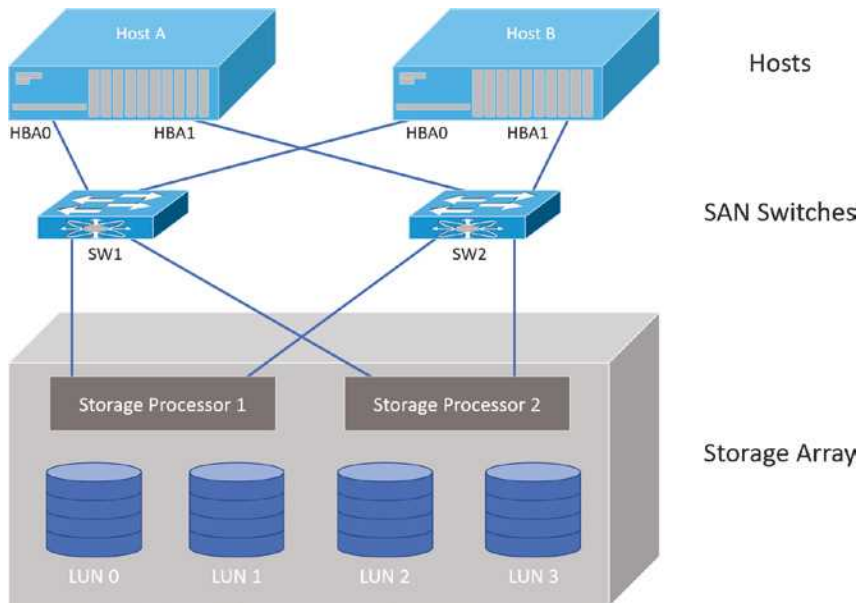
FIGURE 16.1 Multipathing
