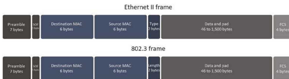
FIGURE 4.5 802.3 and Ethernet frame formats in bytes
