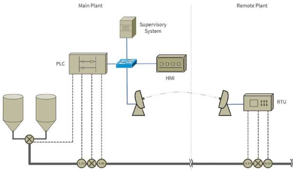
FIGURE 21.17 SCADA systems
