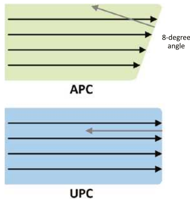
FIGURE 3.11 APC and UPC connectors
