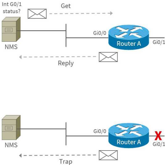
FIGURE 14.4 SNMP get and trap methods
