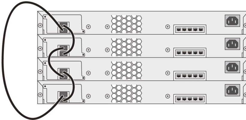
FIGURE 16.4 Switch stacking
