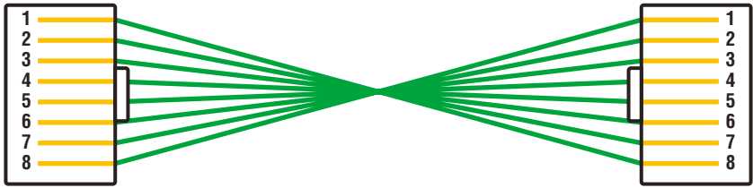
FIGURE 3.26 Rolled Ethernet cable
