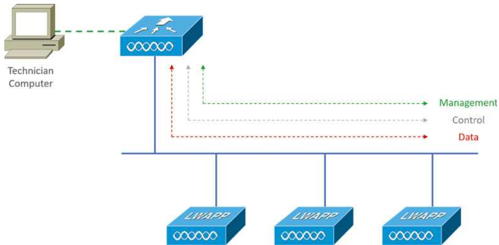
FIGURE 12.14 LWAPP
