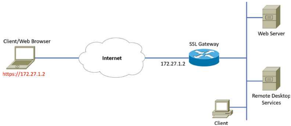
FIGURE 13.2 Clientless VPN
