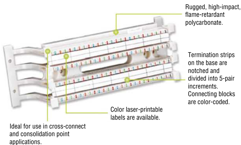
FIGURE 3.28 A 110 block
