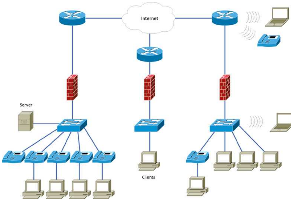
FIGURE 15.3 Network diagram with firewalls from SmartDraw
