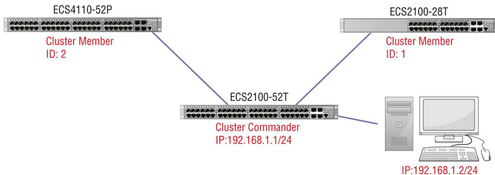
FIGURE 16.5 Switch cluster
