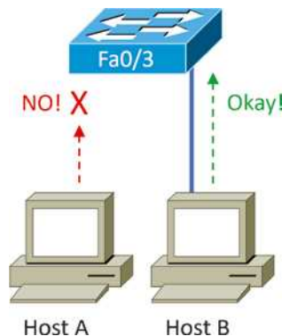
FIGURE 11.23 Port security on a switch port restricts port access by MAC address.
