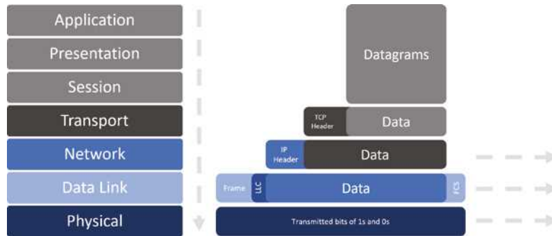
FIGURE 6.21 Data encapsulation
