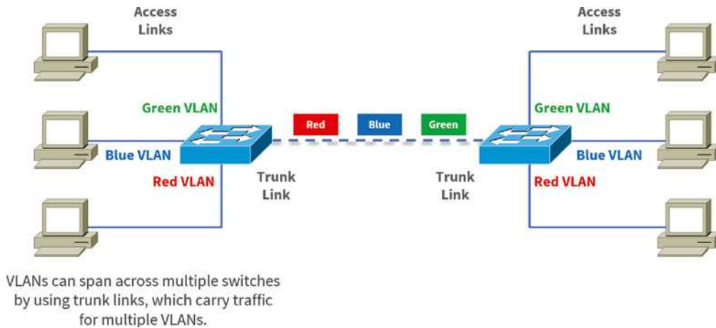
FIGURE 11.17 Access and trunk links in a switched network
