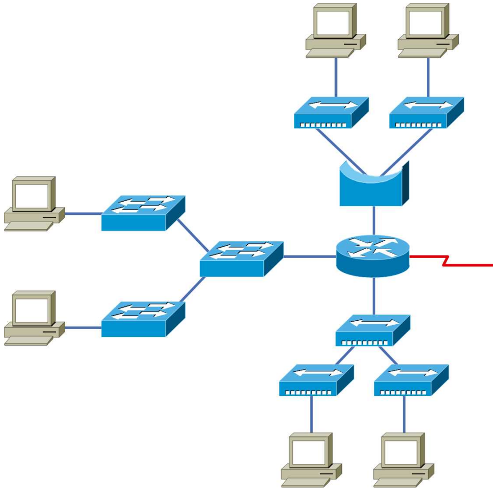
FIGURE 5.28 Internetworking devices
