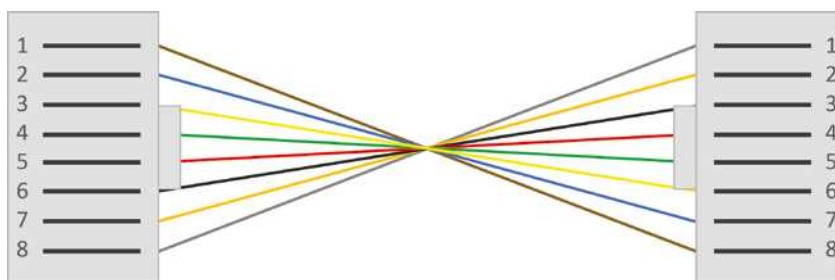
FIGURE 18.1 A router/switch console connection
