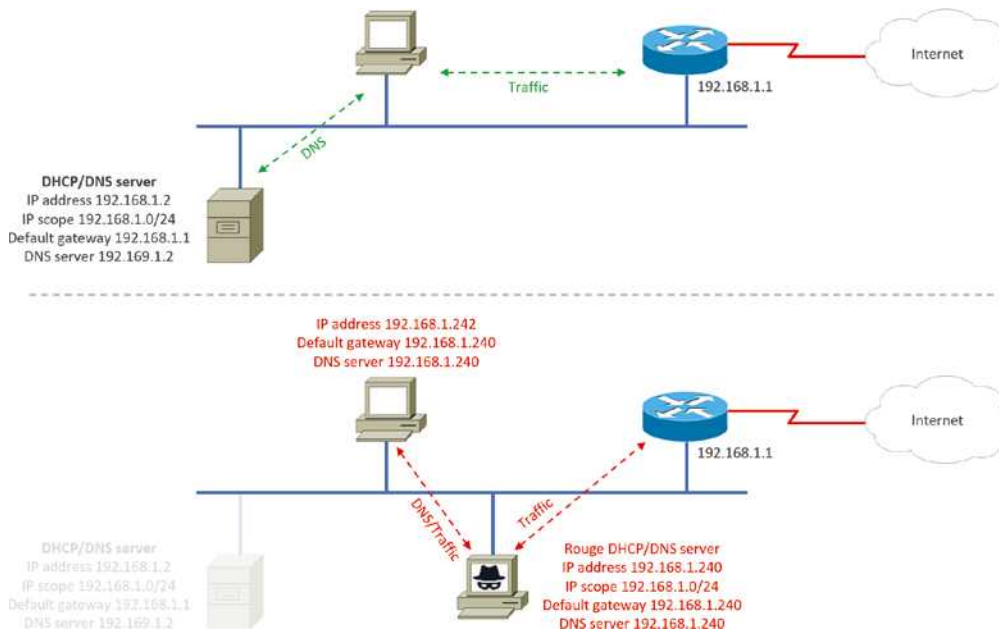
FIGURE 18.7 Rogue DHCP
