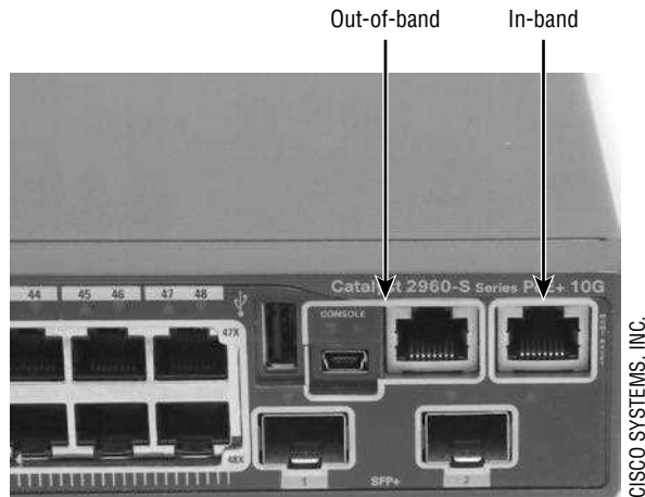
FIGURE 13.7 A Cisco 2960 console connections
