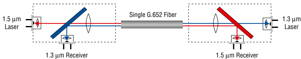
FIGURE 3.12 Bidirectional communication
