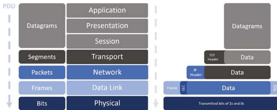
FIGURE 2.11 Data encapsulation
