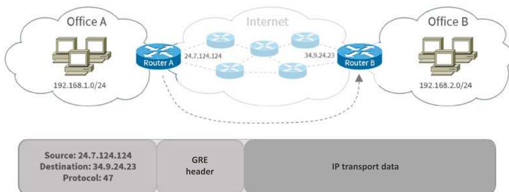
FIGURE 6.20 Generic Routing Encapsulation (GRE) tunnel structure
