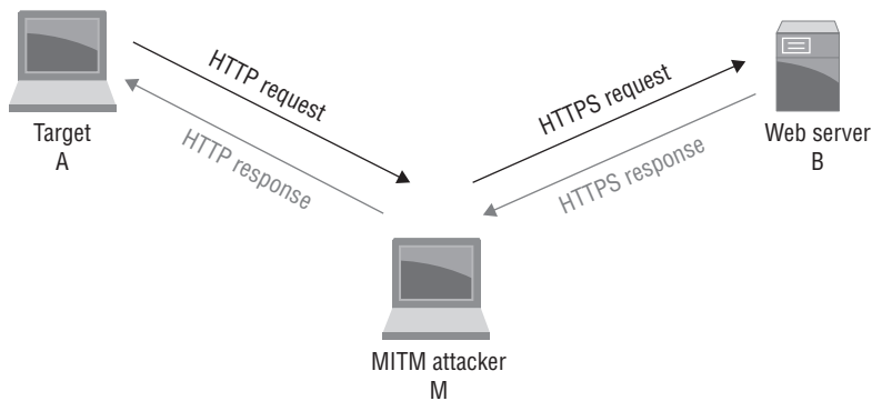
FIGURE 7.5 SSL stripping attack
