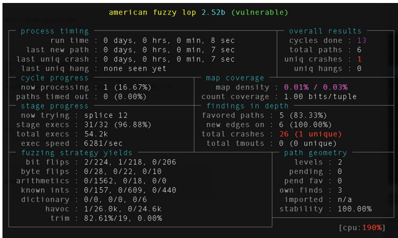
FIGURE 9.17 american fuzzy lop performing fuzz testing
