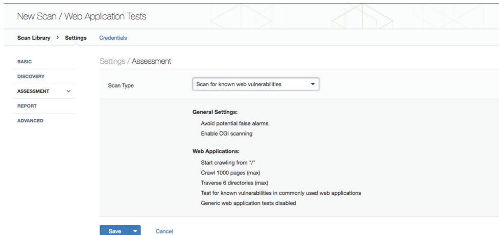
FIGURE 4.13 Nessus web application scanner
