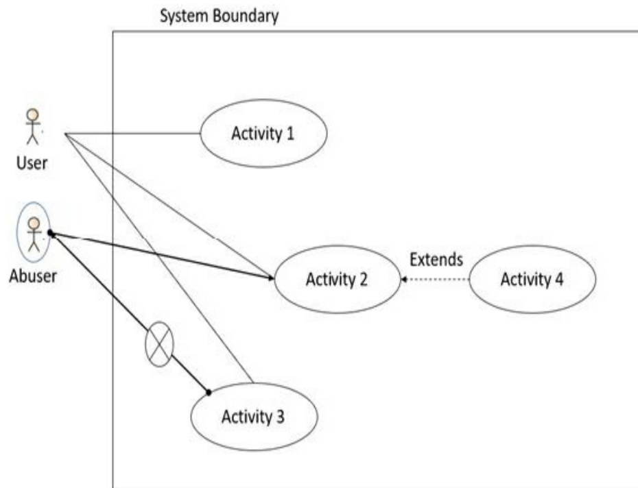
Figure 15.9 Example Mis-use case diagram
