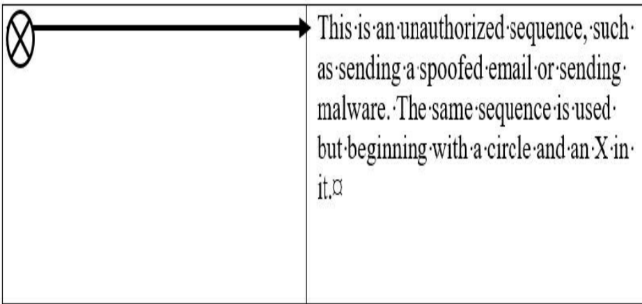
Figure 15.13 Cybersecurity additions to sequence diagrams
