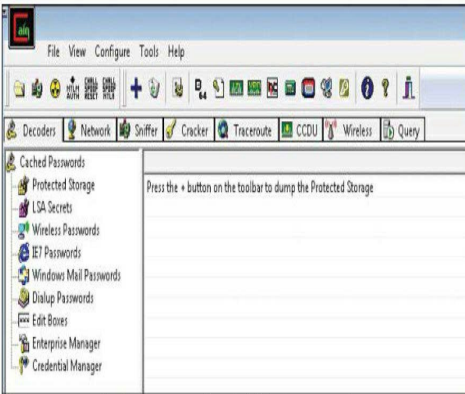
Figure 6.4 Cain and Abel.
