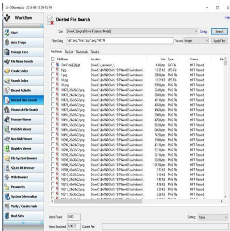
Figure 14.11 OSForensics Deleted File Search.
