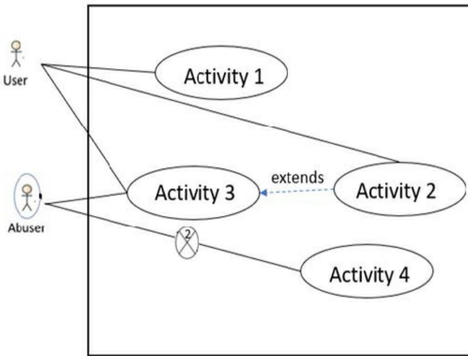
Figure 15.10 Another Misuse Case Example
