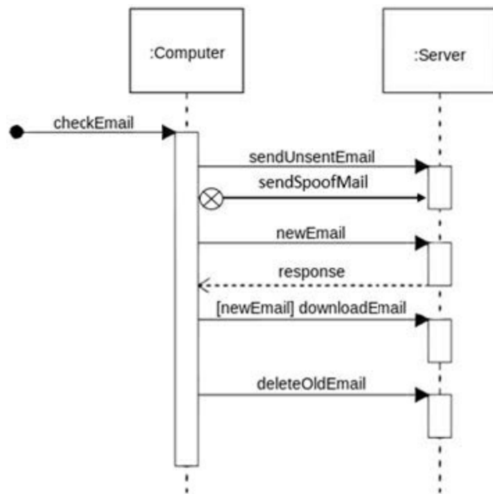
Figure 5.14 Modified Sequence Diagram
