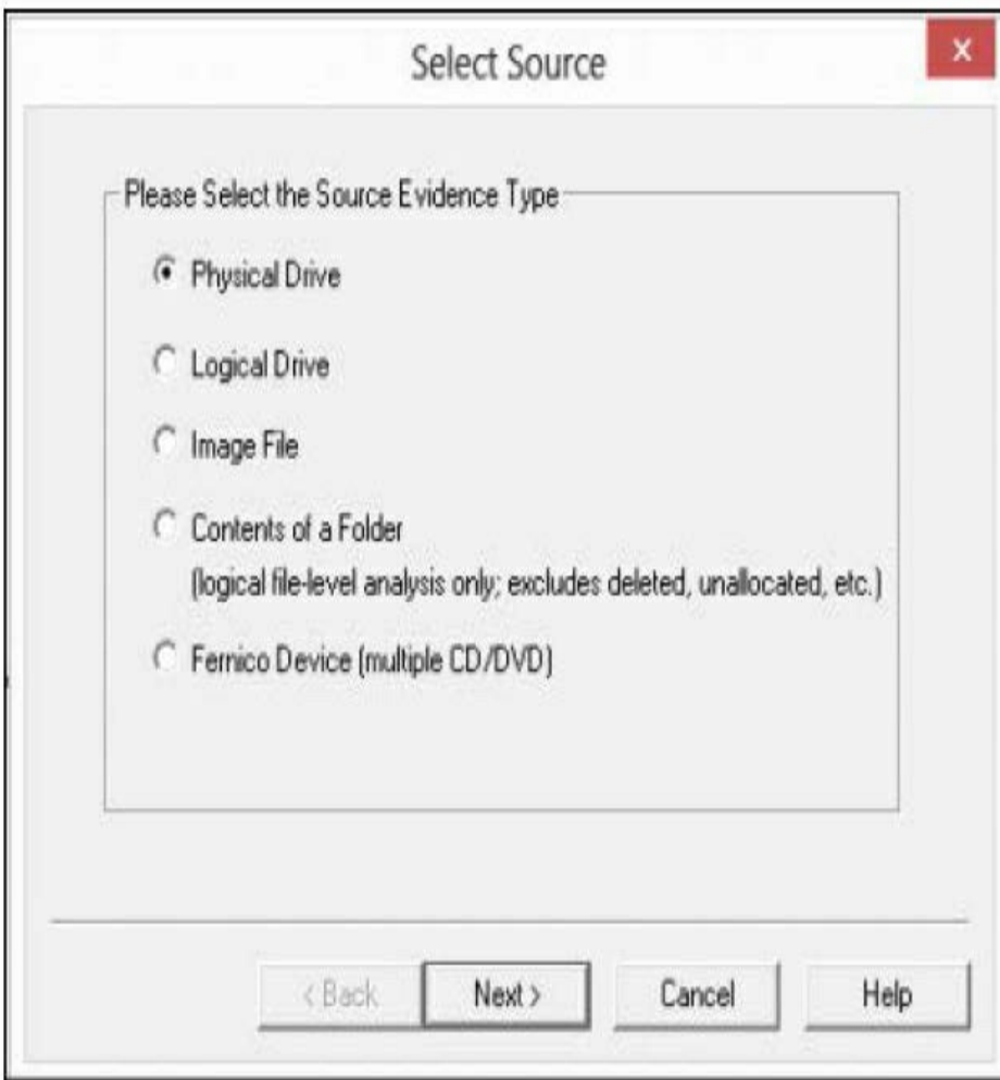
Figure 14.3 FTK Imager—Select Source.
