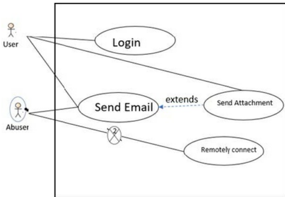
Figure 15.11 Specific Misuse Case Example
