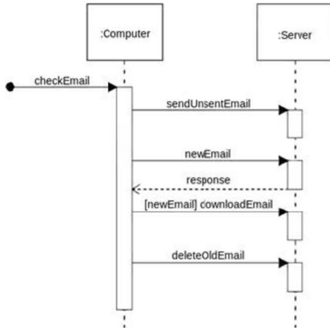
Figure 15.12 UML/SysML Sequence Diagram
