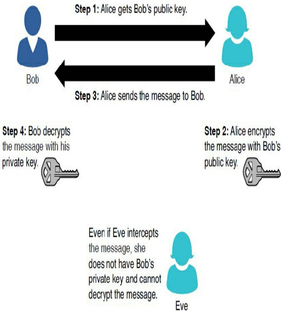
Figure 8.7 Public key cryptography.
