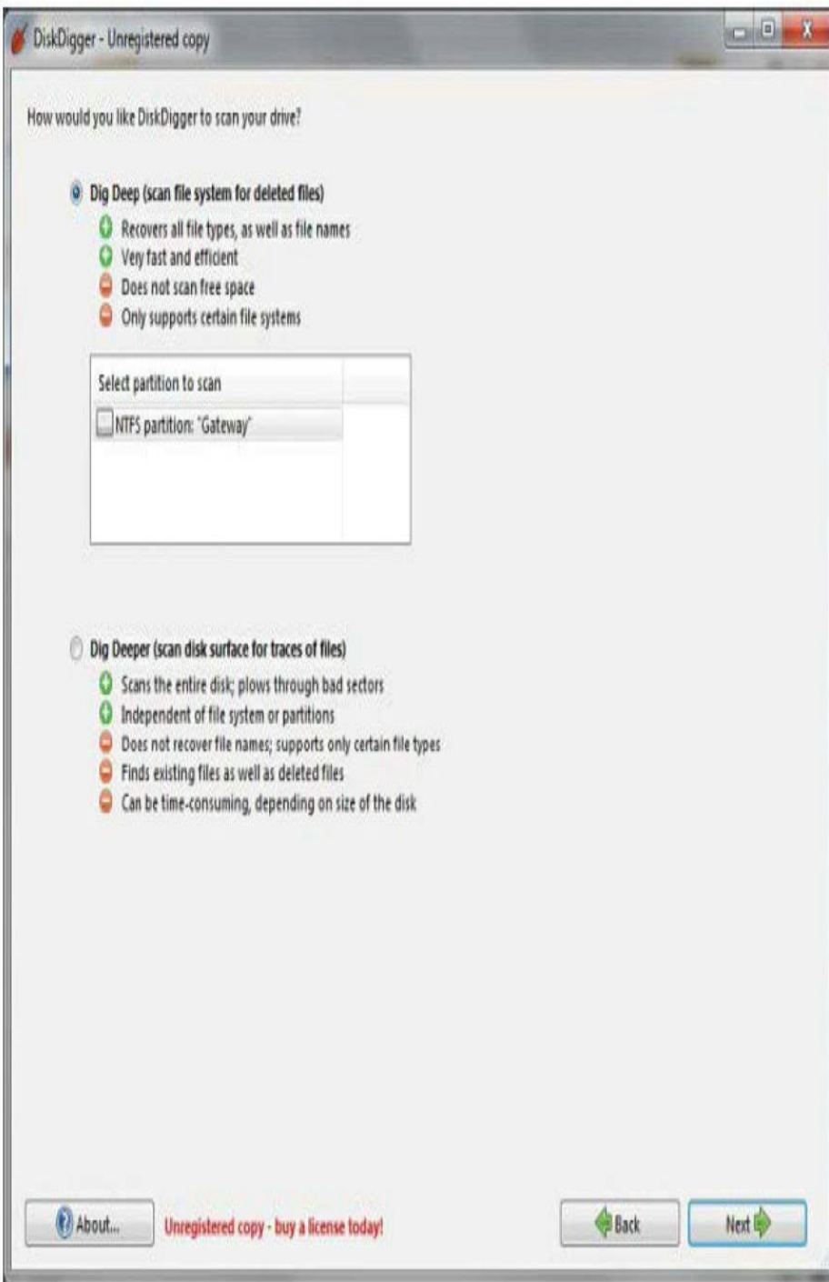
Figure 14.9 Select depth of scan.
