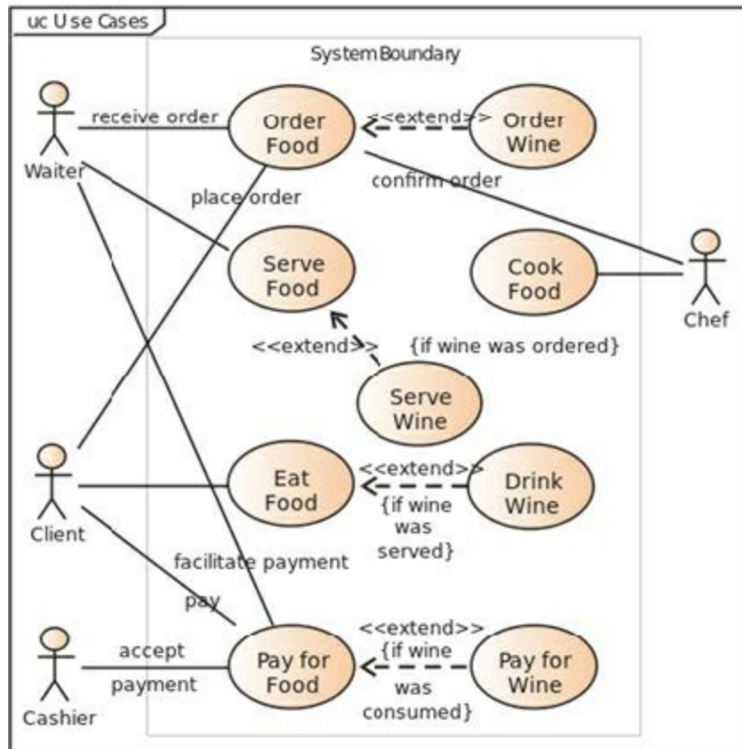
Figure 15.7 Typical Use Case Diagram
