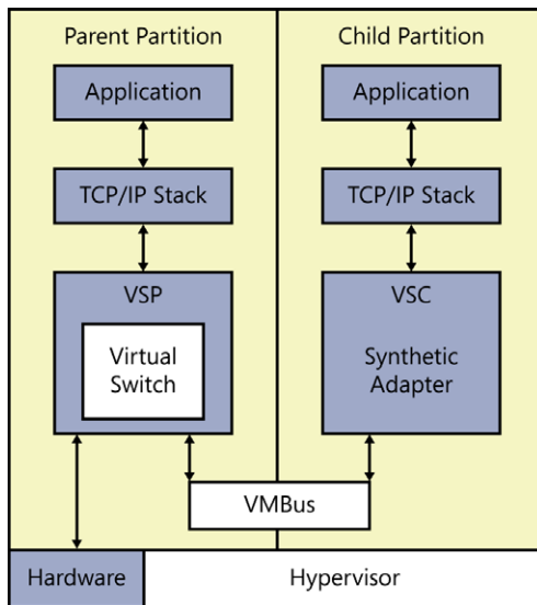
FIGURE 3-28 Synthetic network adapters communicate by using the VMBus.
