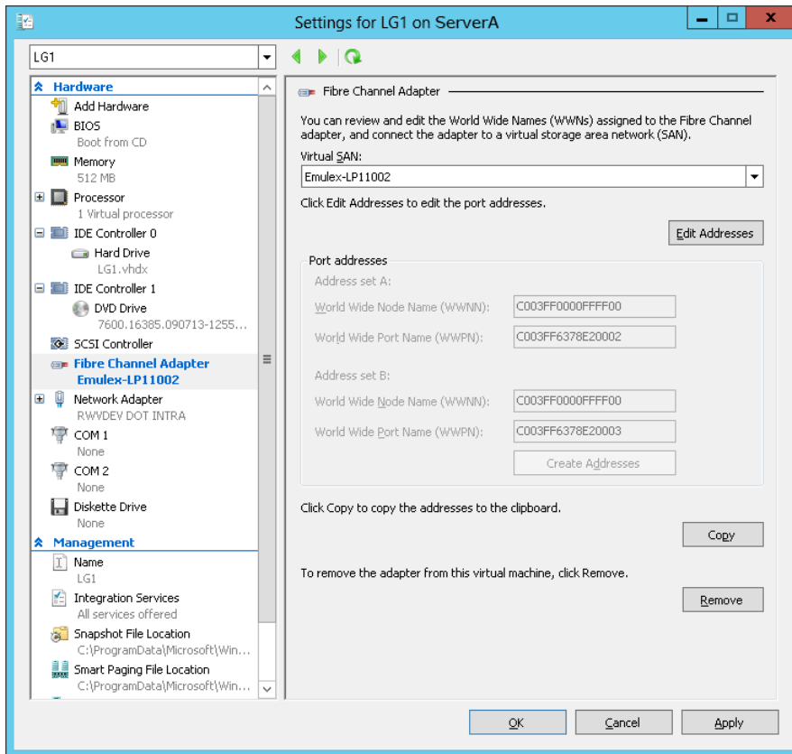
FIGURE 3-22 A Fibre Channel adapter in a VM.
