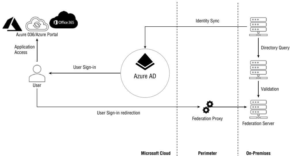
FIGURE 3.5 Microsoft federated authentication reference architecture
