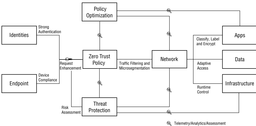
FIGURE 1.1 Microsoft Zero Trust architecture
