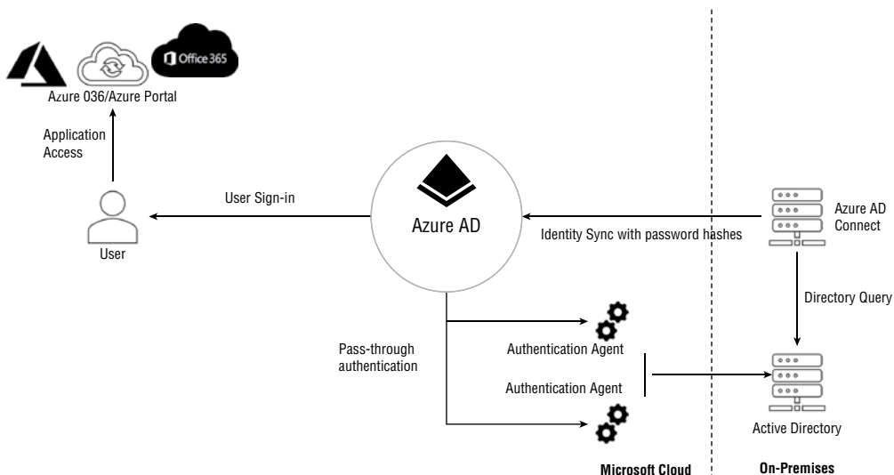
FIGURE 3.4 Microsoft Azure AD pass-through authentication reference architecture
