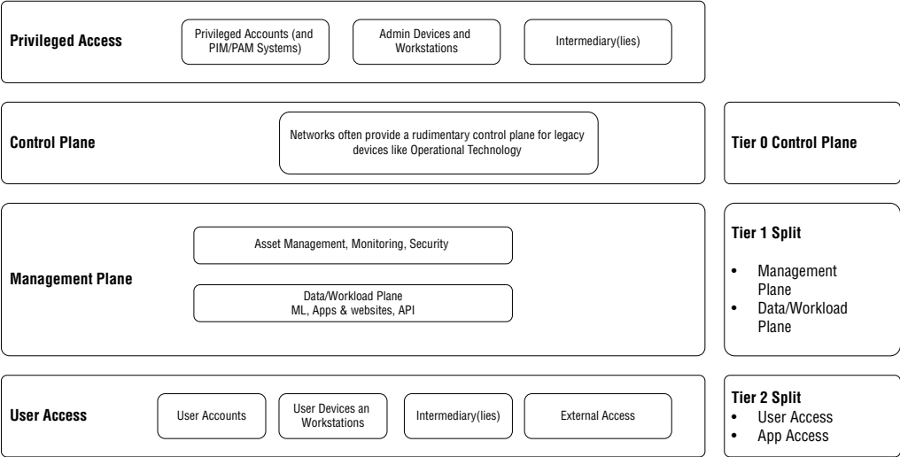
FIGURE 3.1 Enterprise access solution based on Zero Trust
