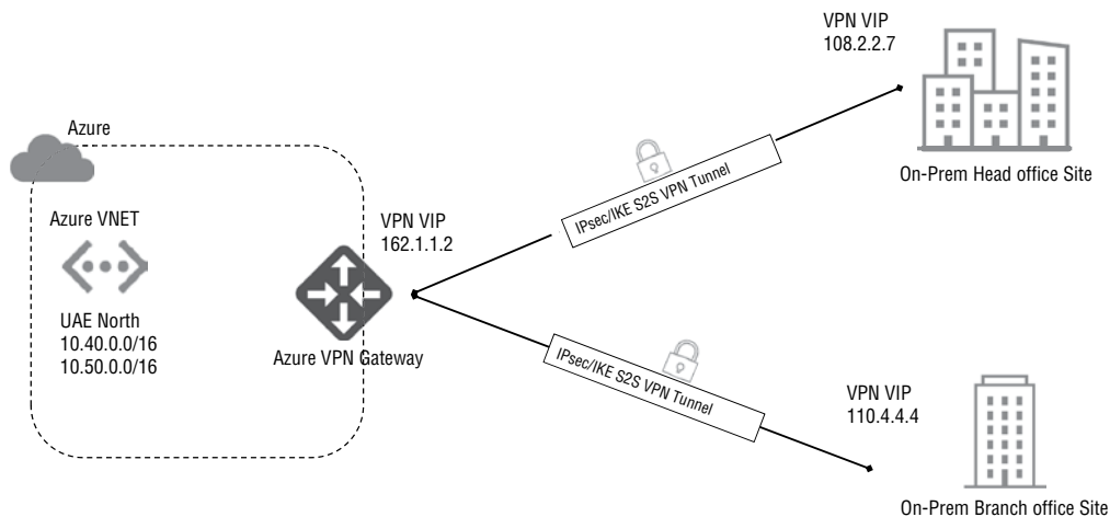
FIGURE 6.10 Microsoft Azure multisite S2S VPN
