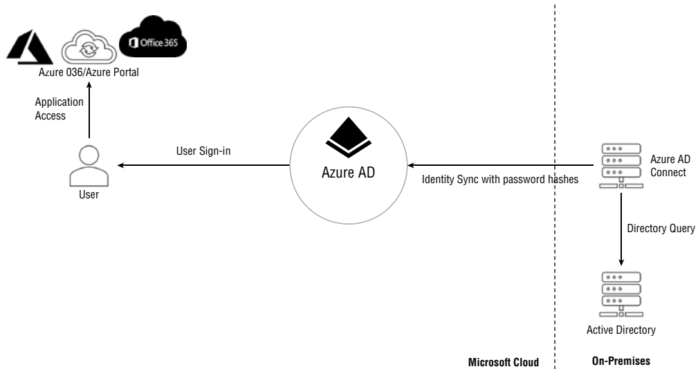
FIGURE 3.3 Microsoft Azure AD password hash synchronization reference architecture
