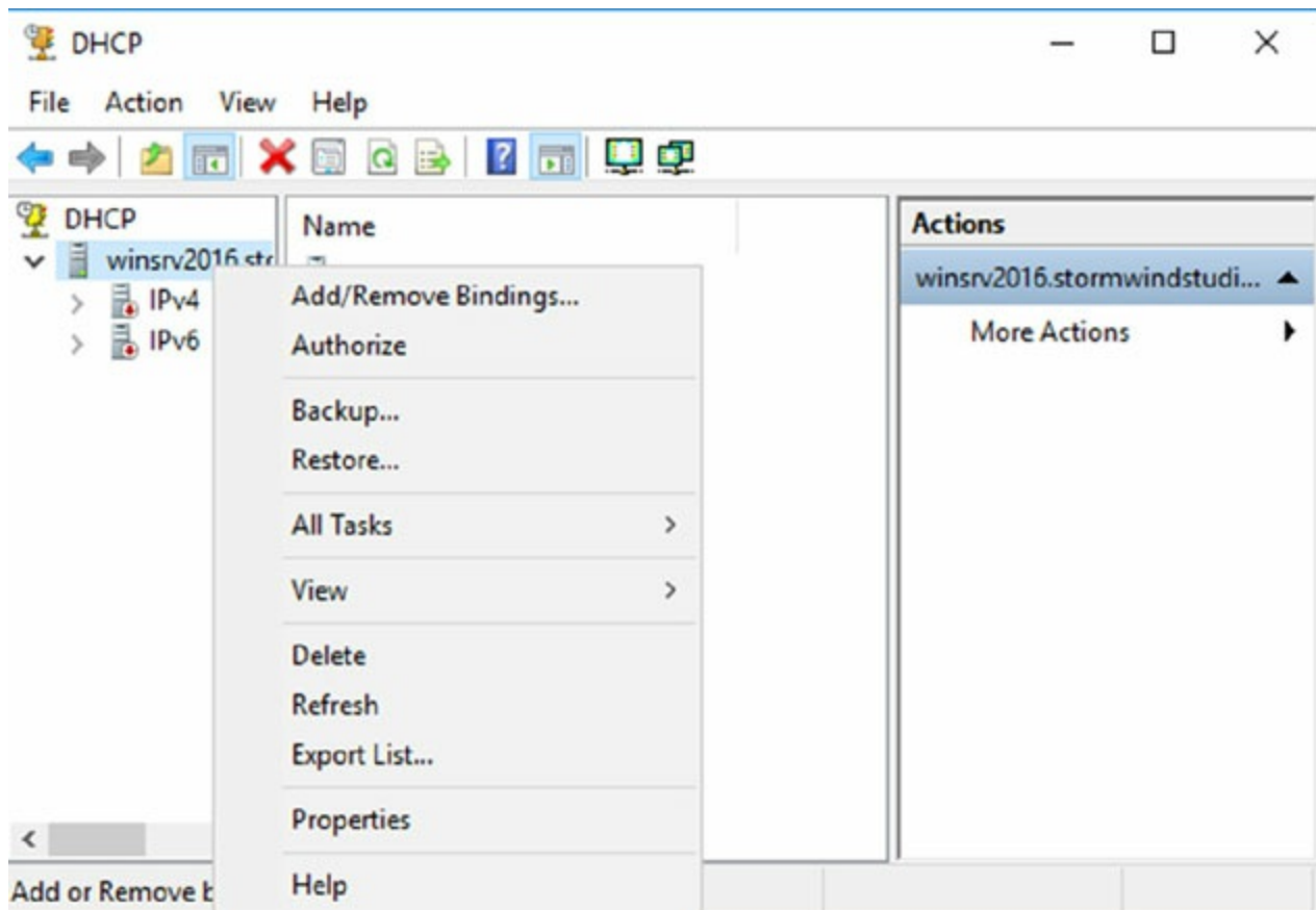
FIGURE 3.3 Choosing Authorize
