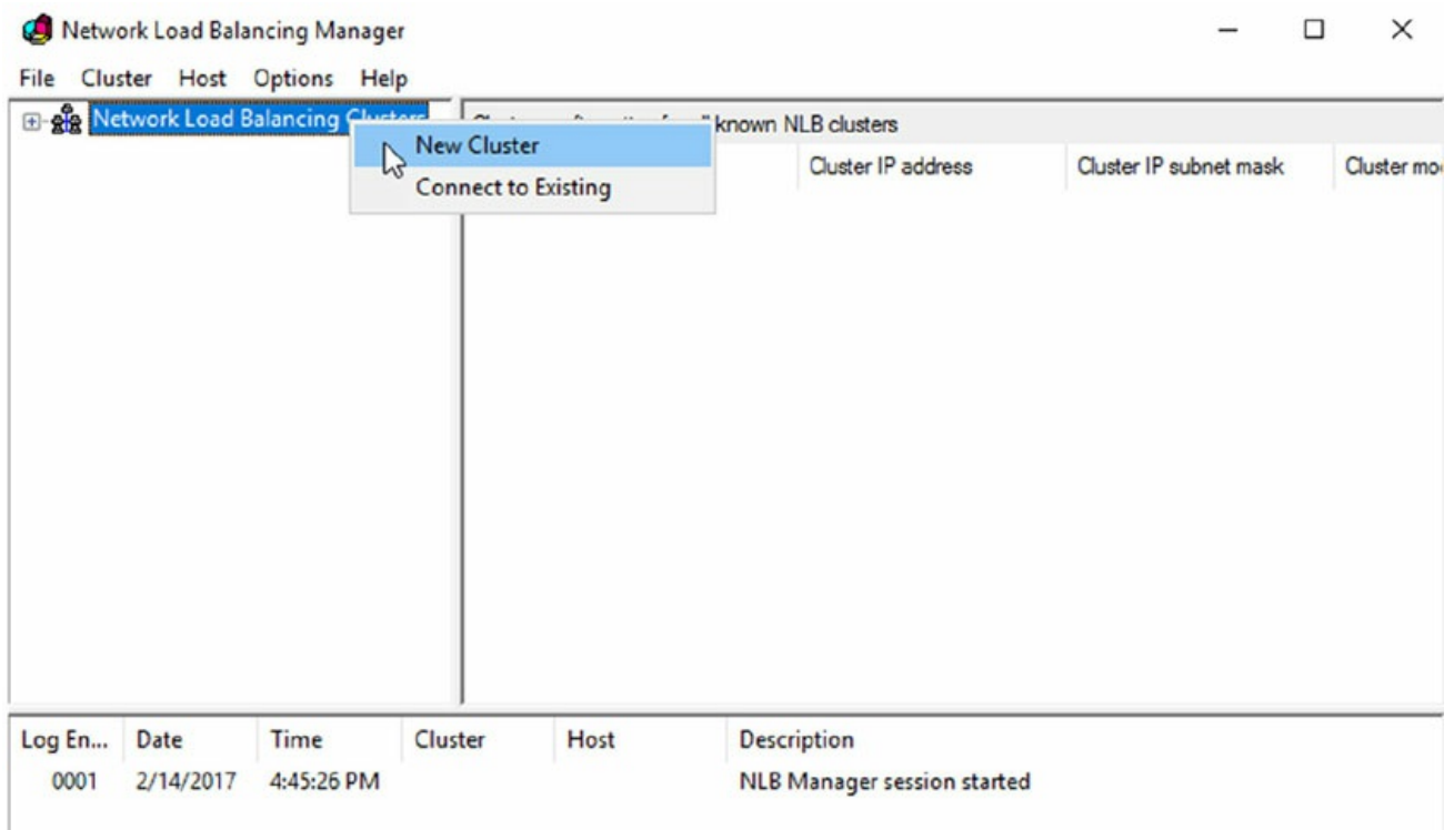
FIGURE 7.2 New Cluster
