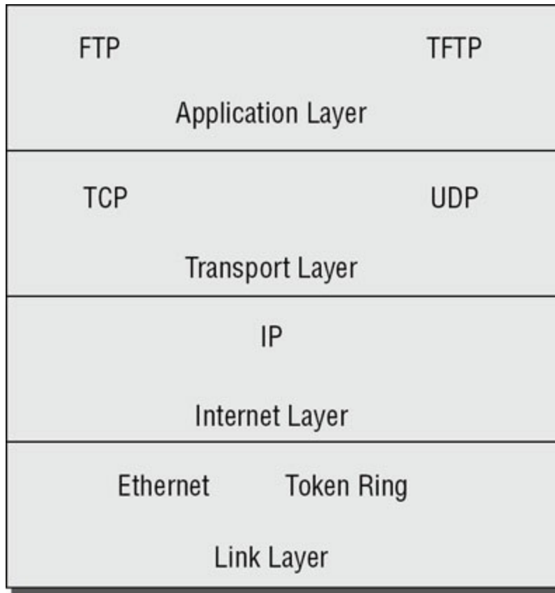
FIGURE 1.1 TCP/IP model
