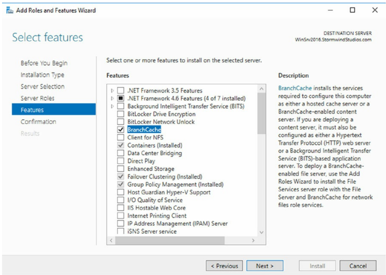
FIGURE 6.7 BranchCache Option
