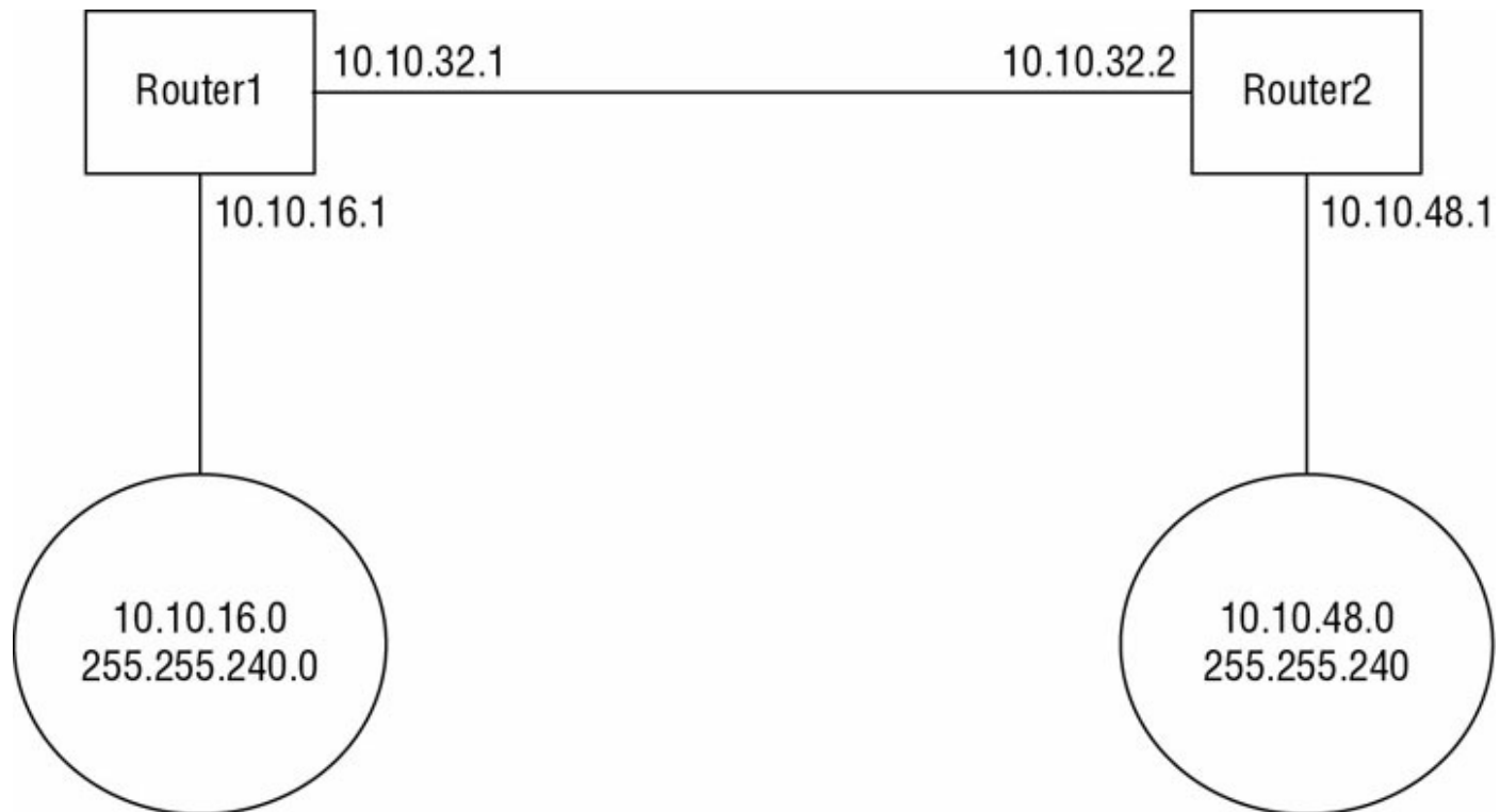
FIGURE 5.15 Network Layout
