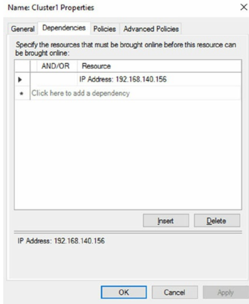
FIGURE 7.17 Resource dependencies
