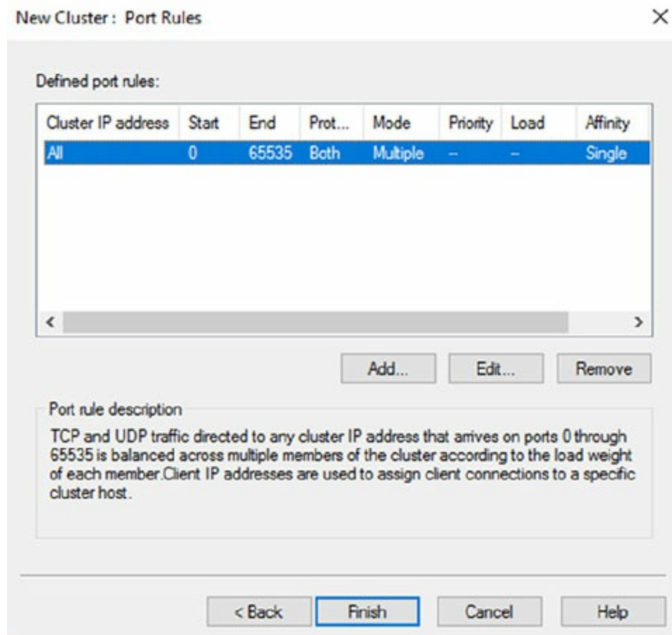
FIGURE 7.6 Port Rules
