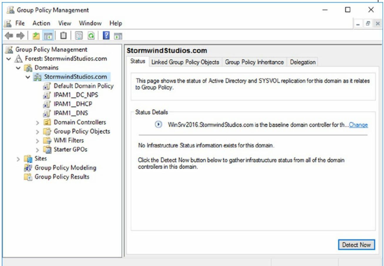
FIGURE 4.6 New GPOs
