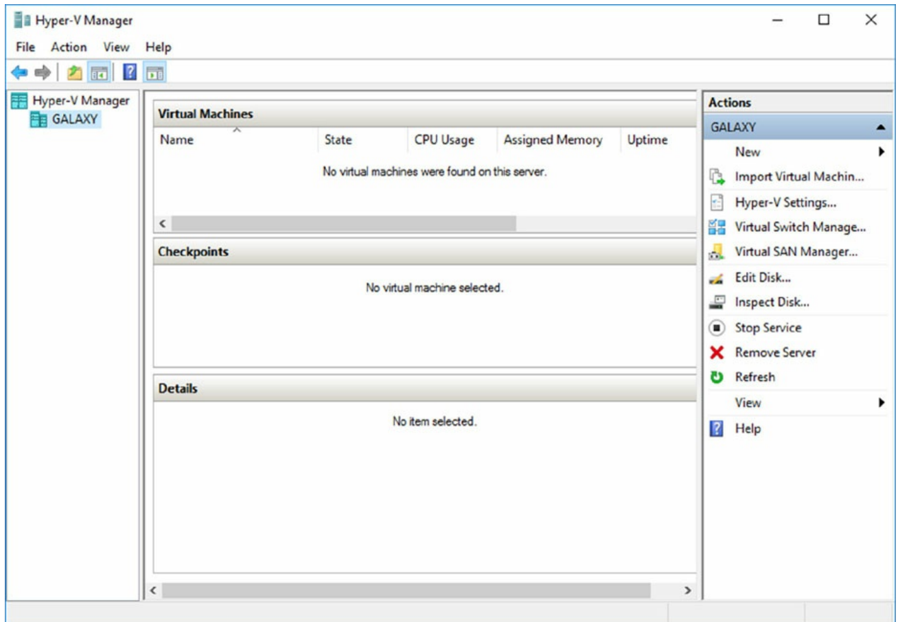
FIGURE 8.12 Hyper-V Manager
