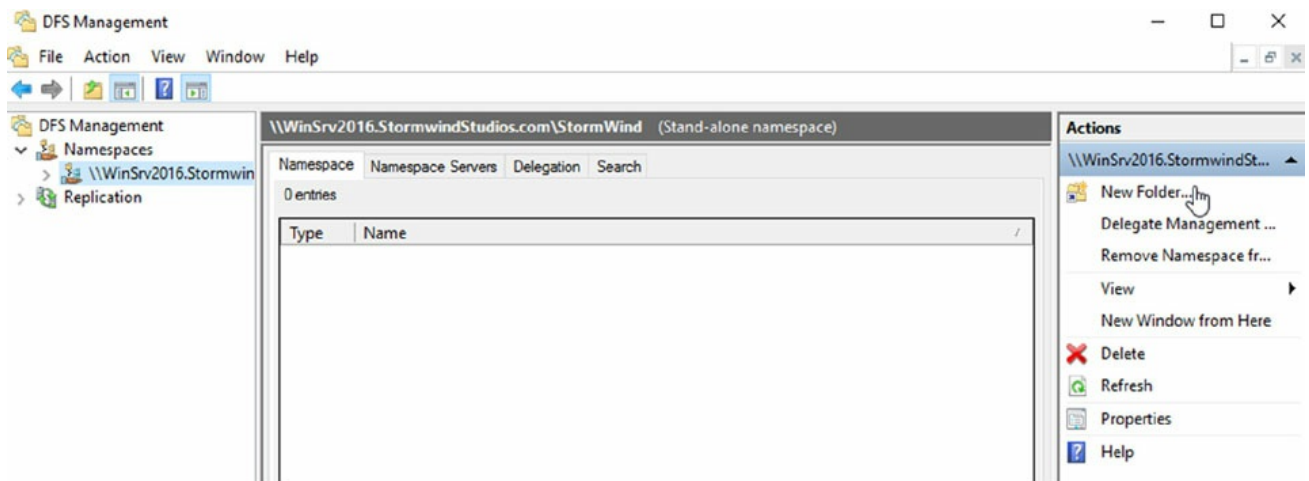
FIGURE 6.5 New Folder
