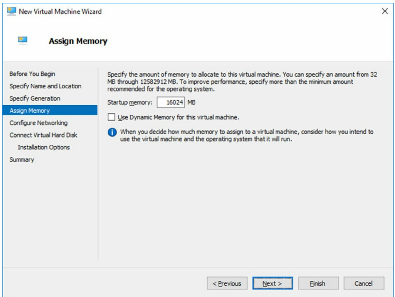
FIGURE 8.14 VM RAM
