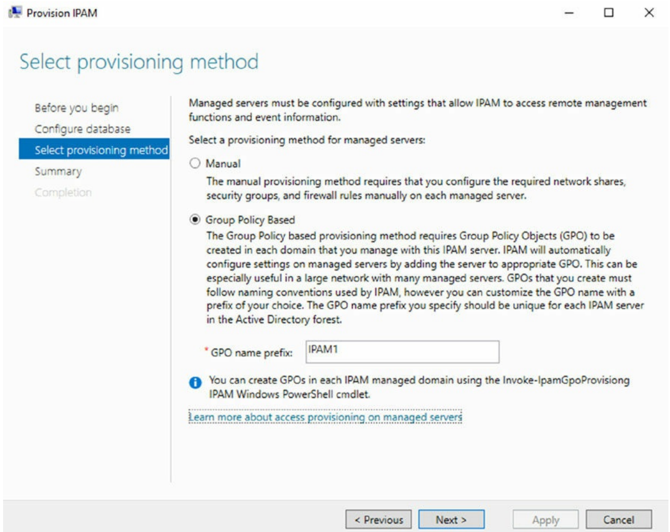
FIGURE 4.4 Select Provisioning
