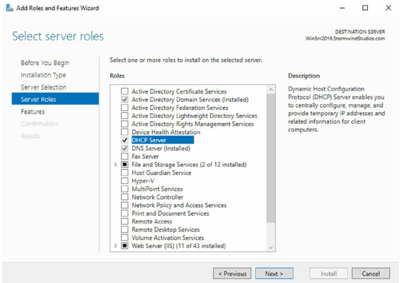
FIGURE 3.1 Choosing DHCP
