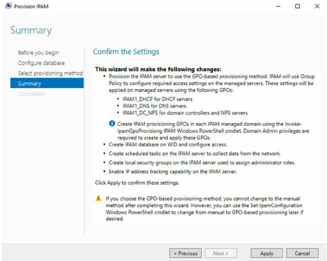
FIGURE 4.5 GPOs Needed
