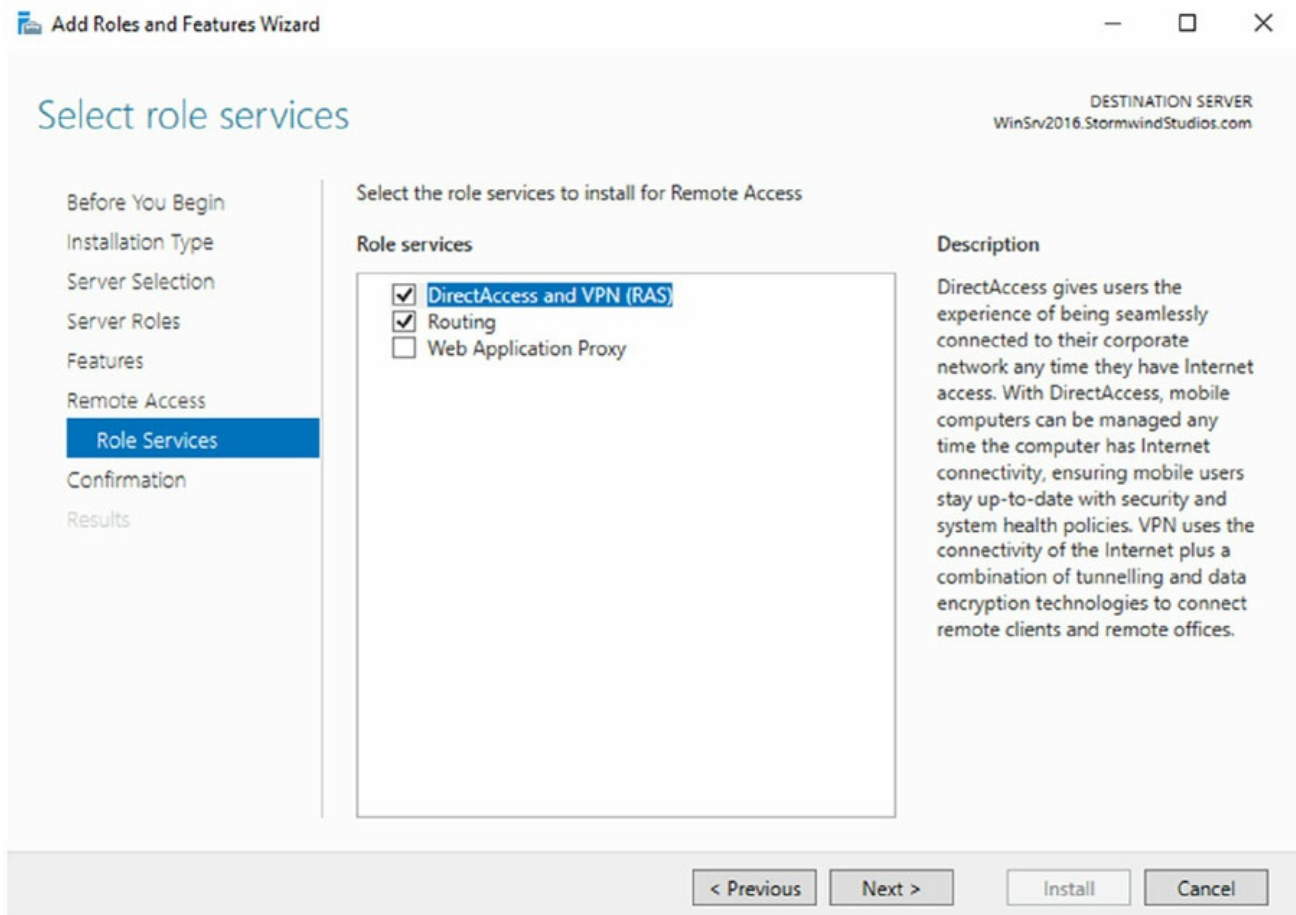
FIGURE 5.7 Remote Access
