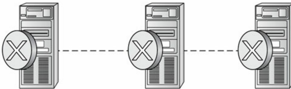
FIGURE 7.9 Majority needed
