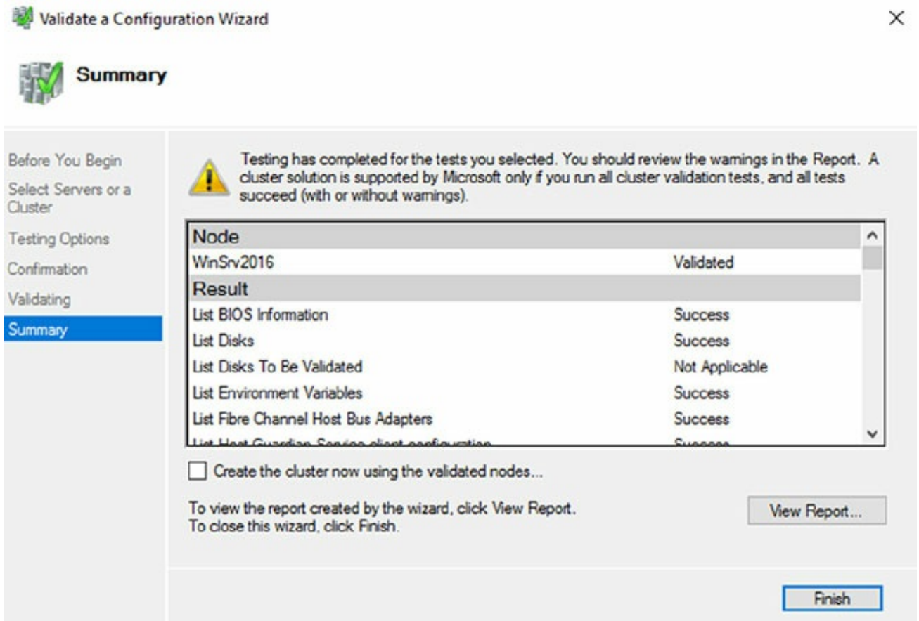
FIGURE 7.13 Cluster Tests
