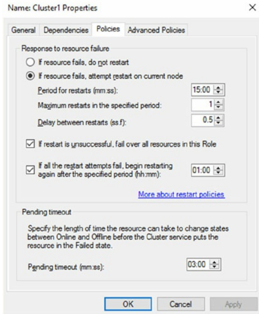
FIGURE 7.18 Resource policies
