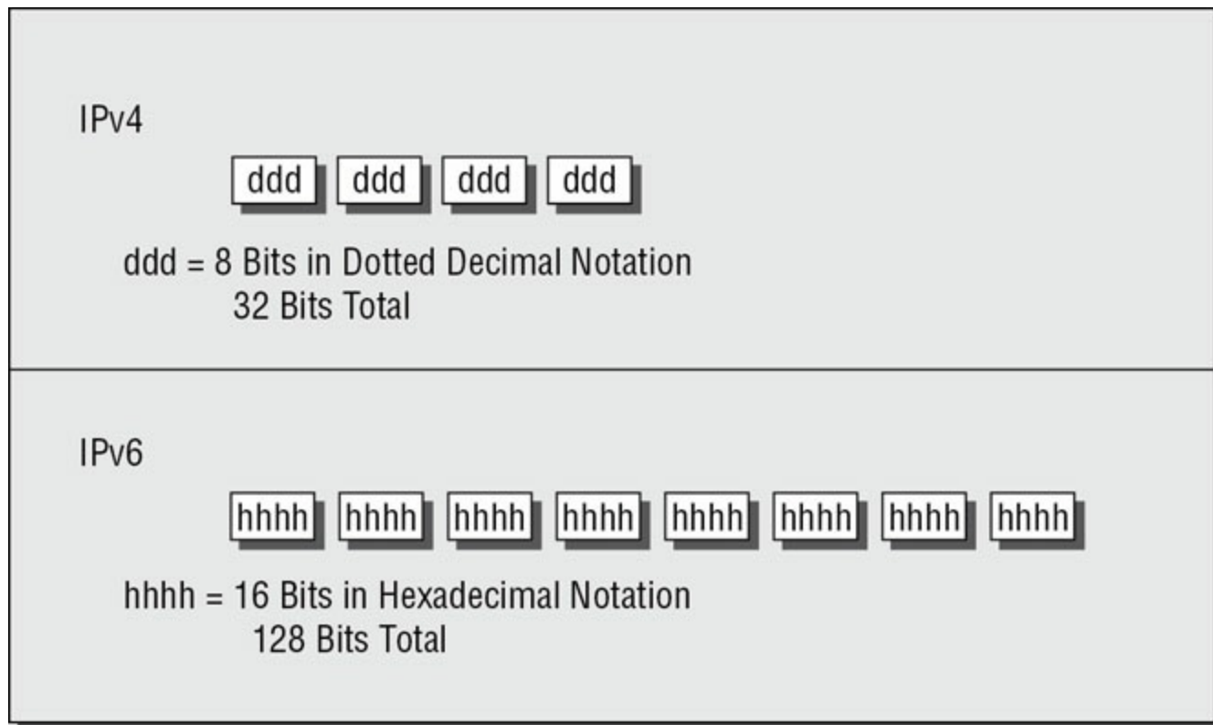
FIGURE 1.13 IPv4/IPv6 comparison
