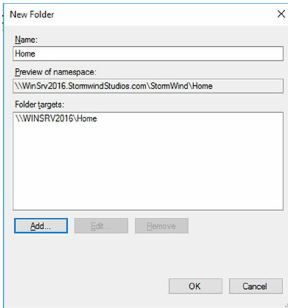
FIGURE 6.6 Home Folder
