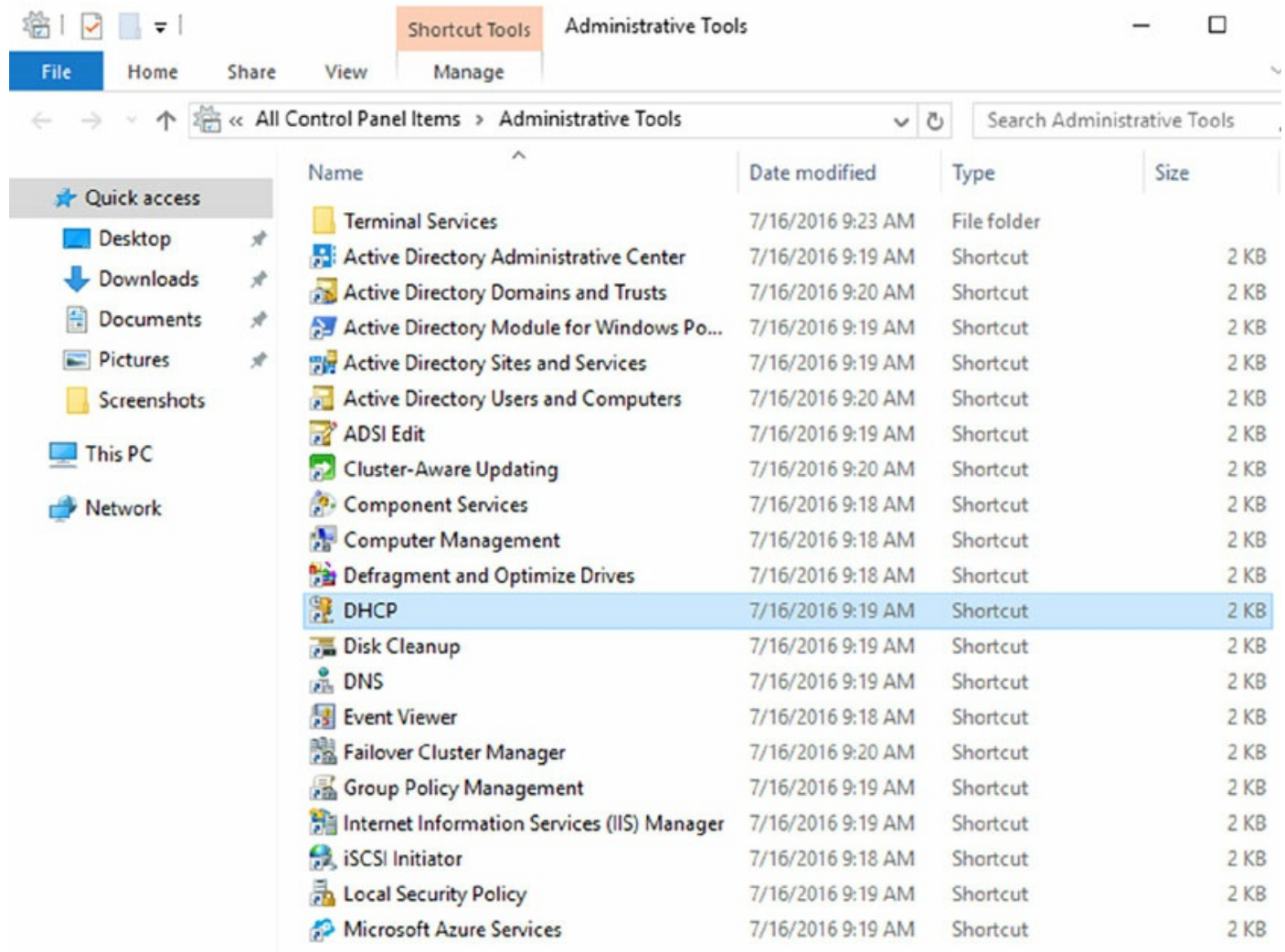
FIGURE 3.2 DHCP snap-in
