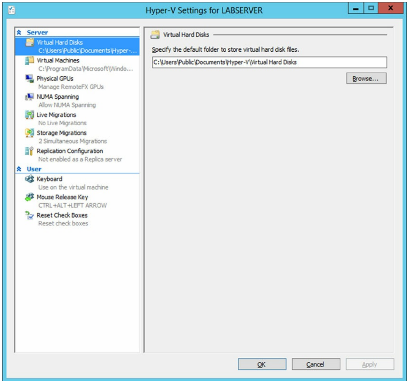
FIGURE 8.7 Hyper-V Settings
