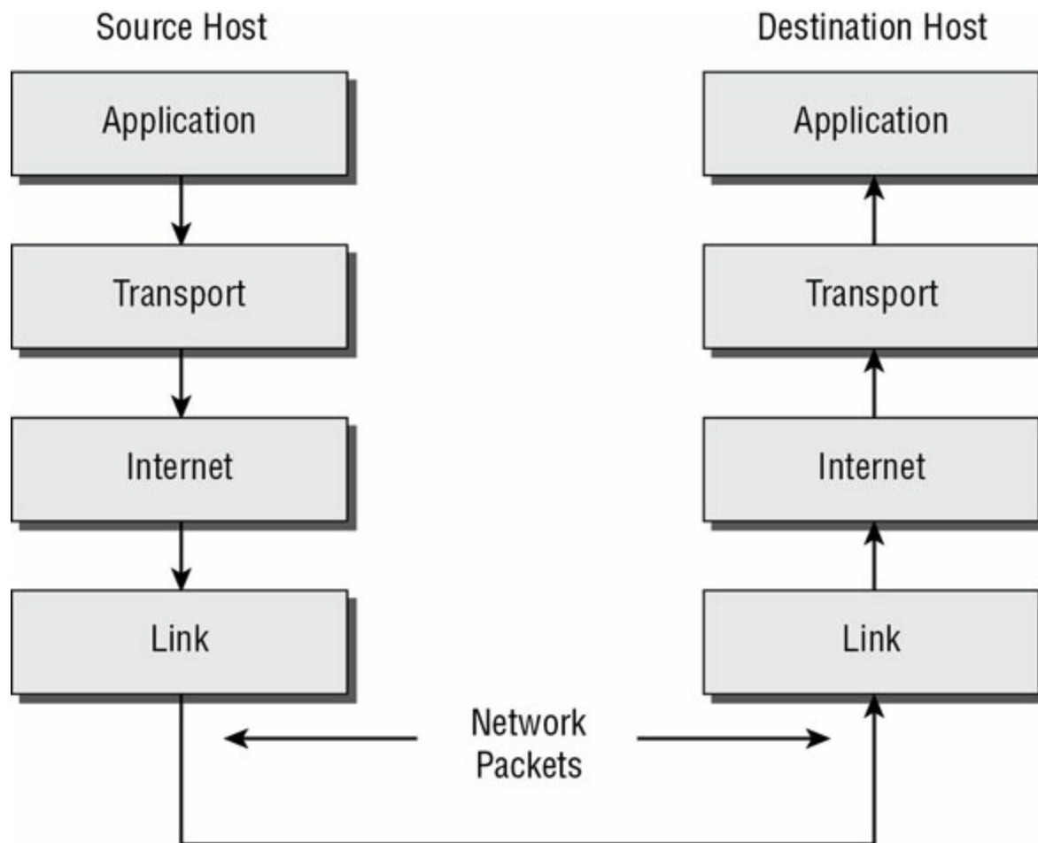
FIGURE 1.2 TCP/IP process
