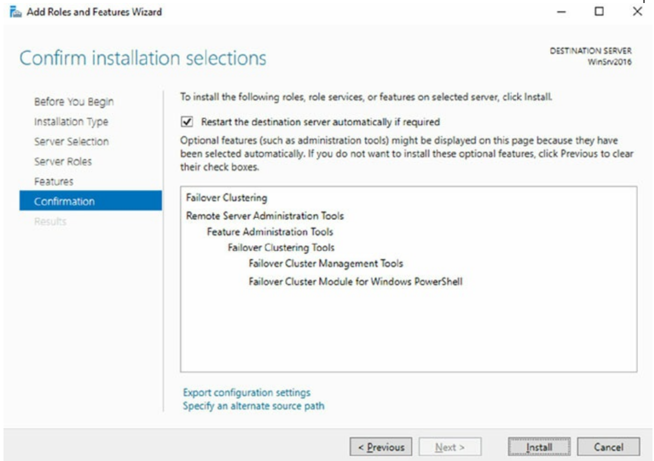
FIGURE 7.11 Confirmation Screen
