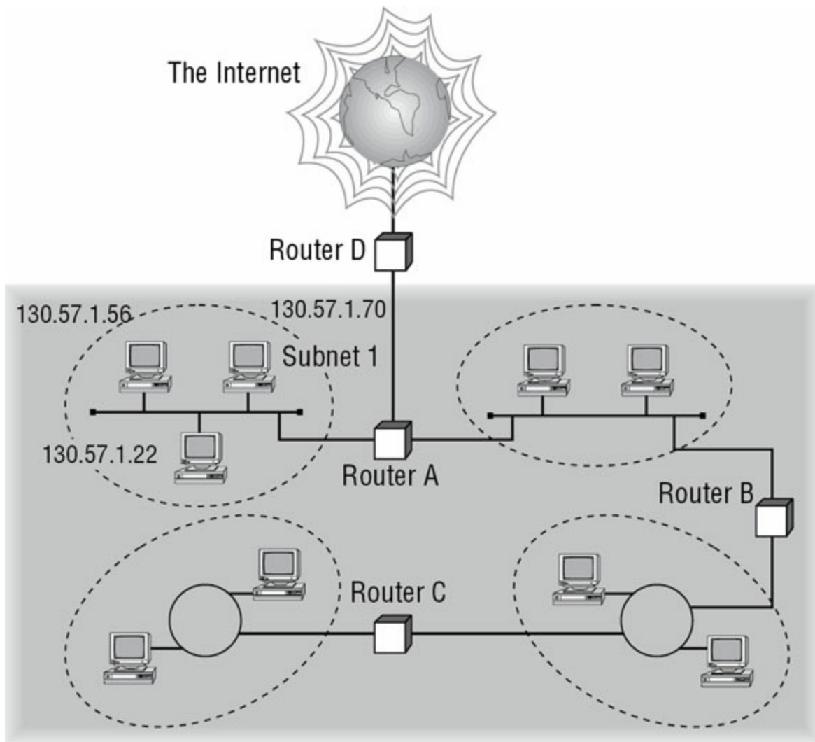
FIGURE 1.5 The network address and its subnet
