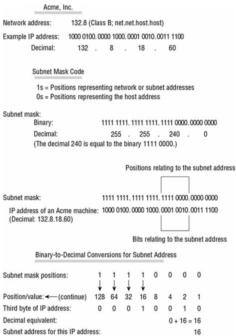
FIGURE 1.10 An example of a smaller subnet address
