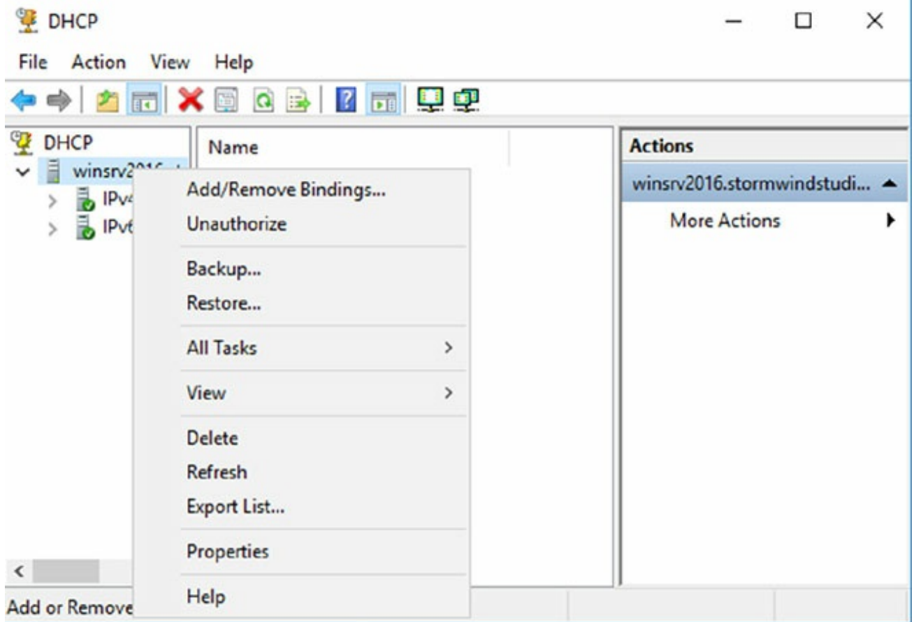
FIGURE 3.4 Choosing Unauthorize
