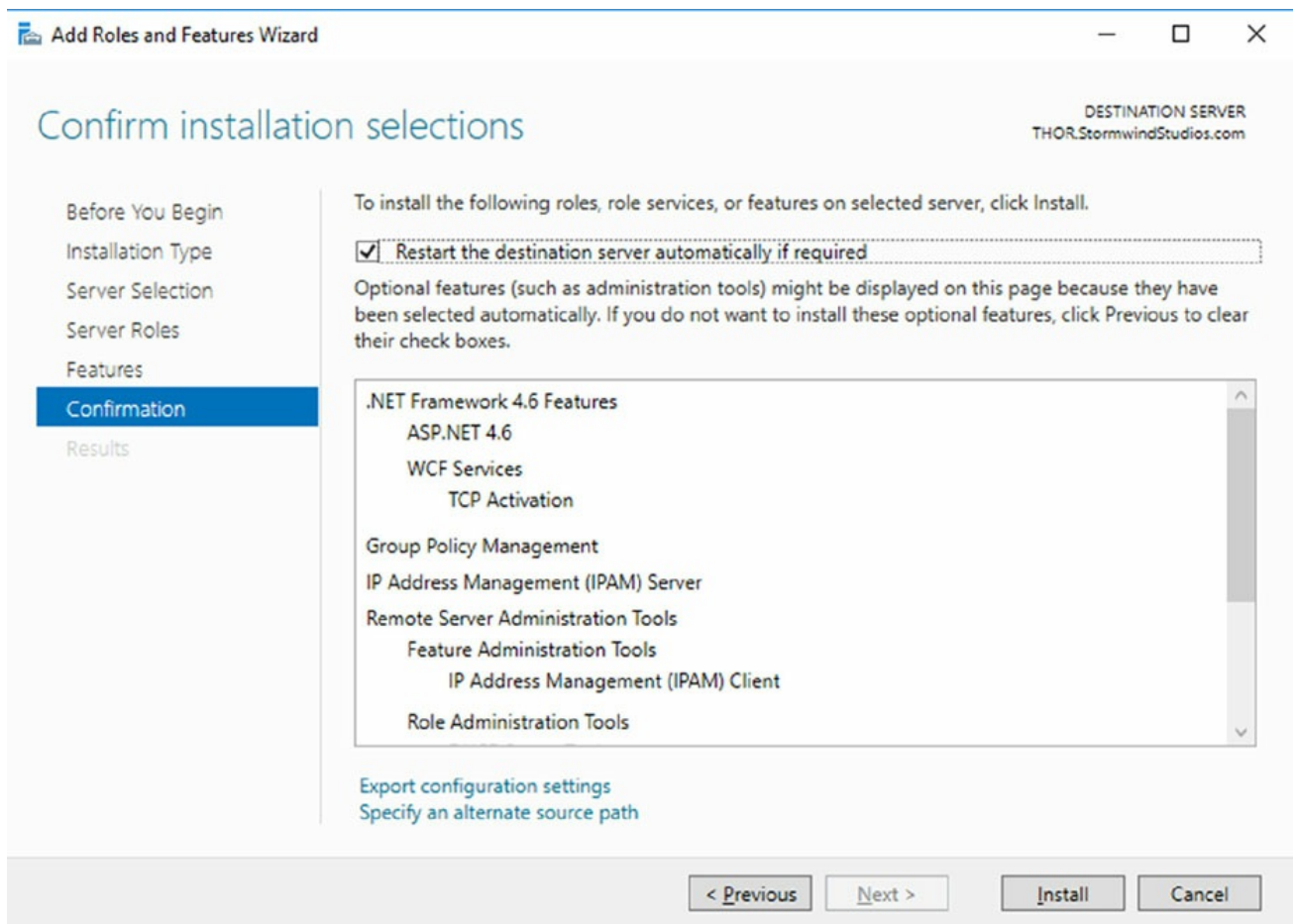
FIGURE 4.2 Confirmation Screen
