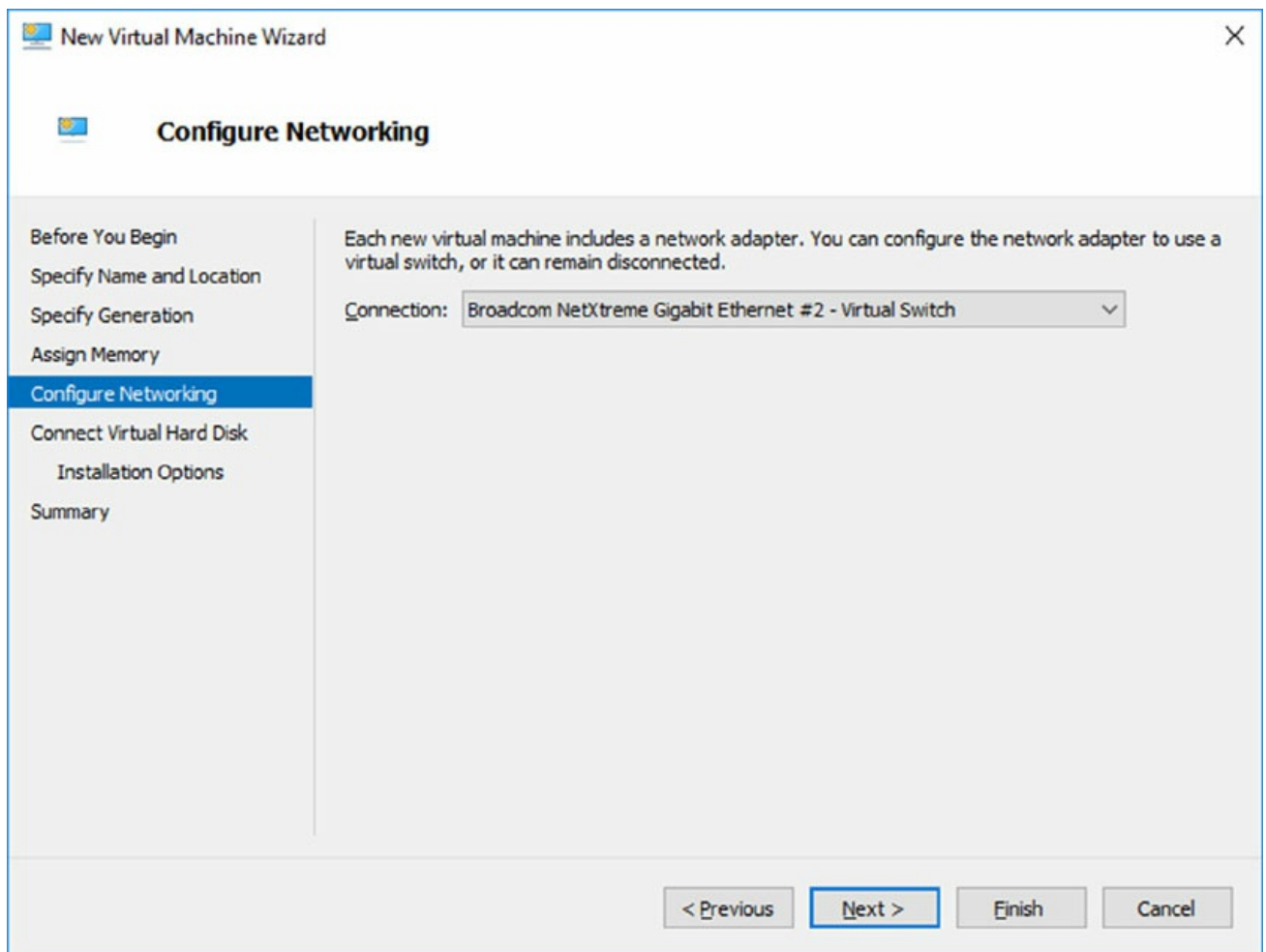
FIGURE 8.15 Networking Page
