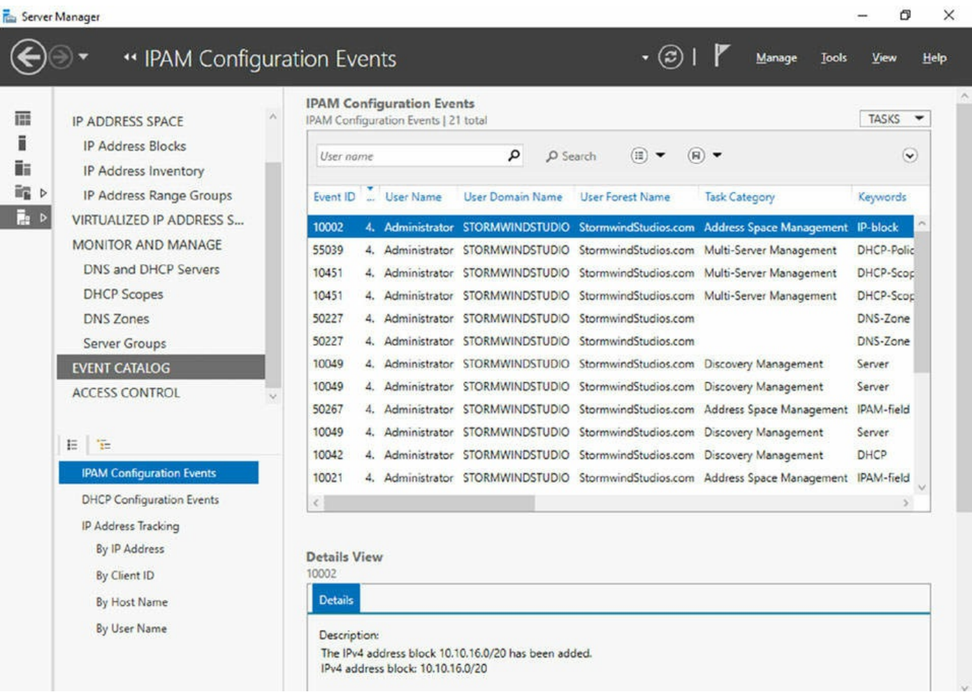
FIGURE 4.24 Event Catalog
