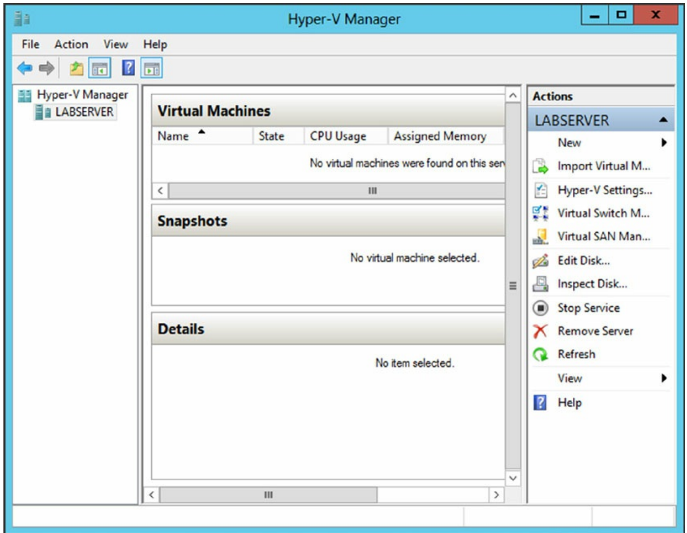
FIGURE 8.6 Hyper-V Manager
