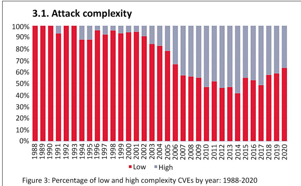
Figure 2.3: Attack complexity
