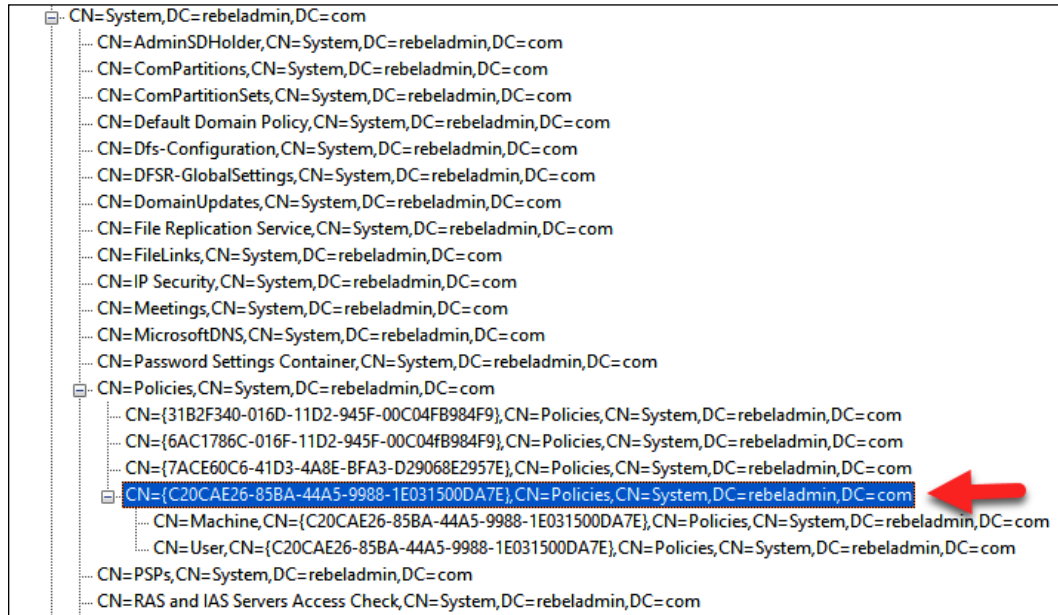
Figure 10.2: GPC information for policy
