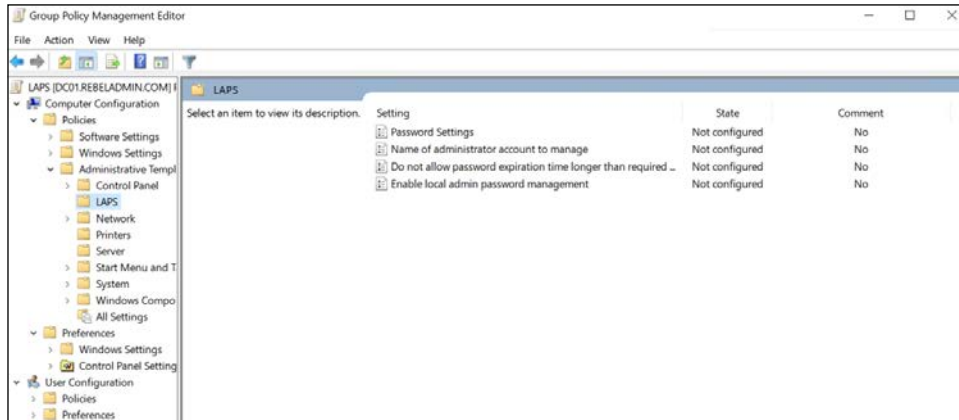
Figure 16.37: Microsoft LAPS GPO settings
