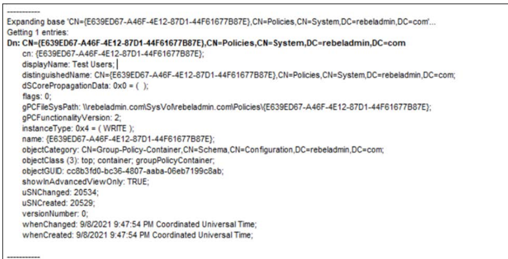
Figure 10.3: GPC information for policy – computer and user configurations
