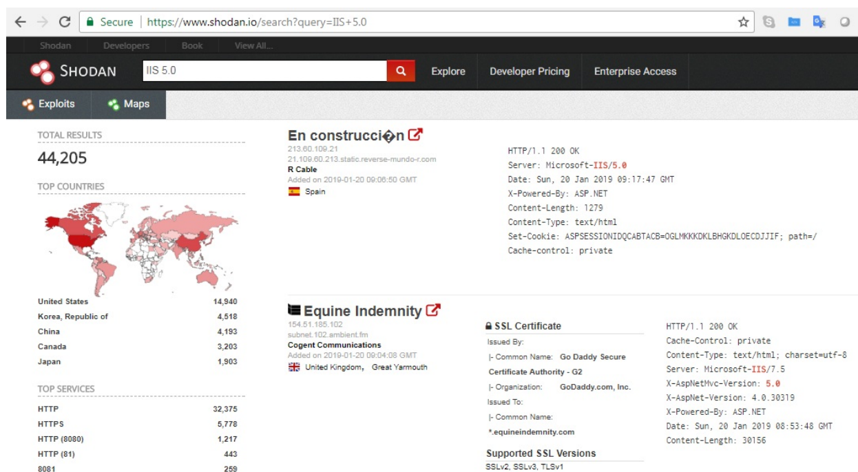
Shodan results for IIS 5.0
