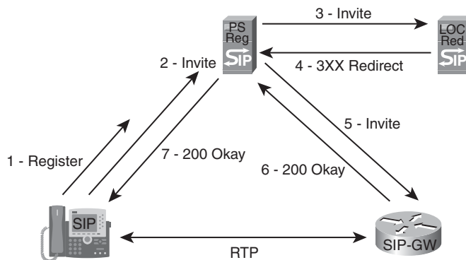
Figure 12-6 SIP Call Setup to a Gateway
