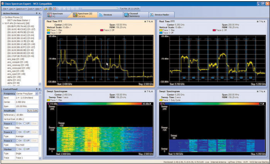
Figure 7-3 Spectrum Expert
