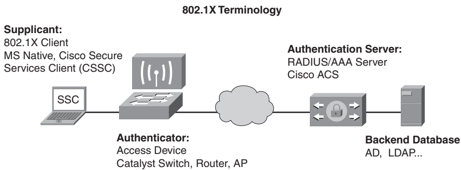
Figure 9-6 802.1x Terminology
