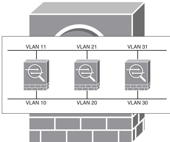
Figure 8-13 Firewall Multiple-Context Mode
