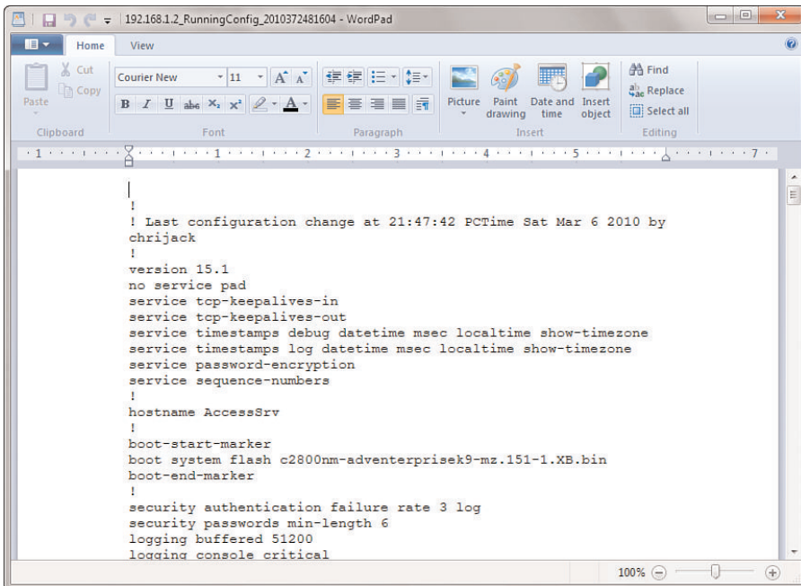
Figure 7-5 SNMP Configuration File Download Through Cain
