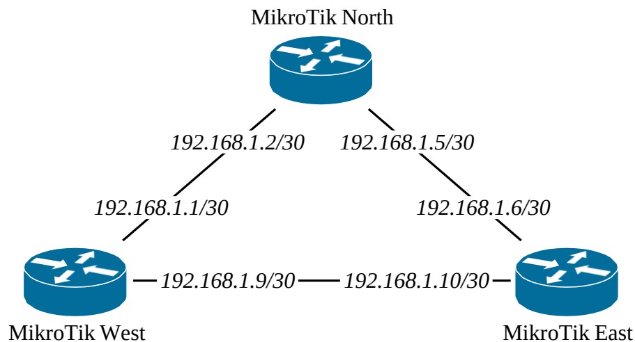
Figure 8.6: /30 Point-to-Point Addressing
