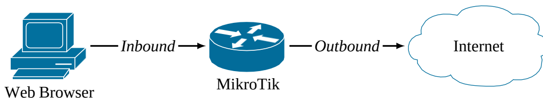
Figure 12.4: Forward Chain Traffic
