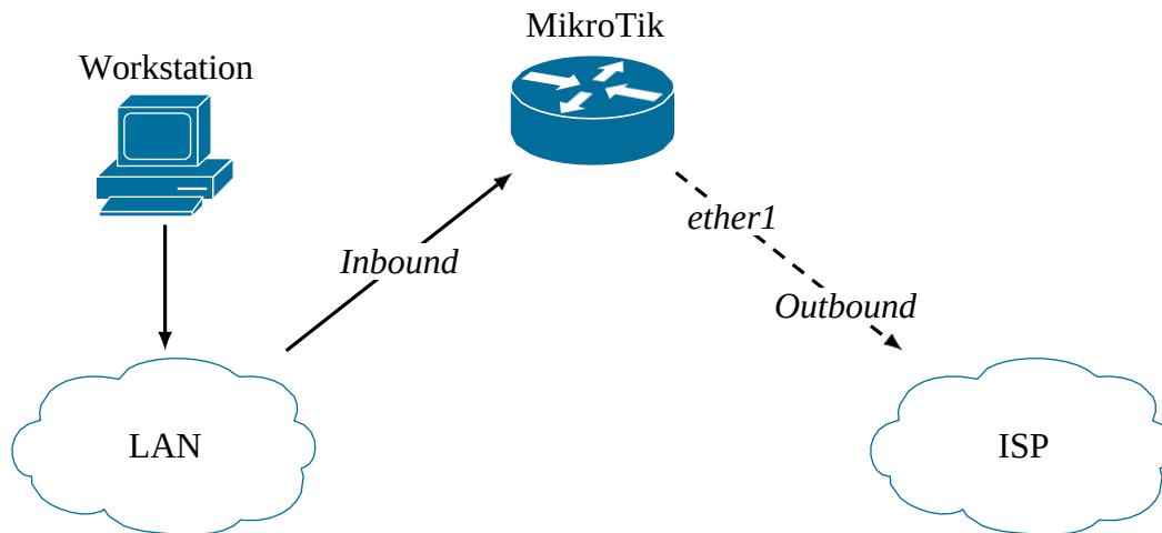
Figure 13.1: Source NAT Topology
