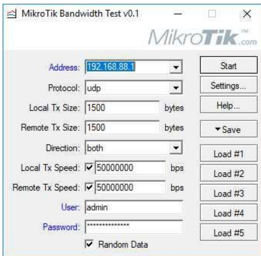
Figure 16.28: Windows Bandwidth Test Tool
