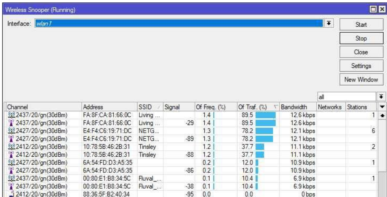
Figure 14.15: Winbox Wireless Snooper
