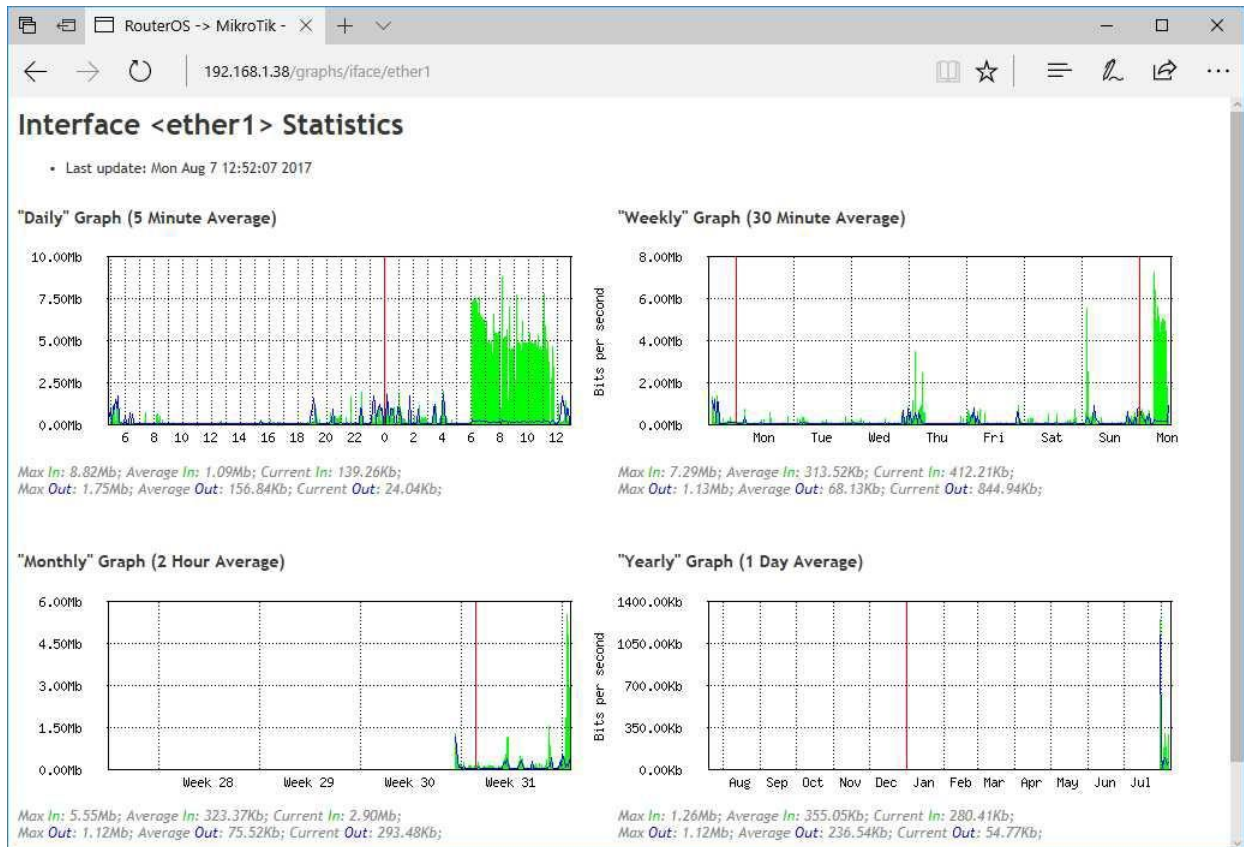
Figure 17.2: Web Console Interface Graph
