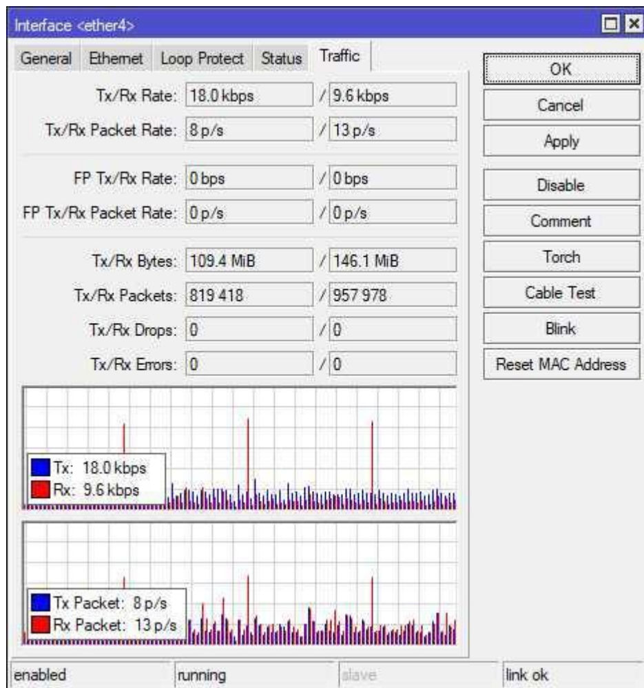
Figure 17.7: Interface Traffic Statistics
