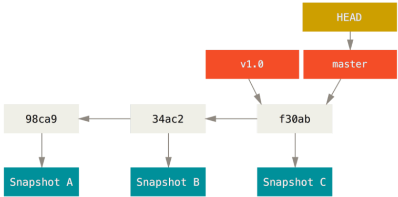
FIGURE 3-3 A branch and its commit history
