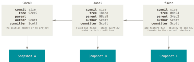
FIGURE 3-2 Commits and their parents
