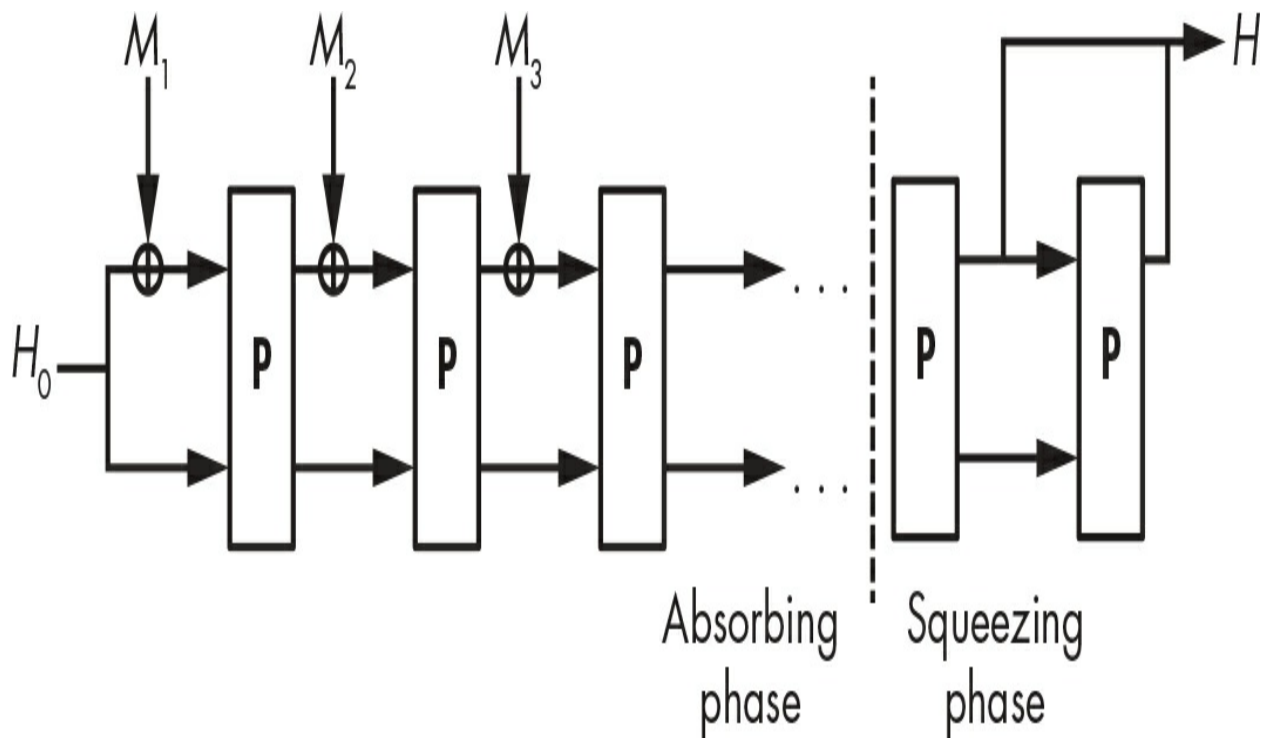
Figure 6-7: The sponge construction
