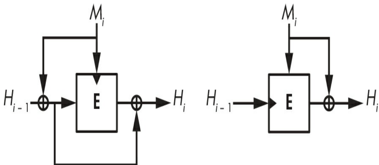
Figure 6-6: Other secure block cipher–based compression function constructions
