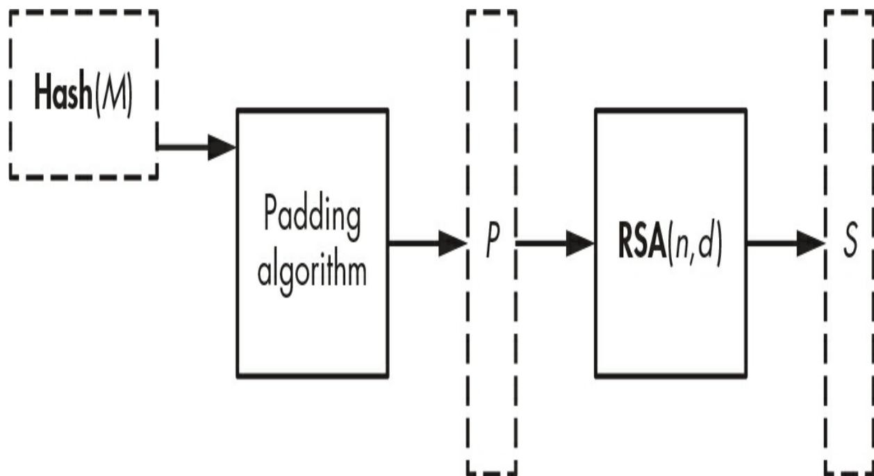
Figure 10-3: Signing a message, M , with RSA and with the PSS standard, where (n, d) is the
