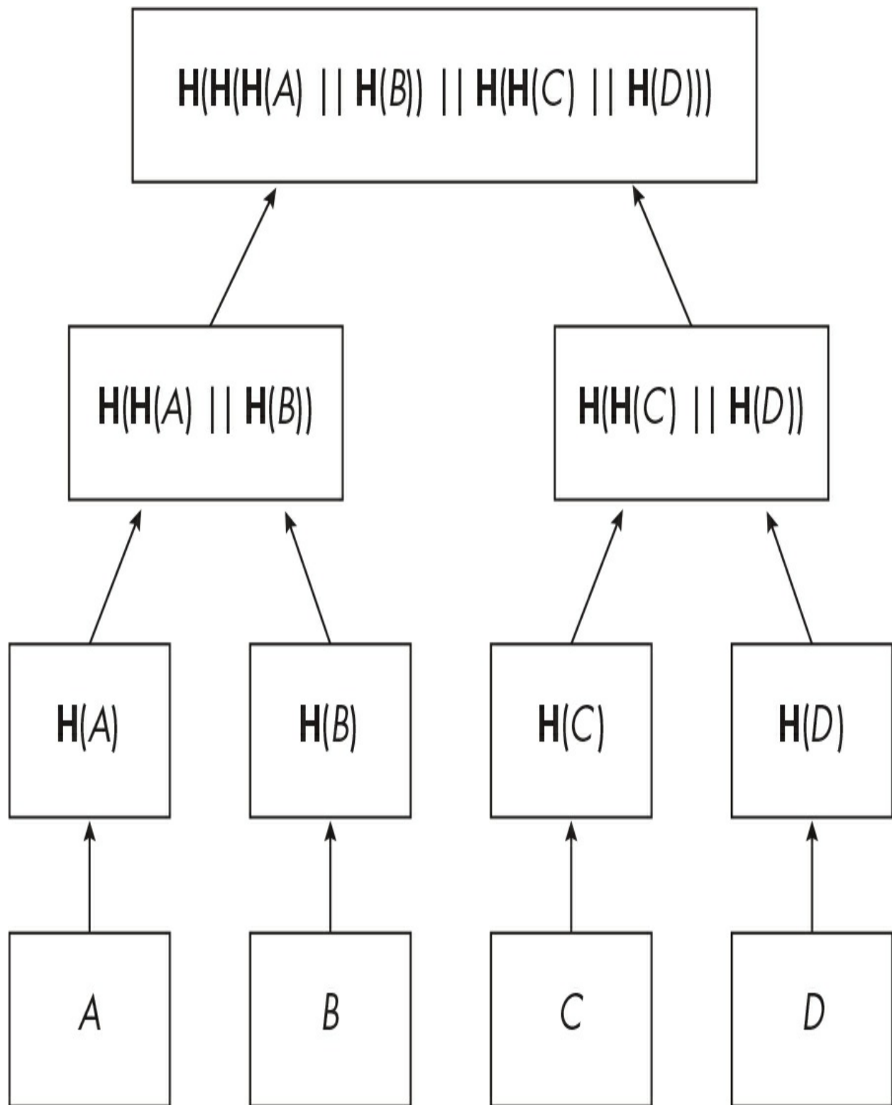
Figure 15-1: A hash tree, where the leaves are the input and the root is the output
