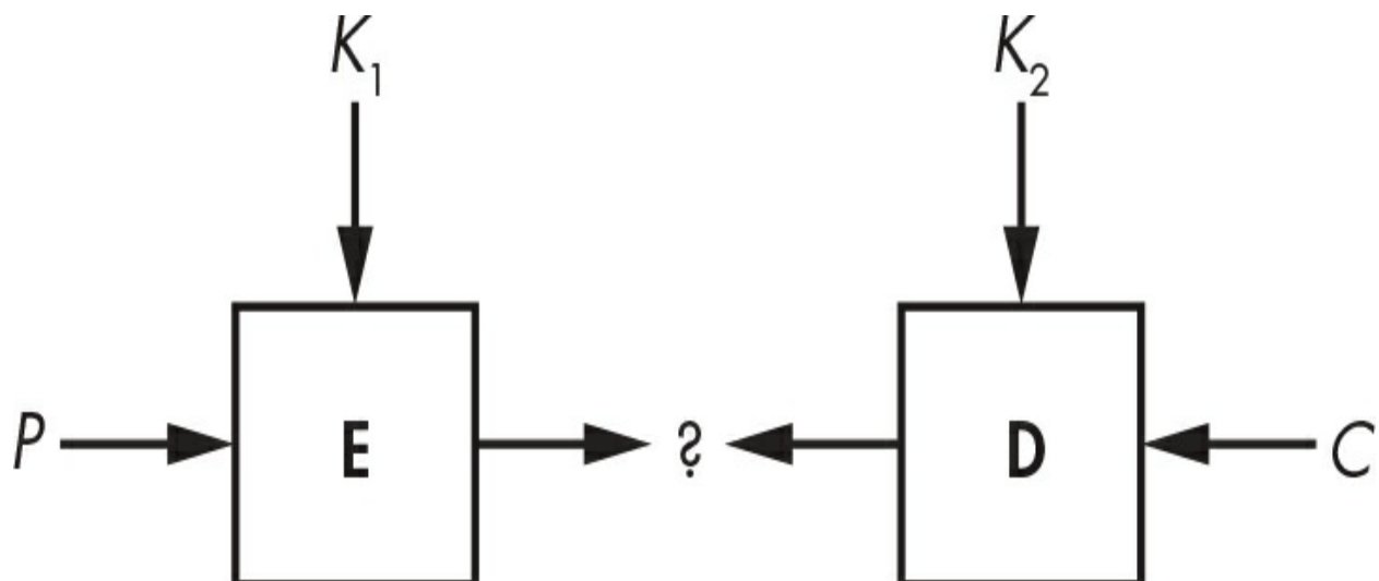
Figure 4-12: The MitM attack
