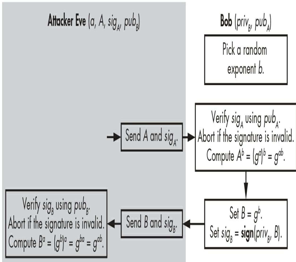
Figure 11-5: An impersonation attack on the authenticated Diffie–Hellman protocol
