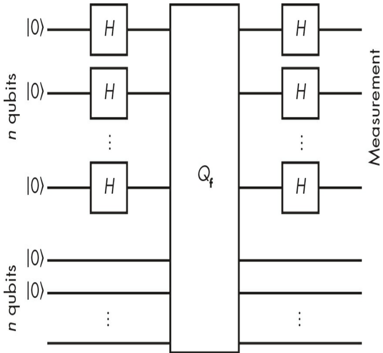
Figure 14-4: The circuit of the quantum algorithm that solves Simon's problem efficiently
