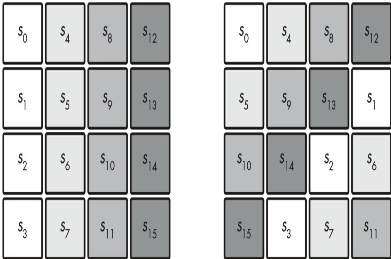
Figure 4-5: ShiftRows rotates bytes within each row of the internal state.
