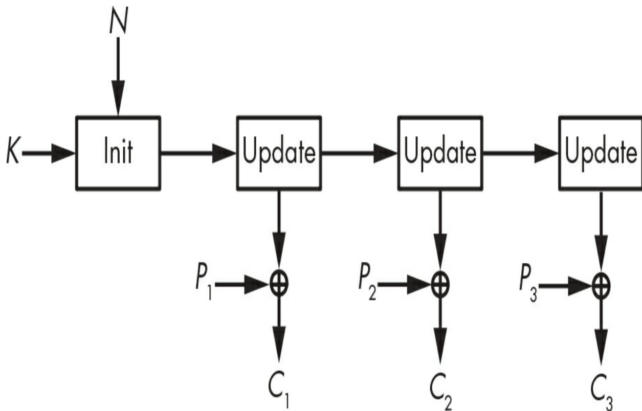
Figure 5-2: A stateful stream cipher
