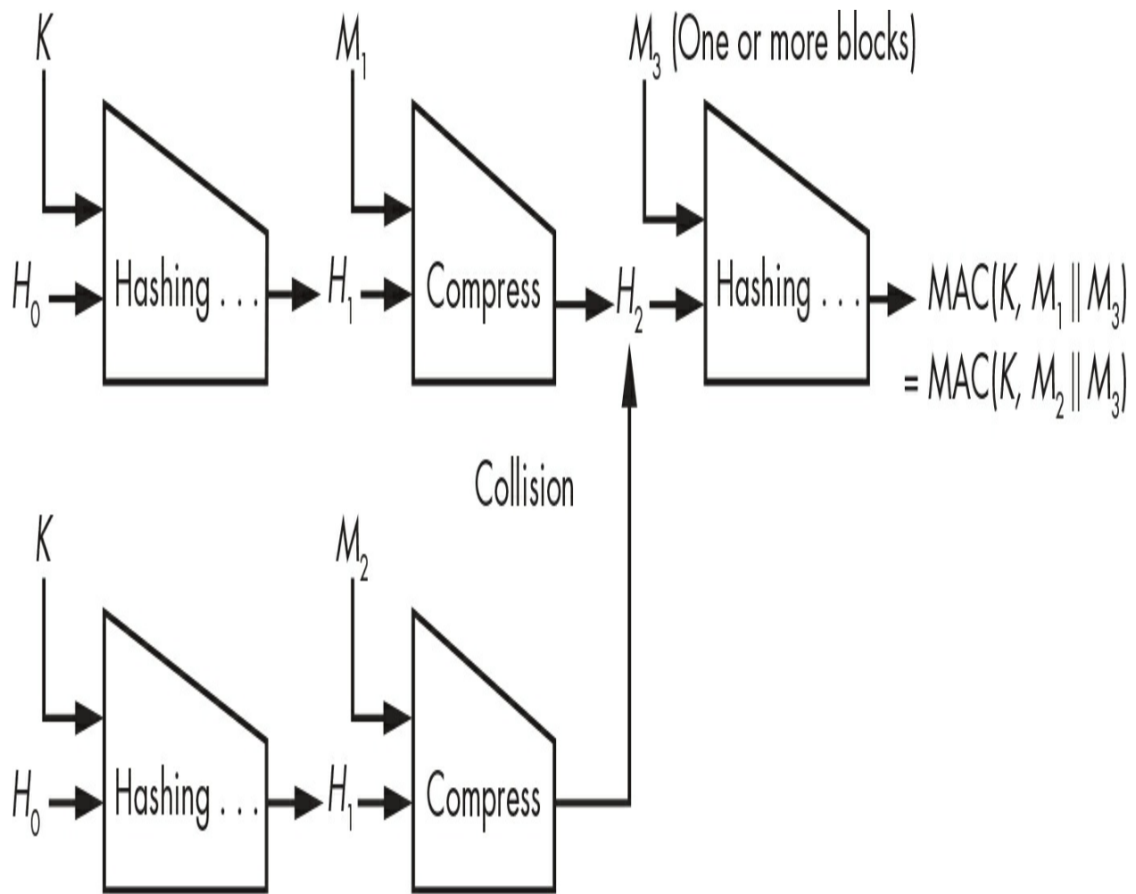
Figure 7-2: The principle of the generic forgery attack on hash-based MACs
