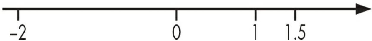
Figure 14-1: A view of real numbers as points on an infinite straight line
