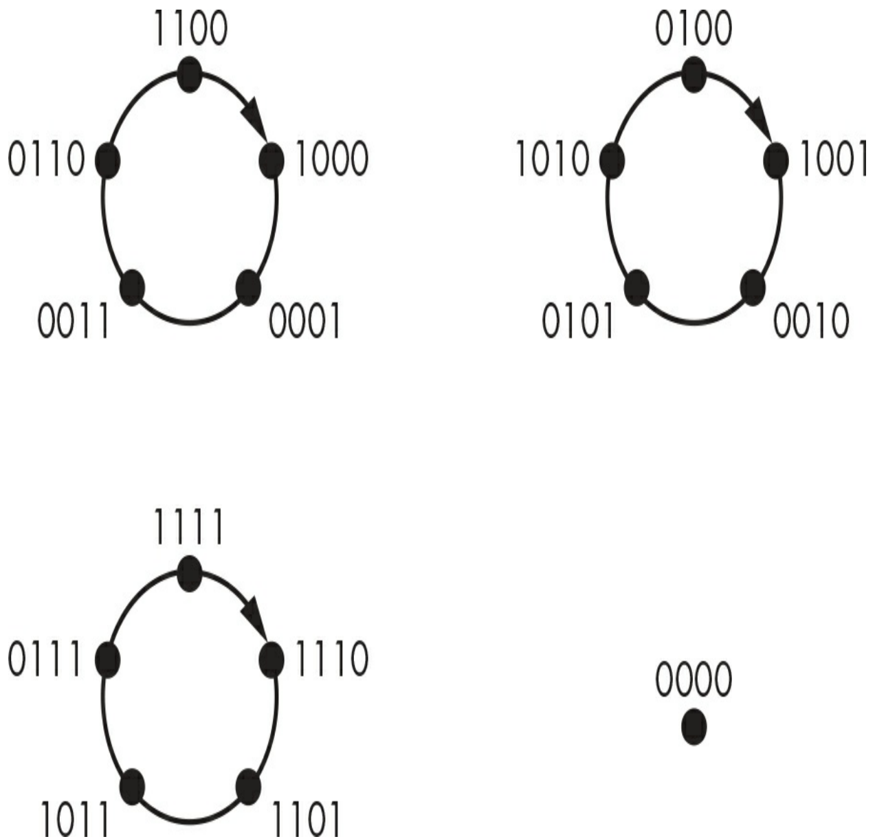
Figure 5-4: Cycles of the FSR whose feedback function XORs the 4 bits together
