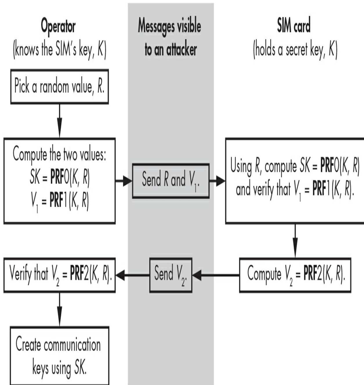
Figure 11-1: The AKA protocol in 4G and 5G telecommunication
