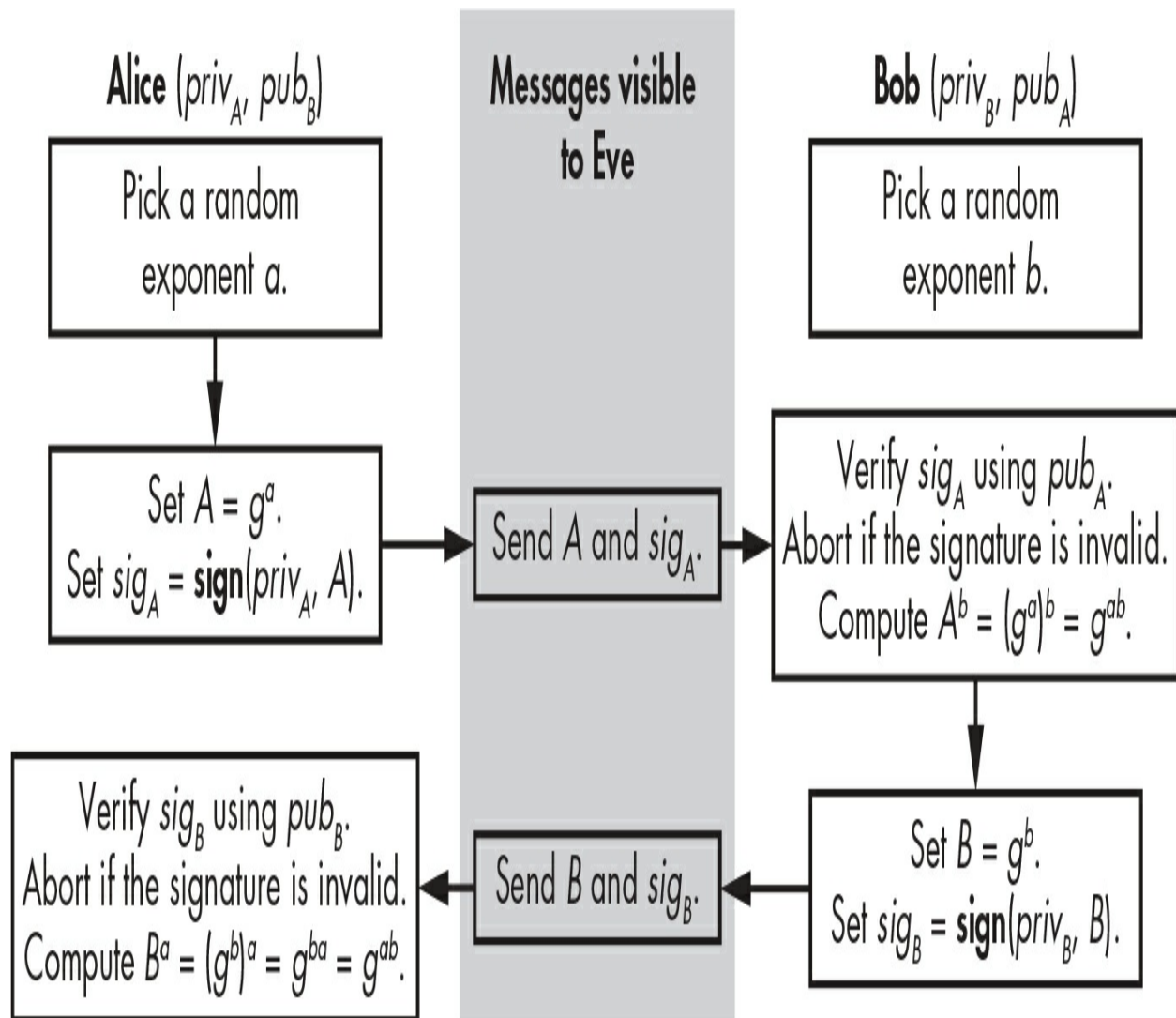
Figure 11-4: The authenticated Diffie–Hellman protocol
