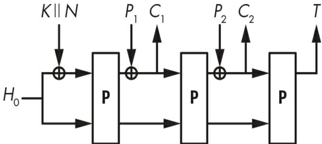
Figure 8-4: A permutation-based authenticated cipher
