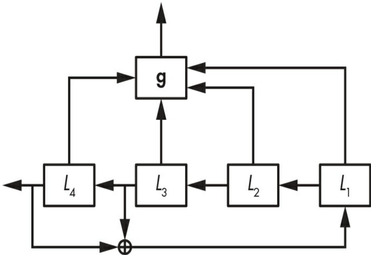
Figure 5-7: A filtered LFSR
