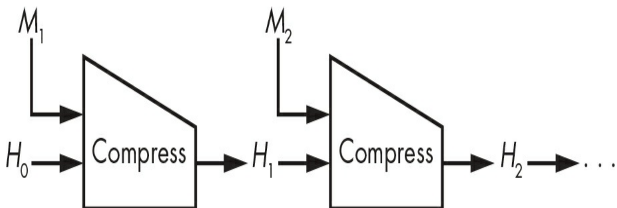
Figure 6-4: The Merkle–Damgård construction using a compression function called Compress
