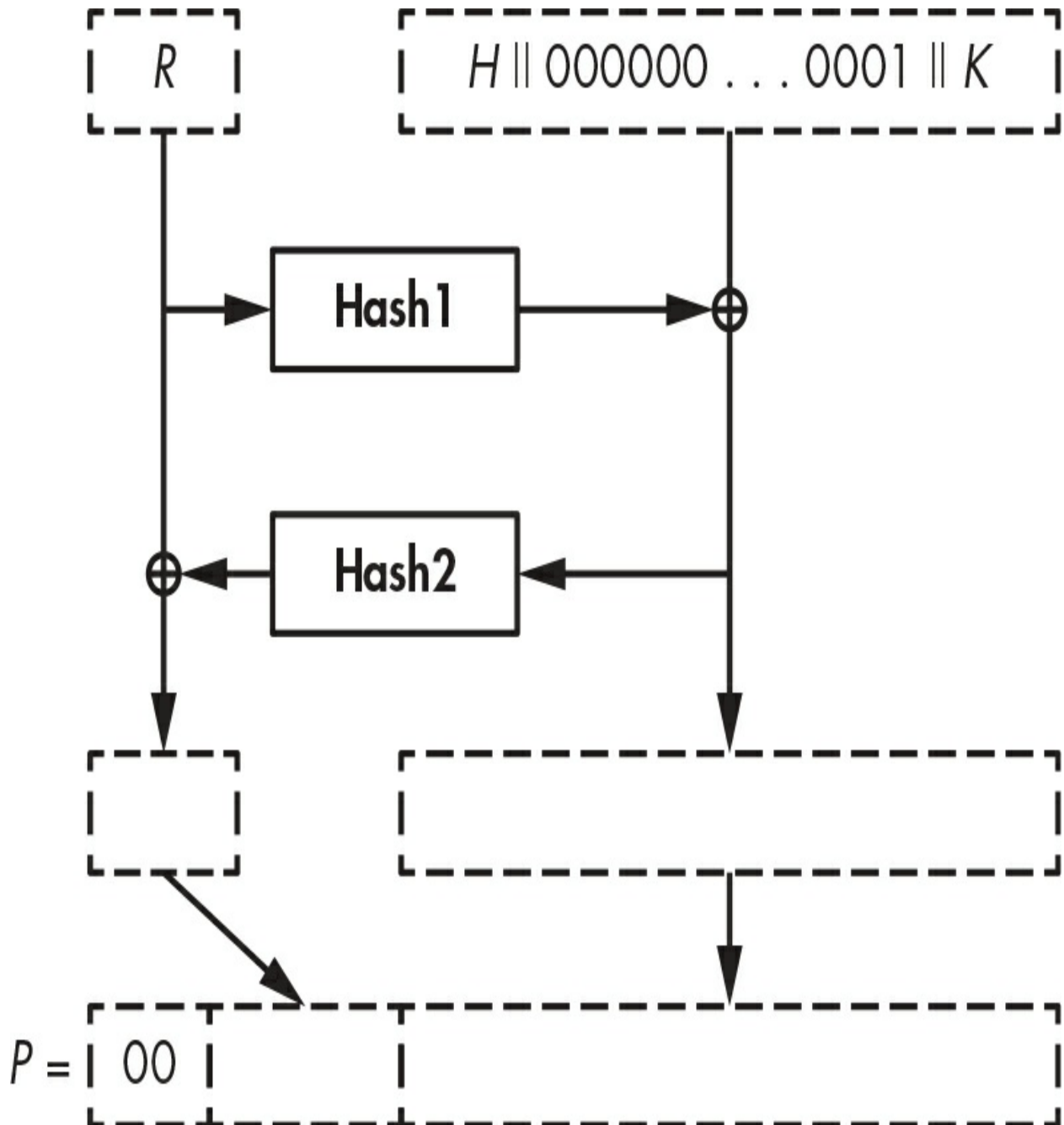
Figure 10-2: Encrypting a symmetric key, K , with RSA-OAEP, where H is a fixed parameter and R is random bits
