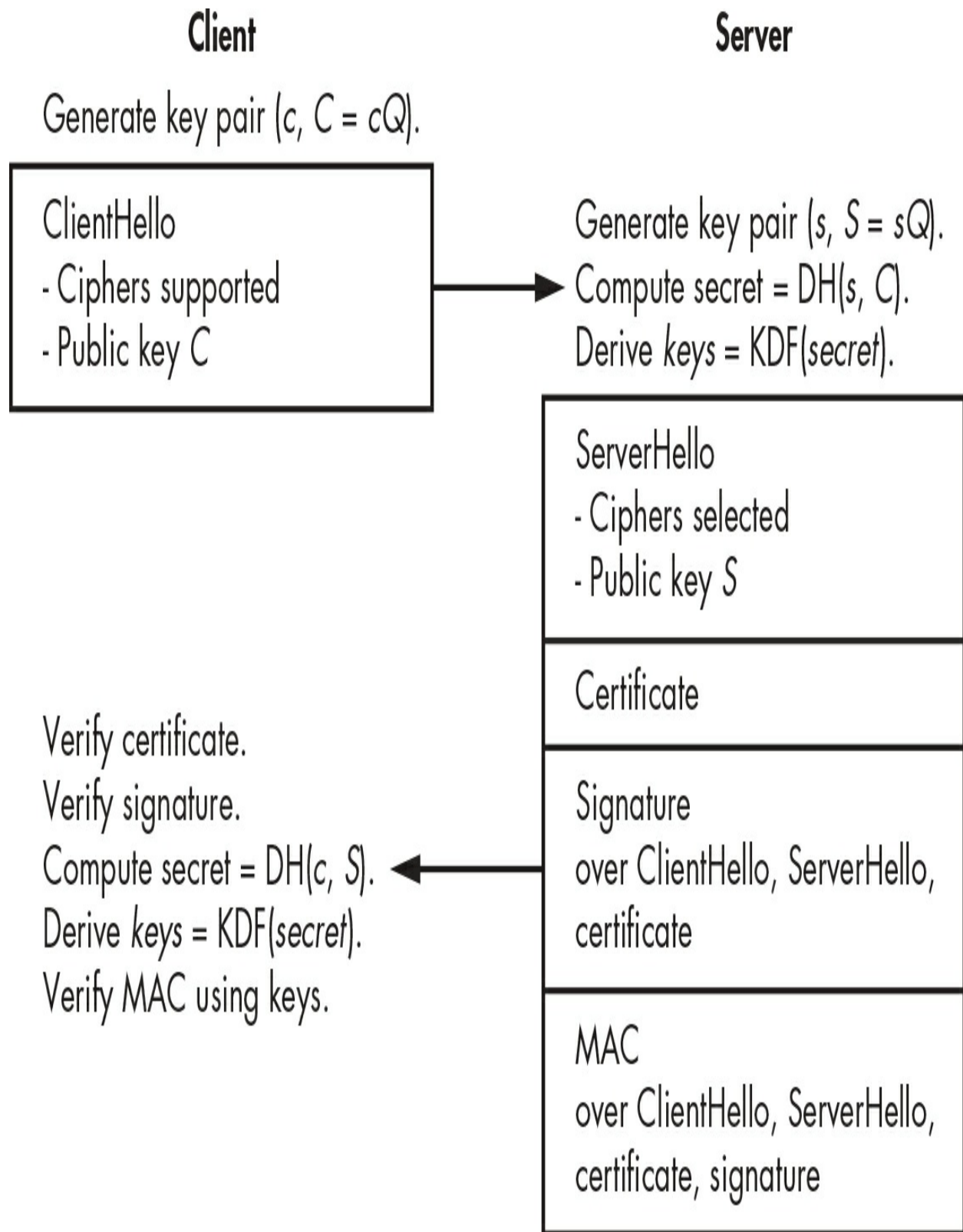
Figure 13-1: The TLS 1.3 handshake process
