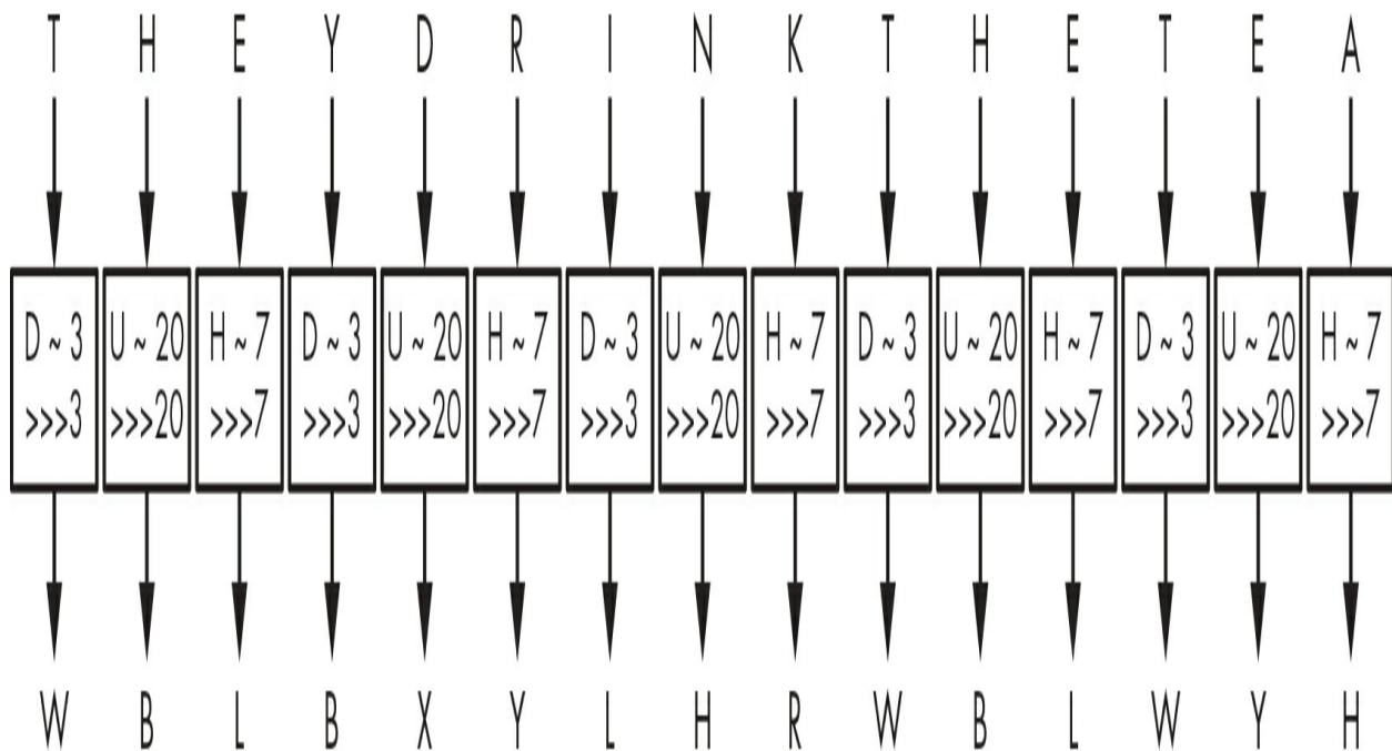
Figure 1-3: The Vigenère cipher
