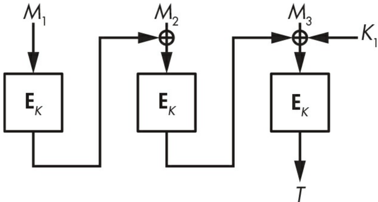
Figure 7-3: The CMAC block cipher-based MAC construction when the message is a sequence of integral blocks
