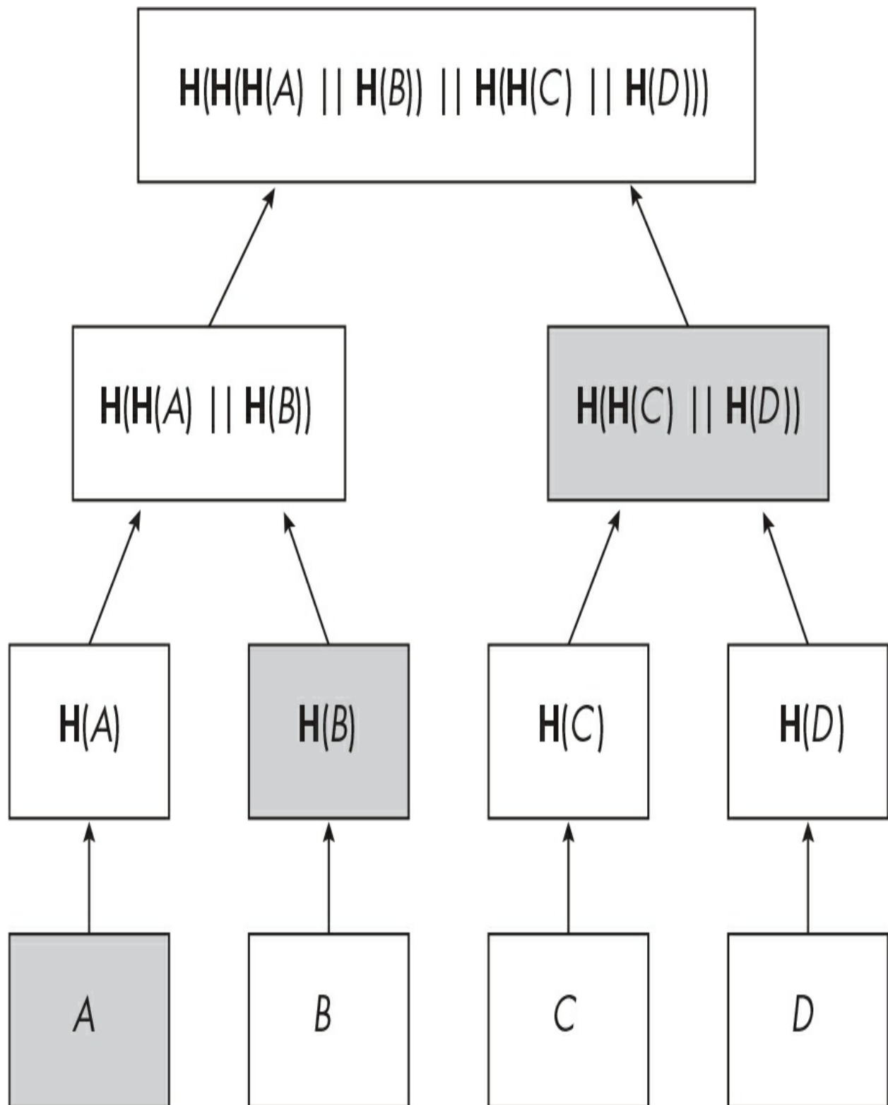
Figure 15-2: A Merkle tree, wherein the shaded cells constitute the membership path of A
