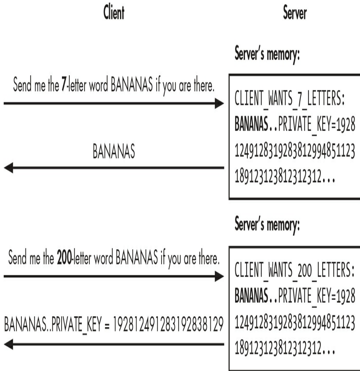
Figure 13-3: The Heartbleed bug in OpenSSL implementations of TLS
