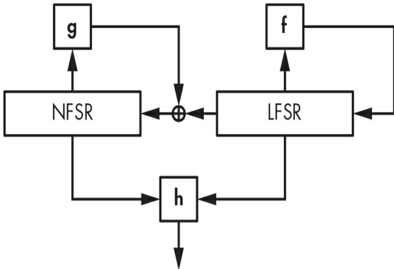
Figure 5-8: The mechanism of Grain-128a, with a 128-bit NFSR and a 128-bit LFSR
