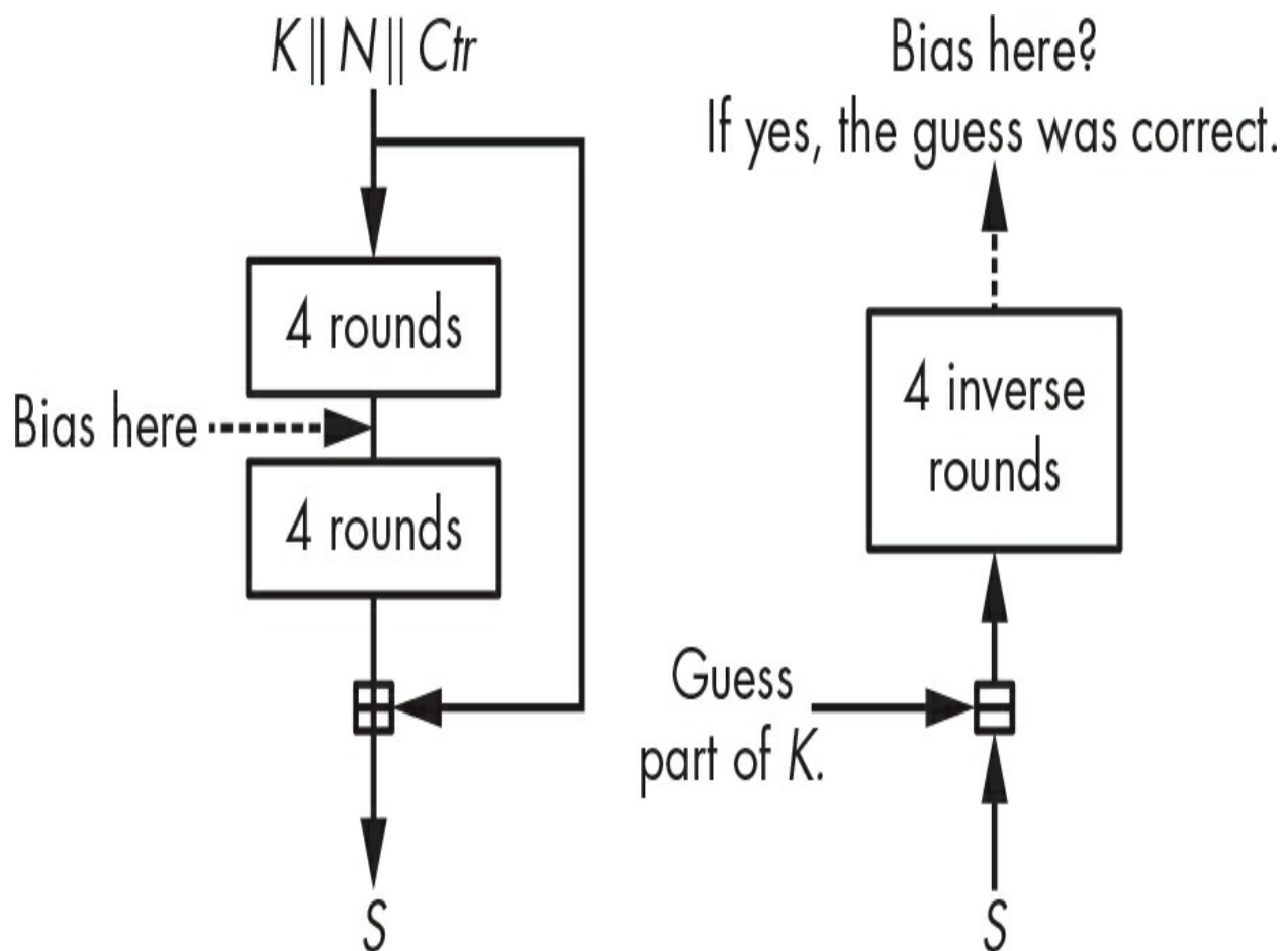
Figure 5-13: The principle of the attack on Salsa20/8
