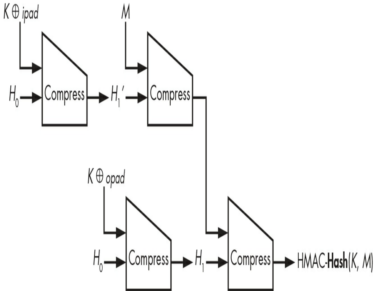
Figure 7-1: The HMAC hash-based MAC construction for a hash function based on a compression function
