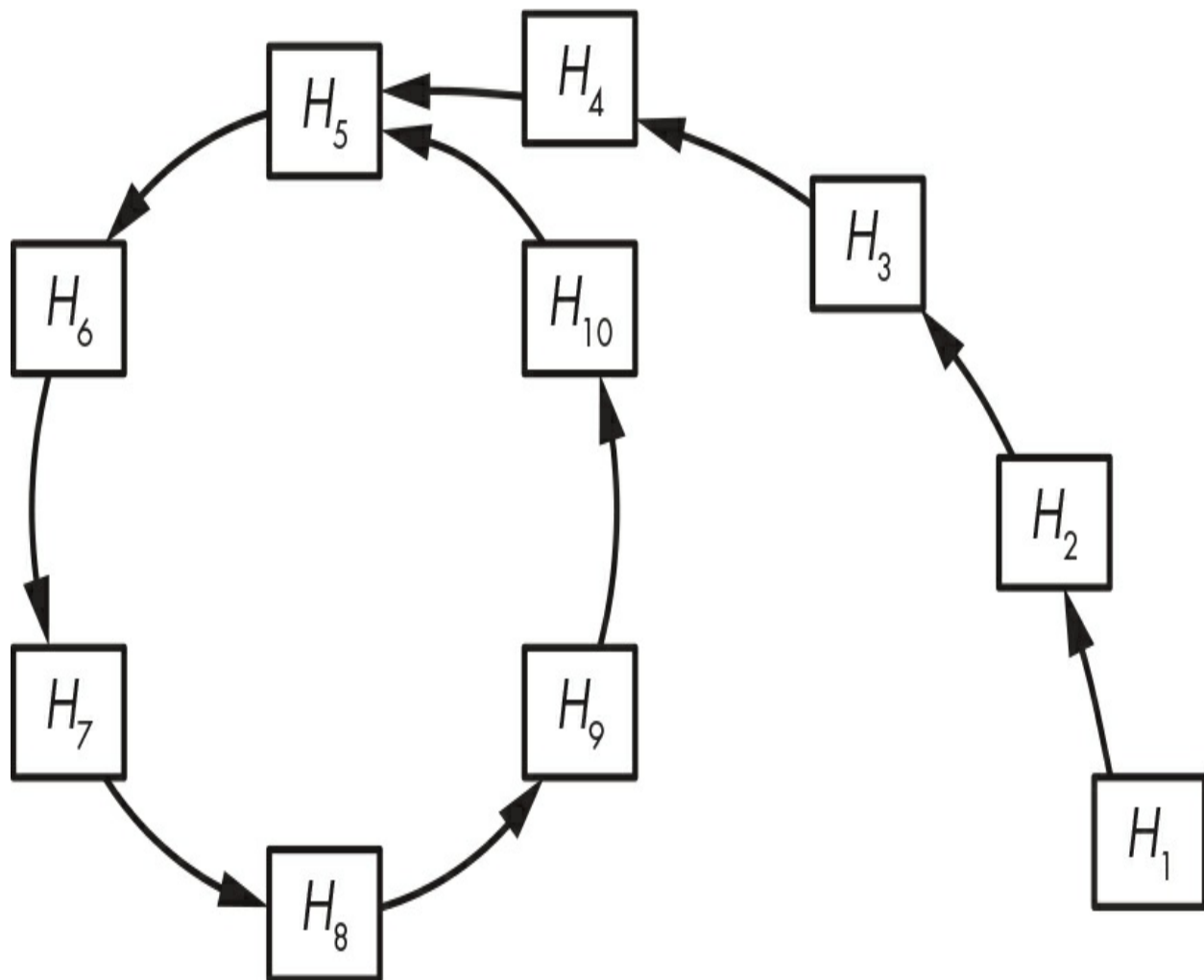
Figure 6-3: The structure of the Rho hash function, where each arrow represents an evaluation of the hash function. The cycle beginning at H_5 corresponds to a collision, \text{Hash}(H_4) = \text{Hash}(H_{10}) = H_5 .
