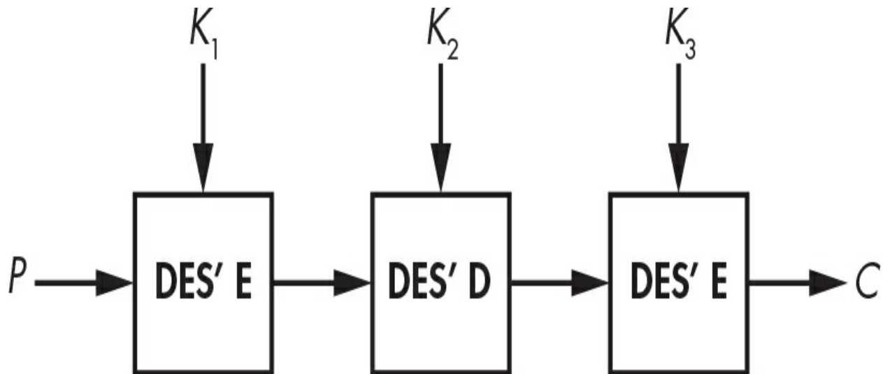
Figure 4-11: The 3DES block cipher construction
