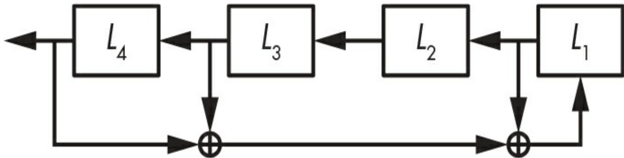
Figure 5-5: An LFSR with the feedback polynomial 1 + X + X^3 + X^4
