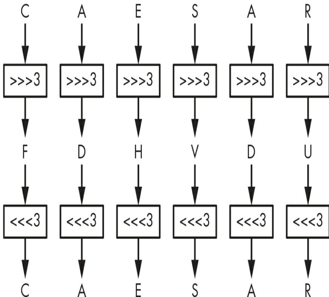
Figure 1-2: The Caesar cipher
