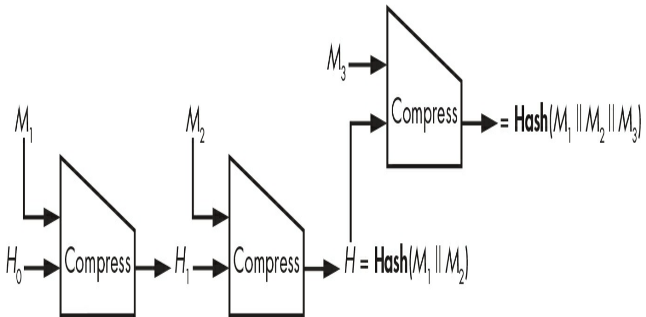
Figure 6-9: The length-extension attack
