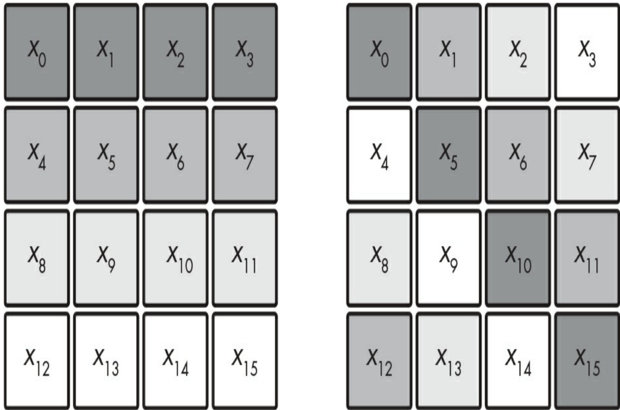
Figure 5-12: Columns and rows transformed by Salsa20's quarter-round ( QR ) function
