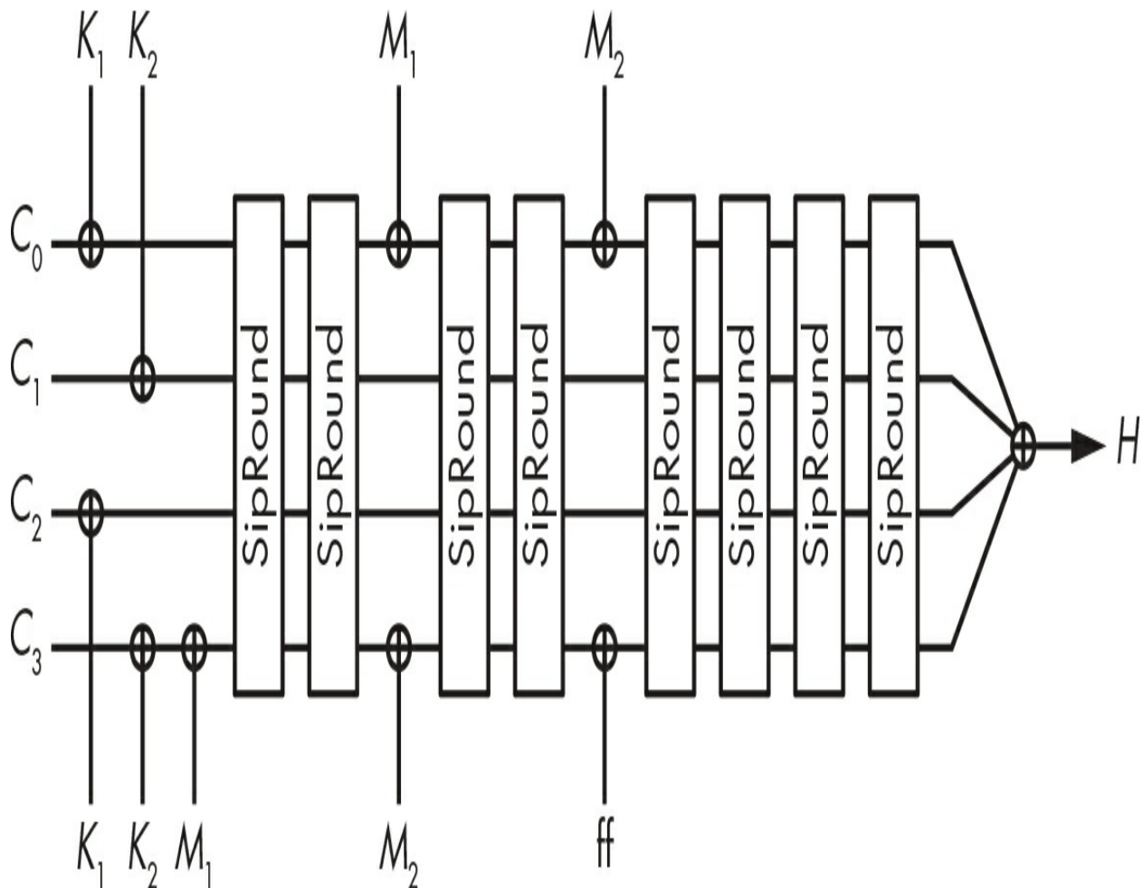
Figure 7-5: SipHash-2-4 processing a 15-byte message (a block, M_1 , of 8 bytes and a block, M_2 , of 7 bytes, plus 1 byte of padding)
