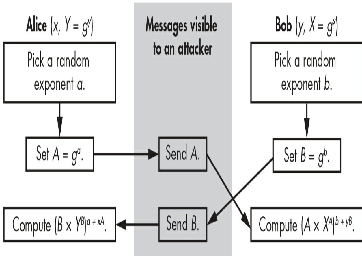
Figure 11-6: The MQV protocol
