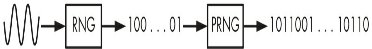
Figure 2-1: RNGs produce few unreliable bits from analog sources, whereas PRNGs expand those bits to a long stream of reliable bits.
