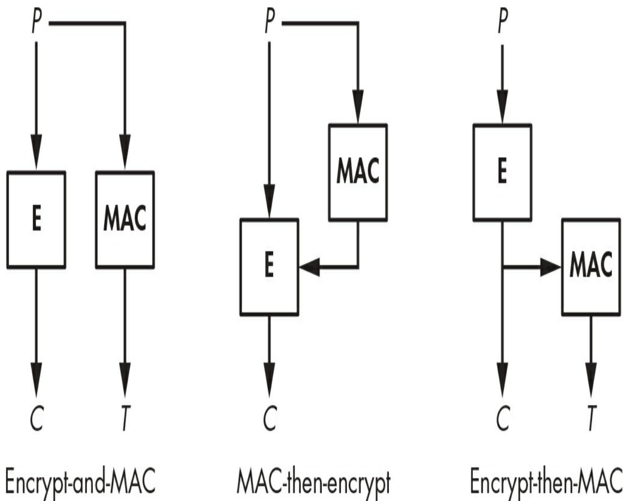
Figure 8-1: Cipher and MAC combinations
