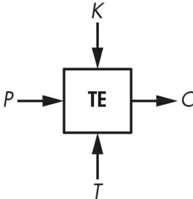
Figure 1-6: Tweakable encryption
