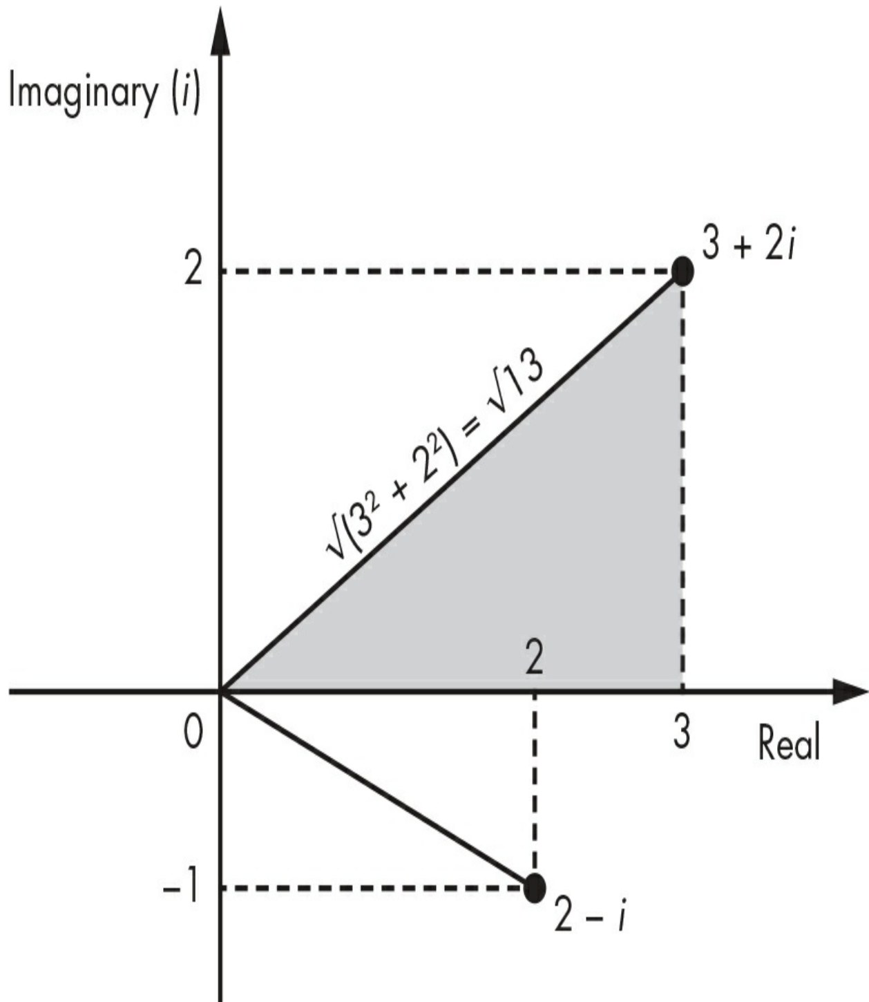
Figure 14-2: A view of complex numbers as points in a two-dimensional space
