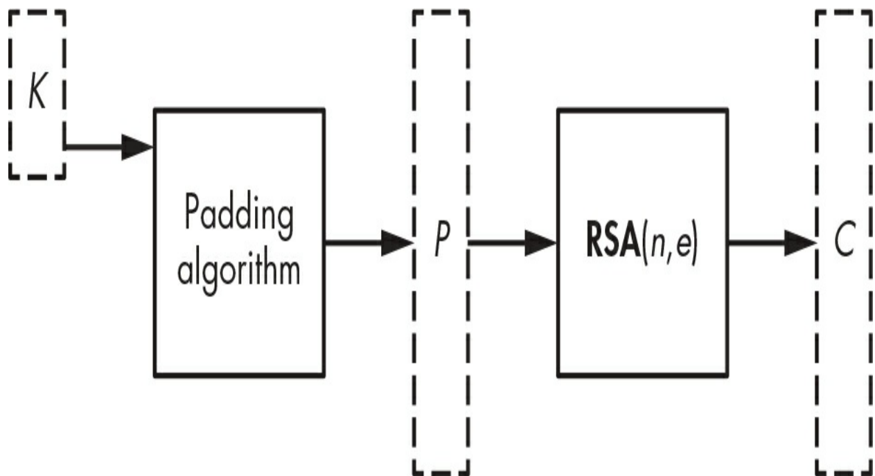
Figure 10-1: Encrypting a symmetric key, K , with RSA using (n, e) as a public key
