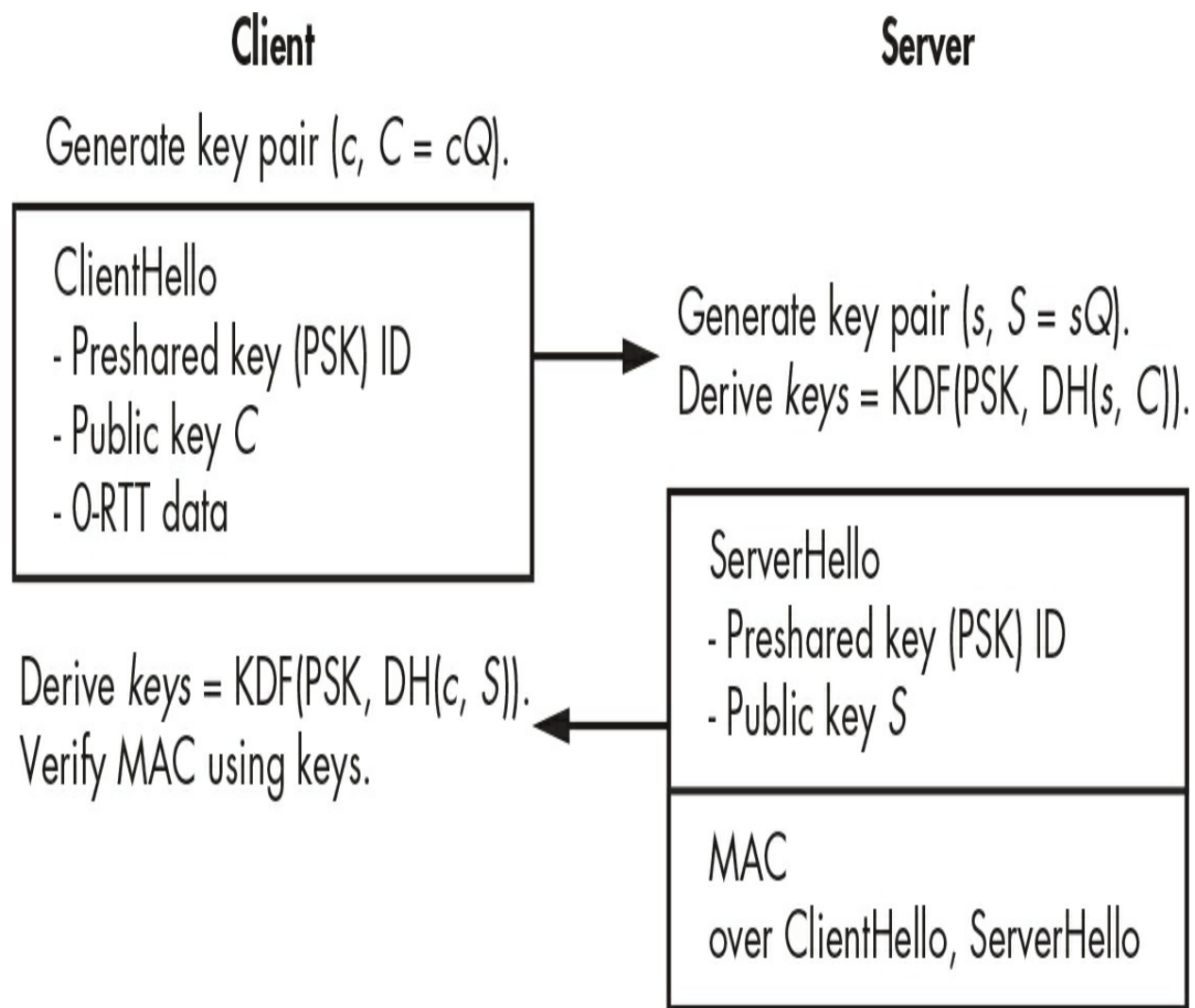
Figure 13-2: The TLS 1.3 session resumption handshake, wherein the 0-RTT data is the session resumption data sent along with the ClientHello
