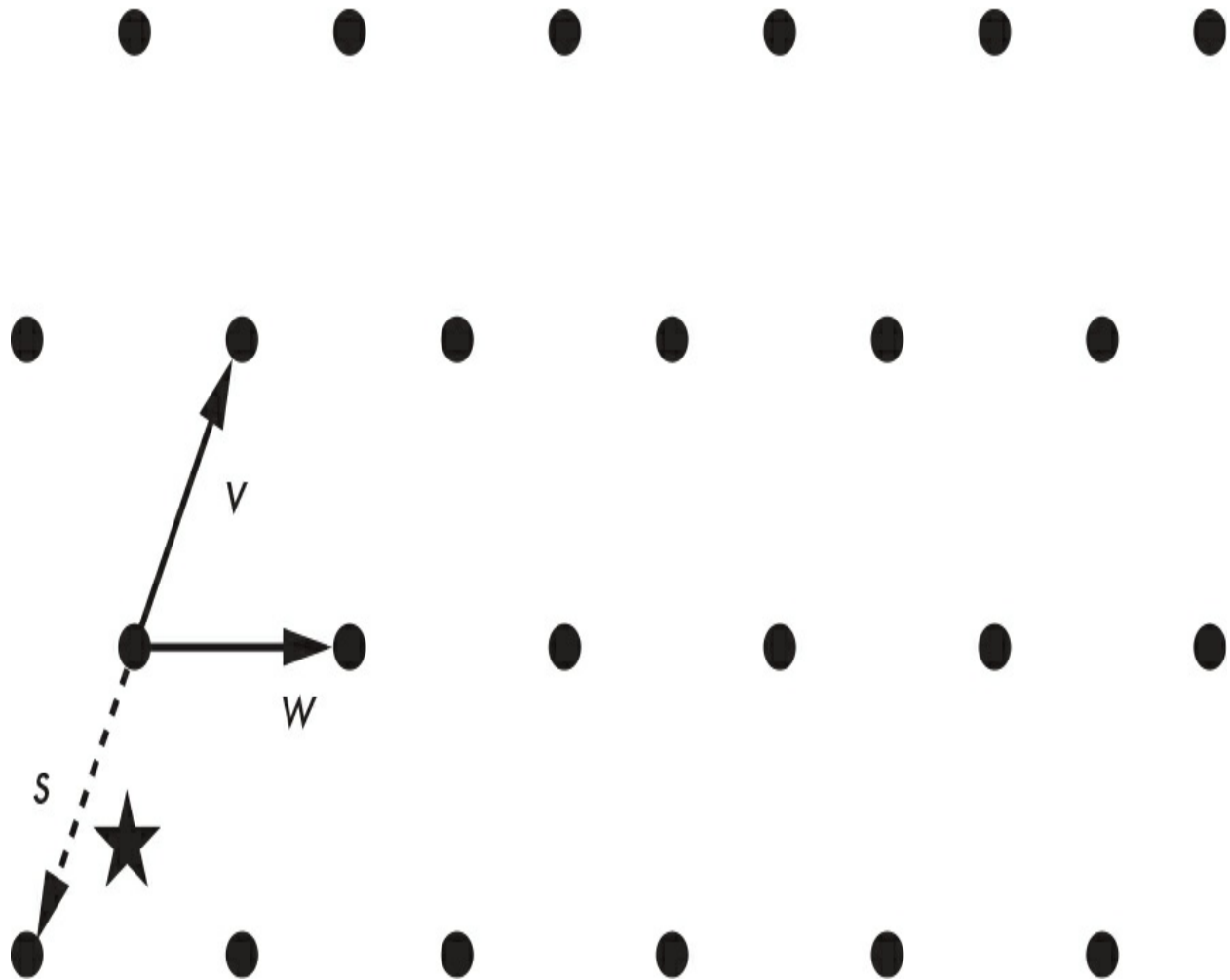
Figure 14-5: Points of a two-dimensional lattice, where v and w are basis vectors of the lattice and s is the closest vector to the star-shaped point
