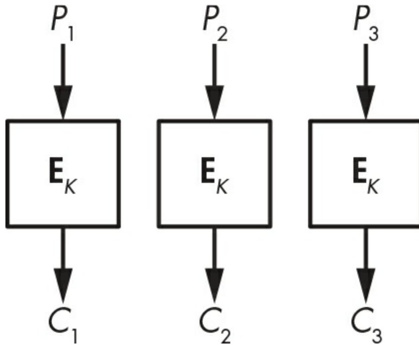
Figure 4-6: ECB mode
