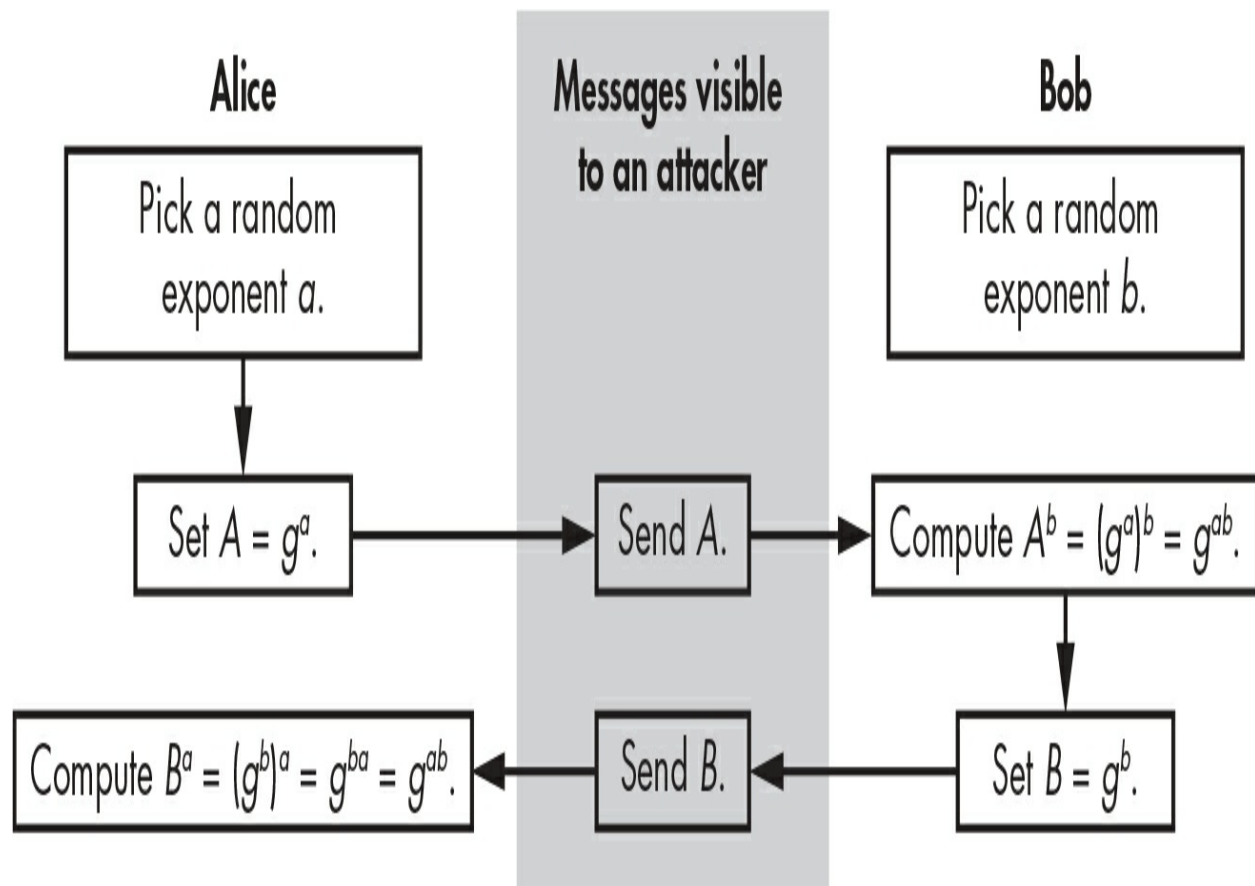
Figure 11-2: The anonymous Diffie–Hellman protocol
