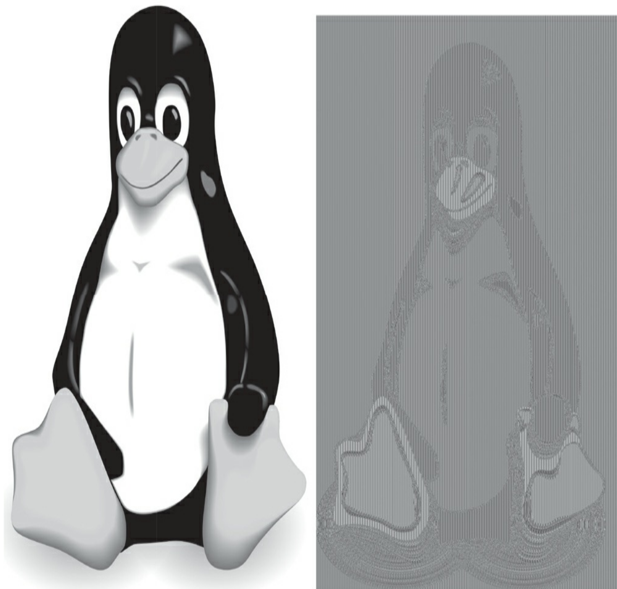
Figure 4-7: The original image (left) and the ECB-encrypted image (right)
