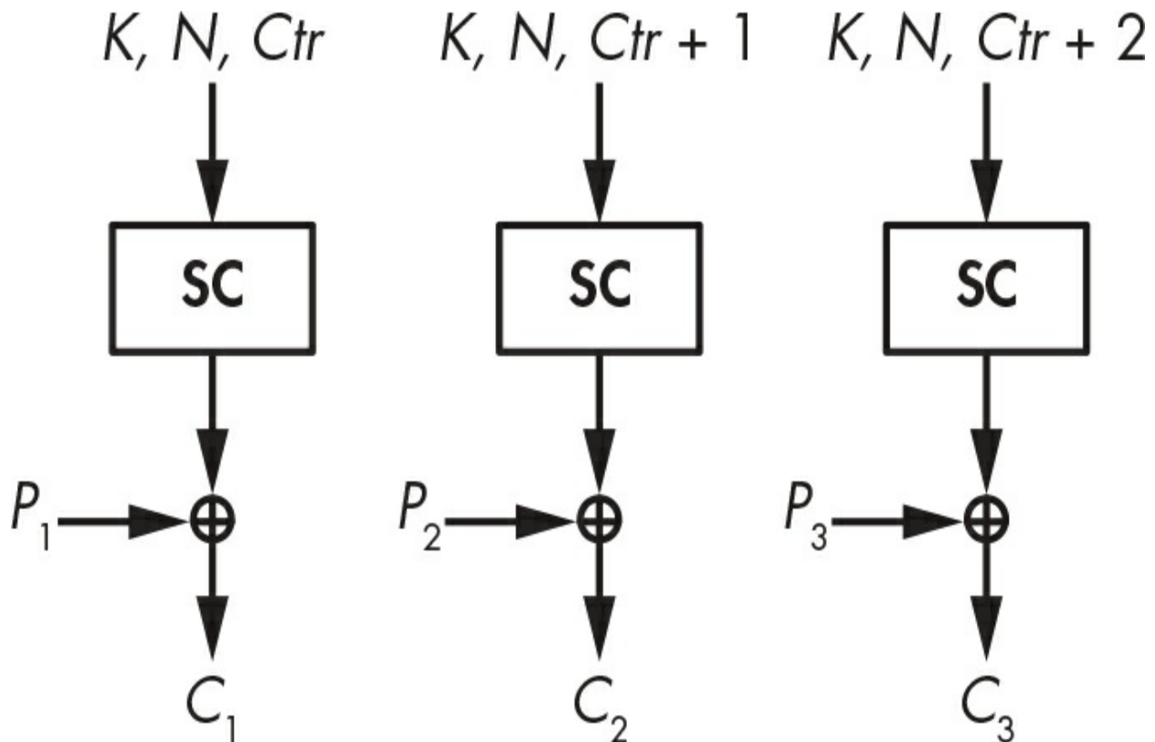
Figure 5-3: A counter-based stream cipher
