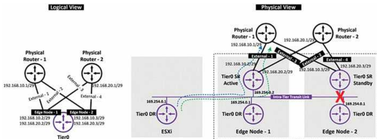
Figure 5.42: Tier0 gateway configured in Active-Standby HA mode
