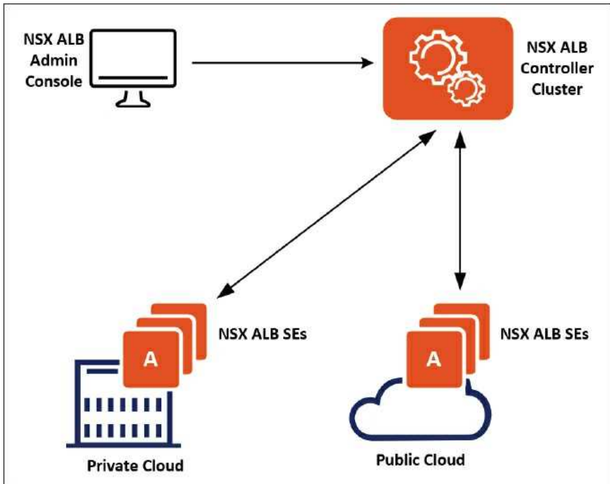
Figure 12.2: Core Components of NSX ALB environment
