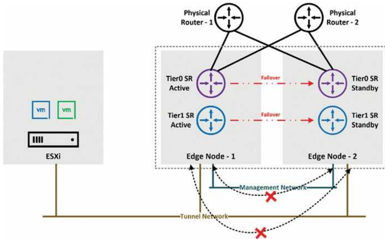
Figure 5.44: Failover trigger with BFD
