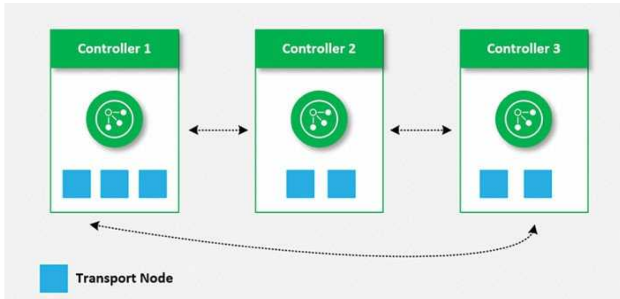
Figure 1.9: Controller Sharding
