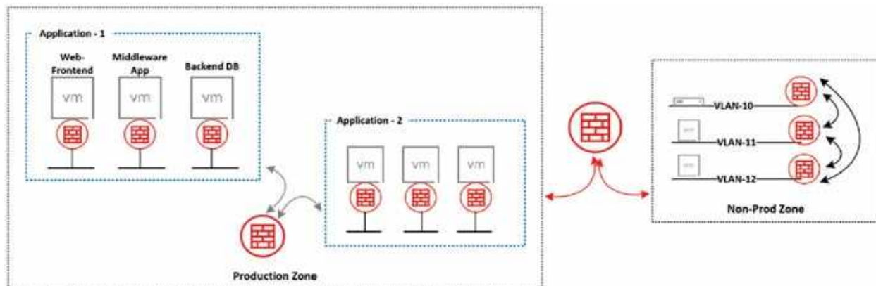
Figure 8.1: Security segmentation
