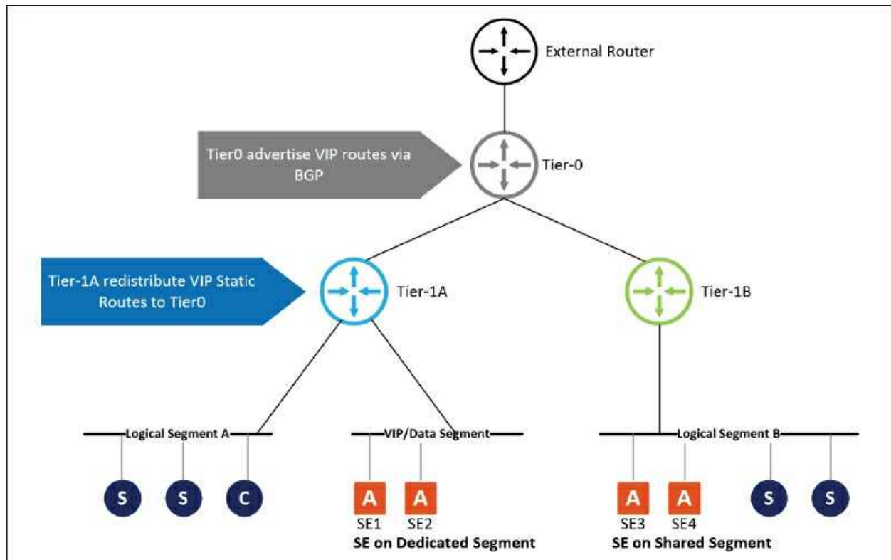
Figure 12.4: NSX ALB Supported Topologies in NSX
