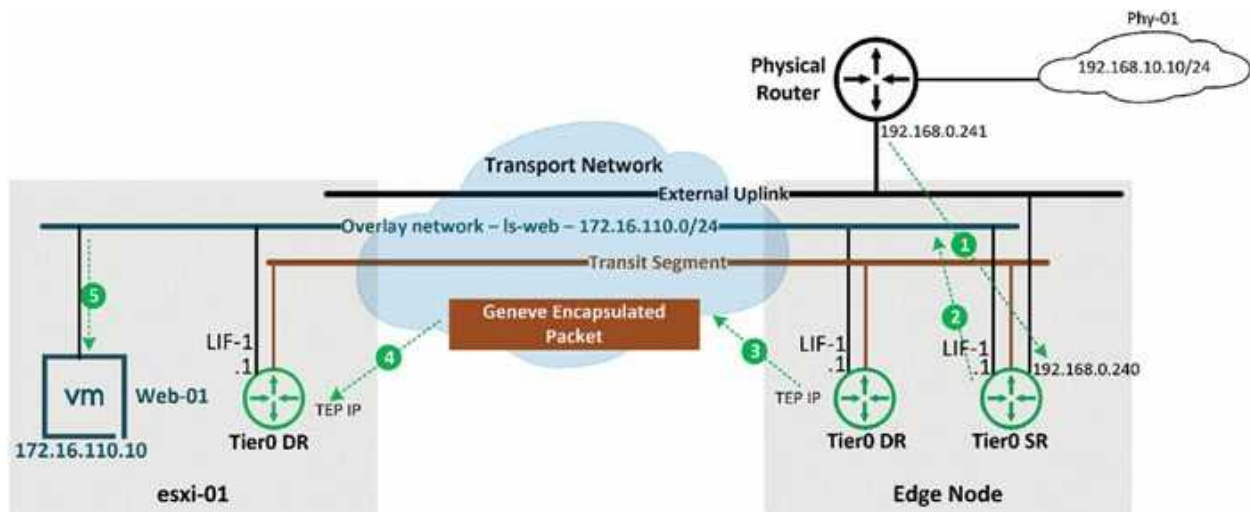
Figure 5.4: North-South packet walk in reverse
