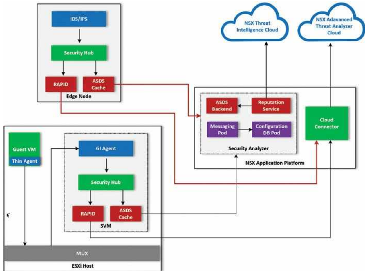
Figure 9.33: NSX Malware Prevention Architecture
