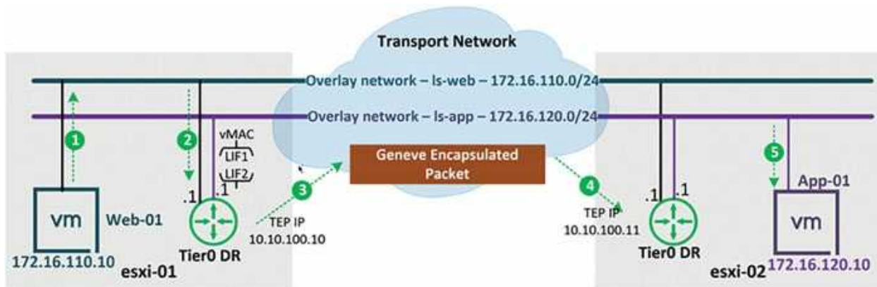
Figure 5.2: East-West Packet walk in single-tier routing
