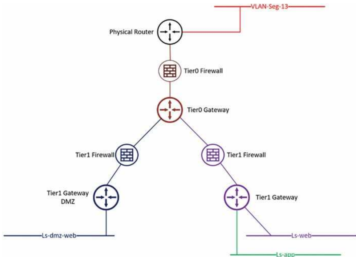
Figure 9.2: Gateway firewall enforcement in NSX
