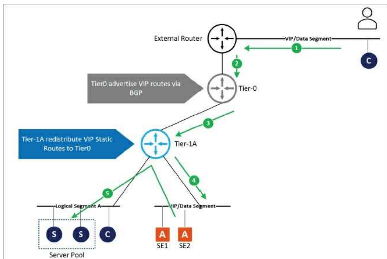
Figure 12.5: North-South Traffic Walk
