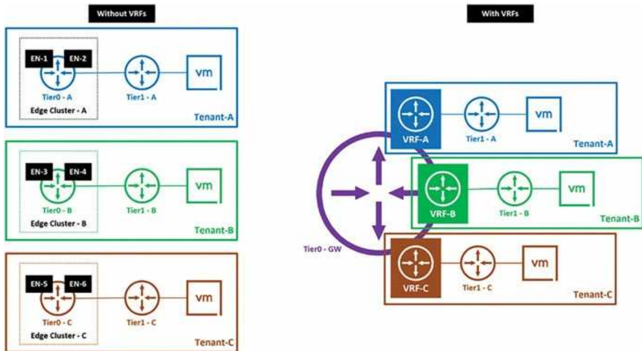
Figure 6.1: VRF gateway hosted on Tier0 gateway
