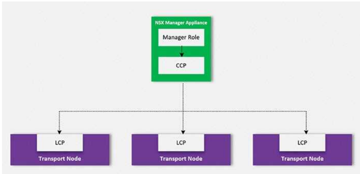
Figure 1.7: NSX Control Plane Architecture
