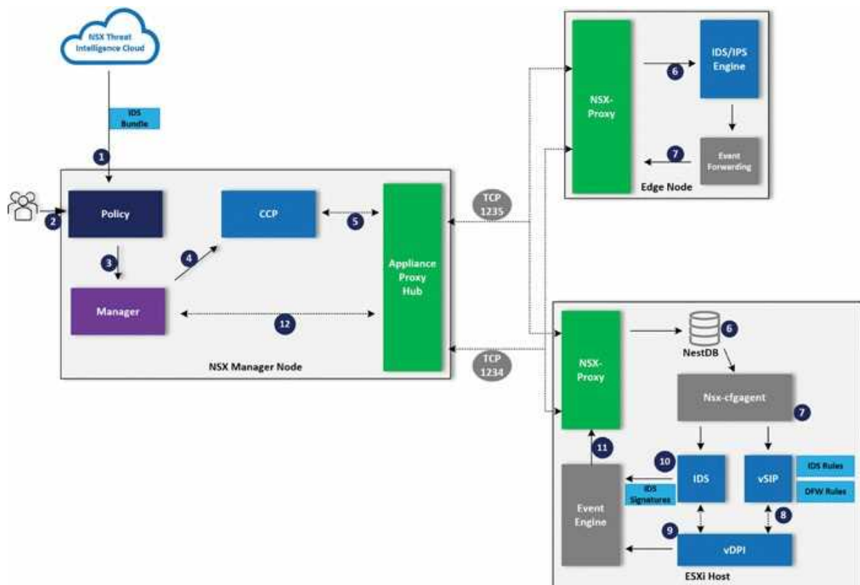
Figure 9.12: NSX IDS/IPS Architecture
