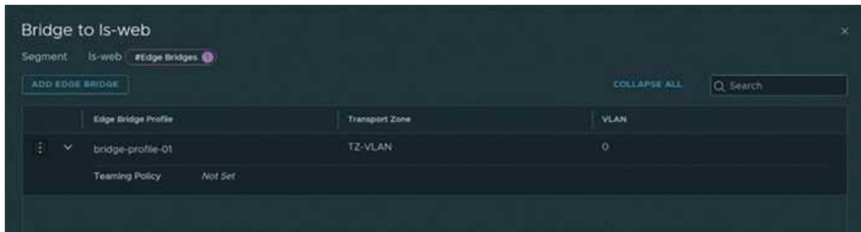
Figure 7.14: NSX Edge bridge added to segment ls-web
