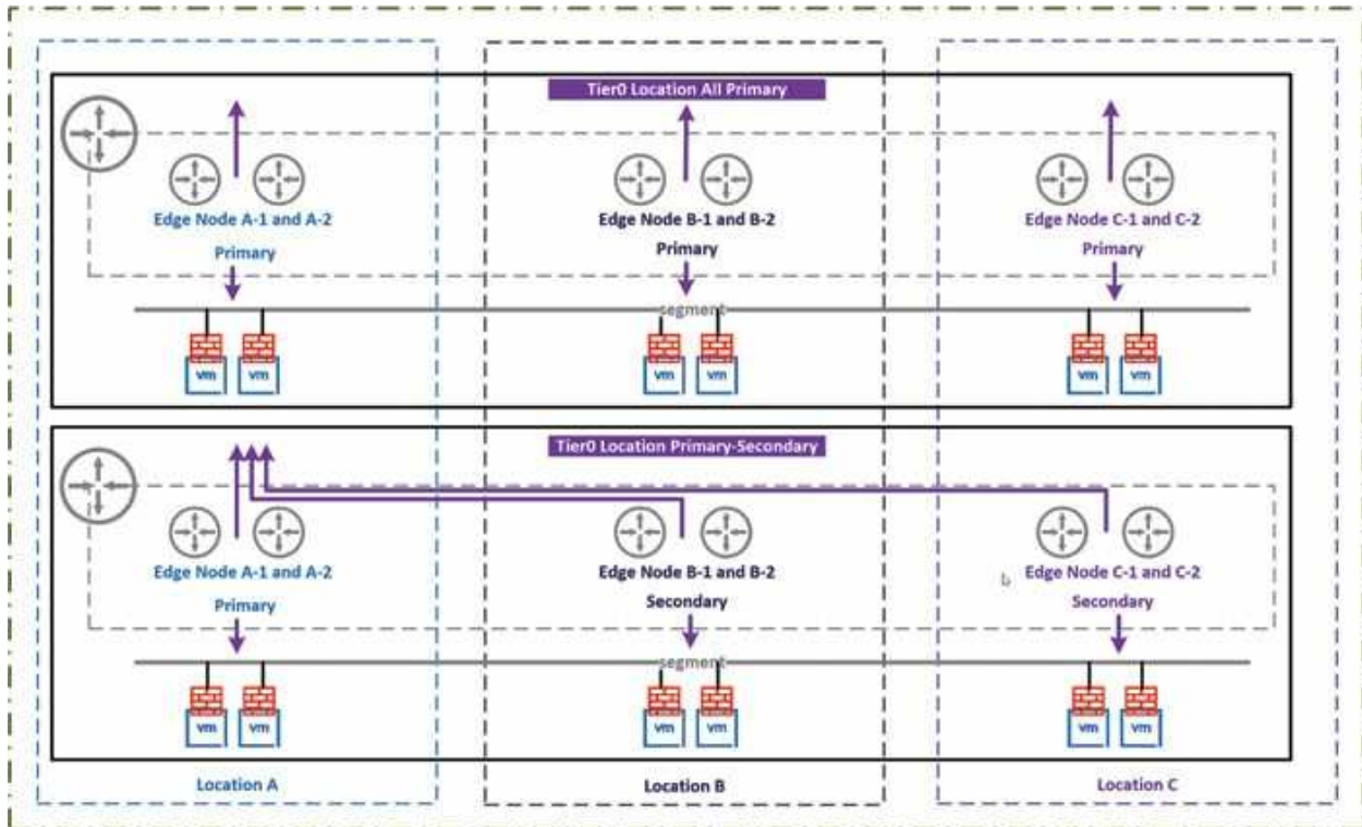
Figure 13.39: Multilocation stretched Tier0 location configurations
