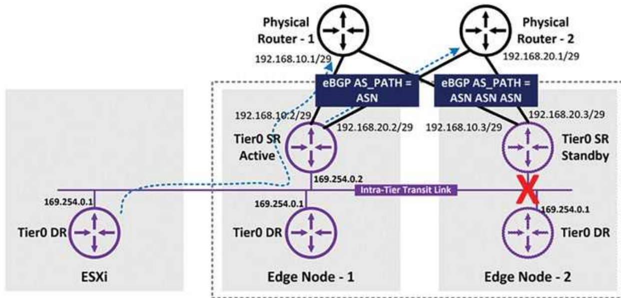
Figure 5.43: BGP configuration in Active-Standby HA mode
