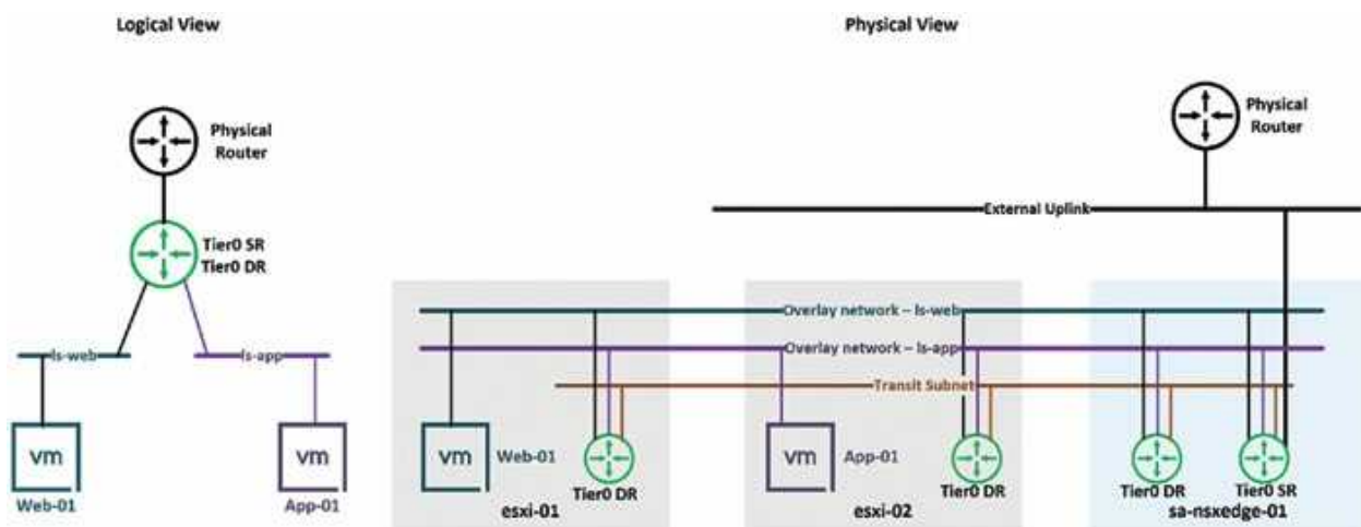
Figure 5.1: Single-Tier Routing Topology
