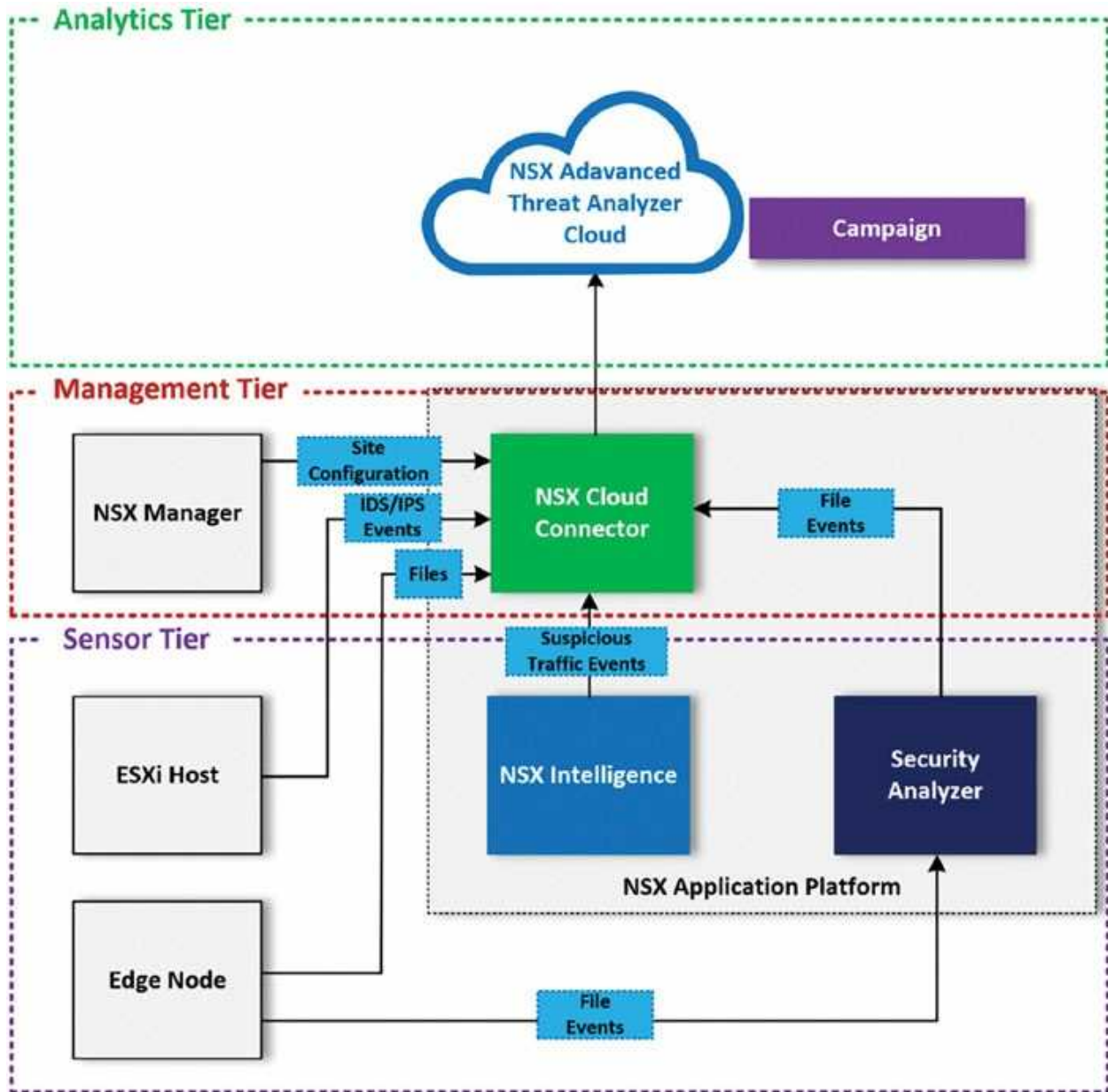
Figure 10.38: Architecture of NSX NDR
