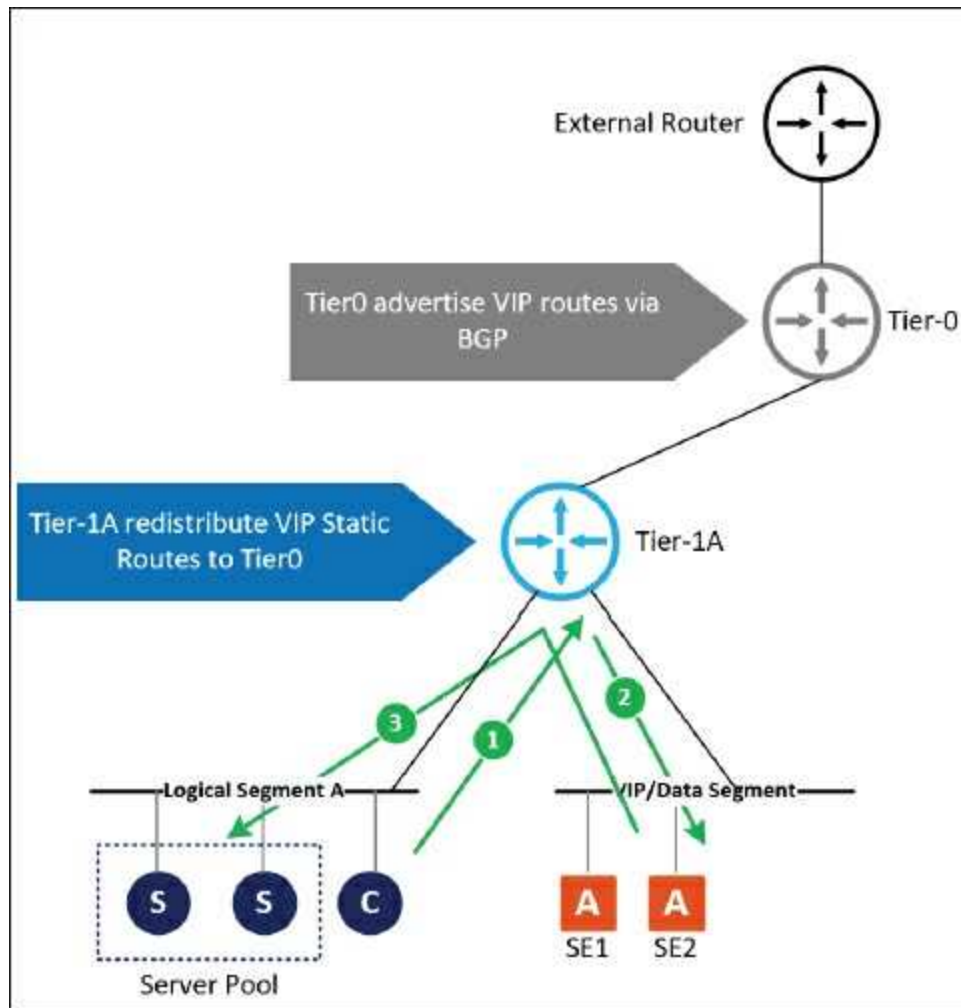
Figure 12.6: East-West Traffic Walk
