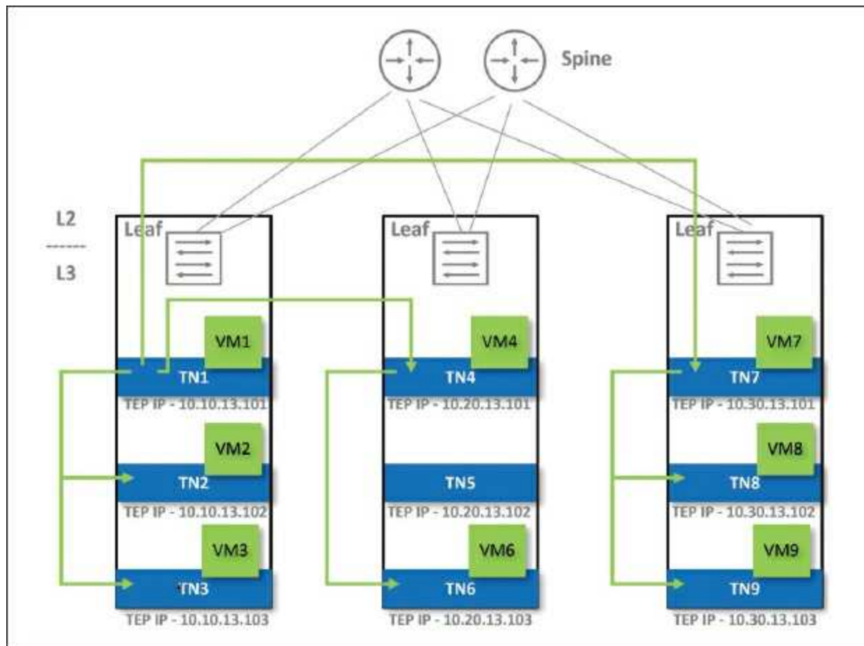
Figure 3.36: Hierarchical Two-Tier Replication method
