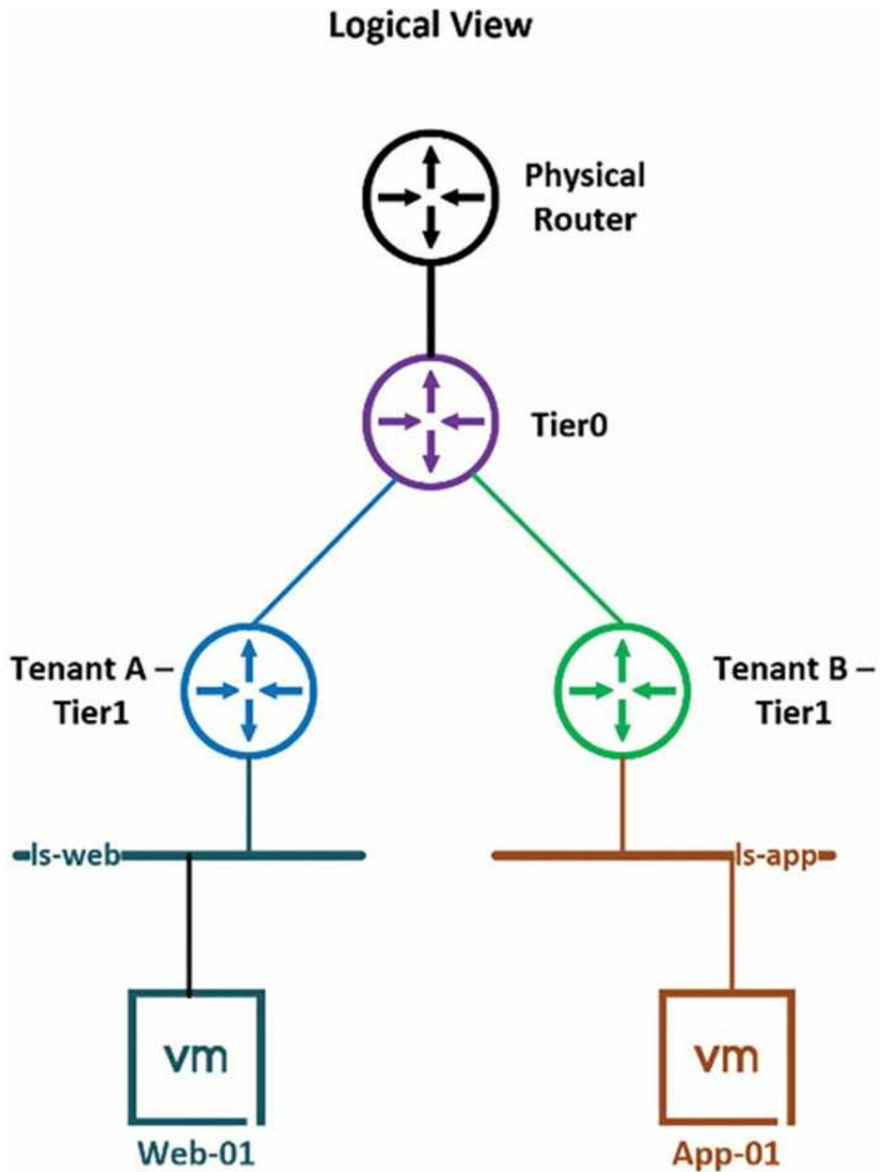
Figure 5.5: An example multi-tier routing topology in NSX
