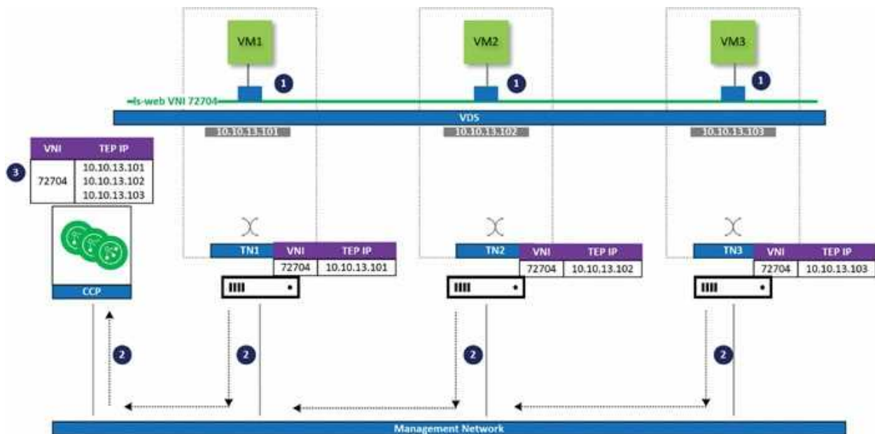
Figure 3.29: TEP table update in NSX environment
