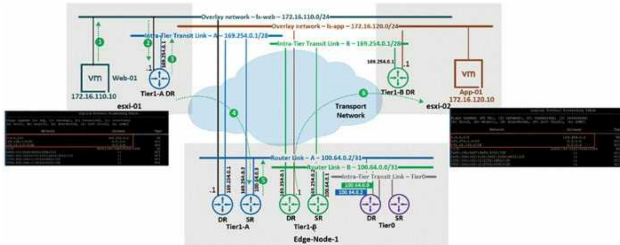
Figure 5.8: Multi-Tier routing packet walk in Tier1 with SR
