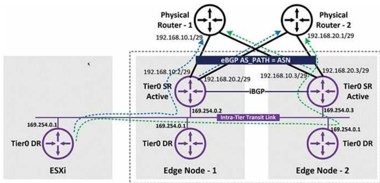
Figure 5.41: BGP configuration in Active-Active HA mode
