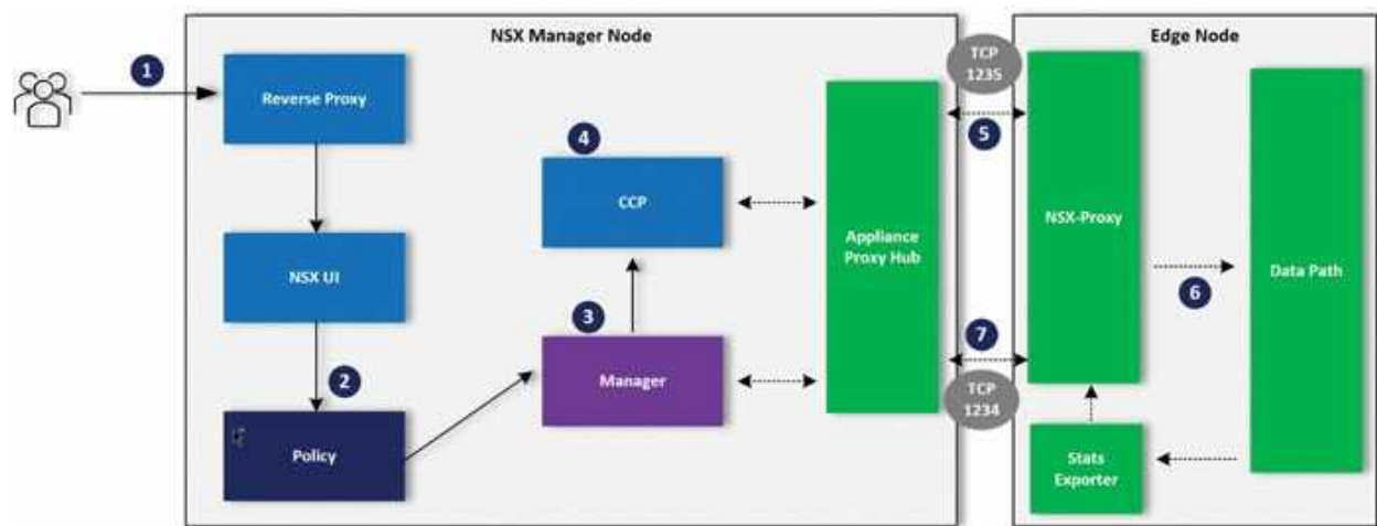
Figure 9.4: NSX Gateway Firewall Architecture
