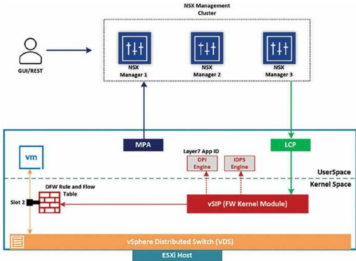
Figure 8.3: NSX DFW Architecture for ESXi host
