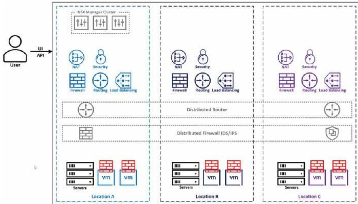
Figure 13.1: NSX Multisite Logical Topology
