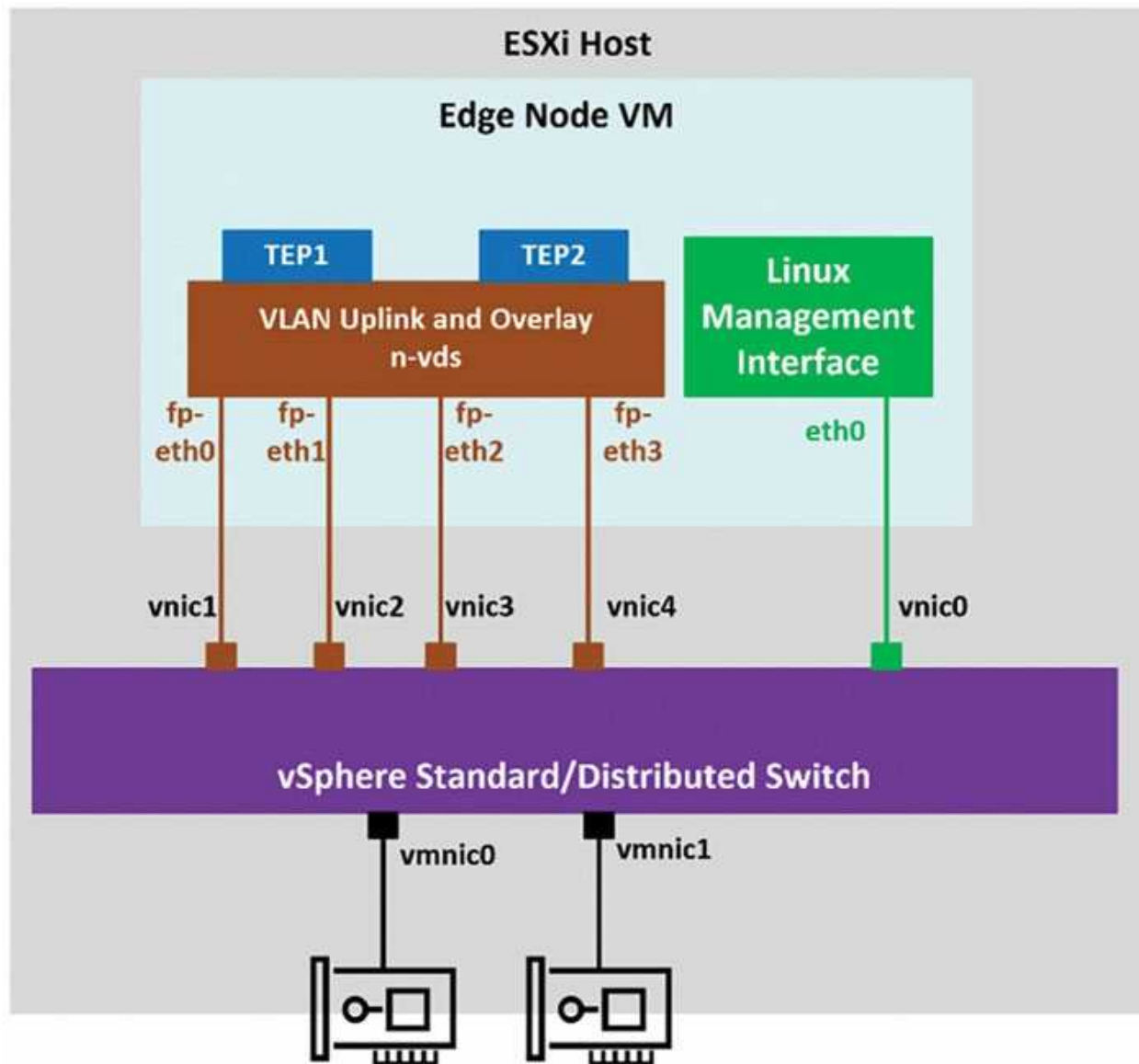
Figure 4.4: Single n-vds configuration on Edge node VM
