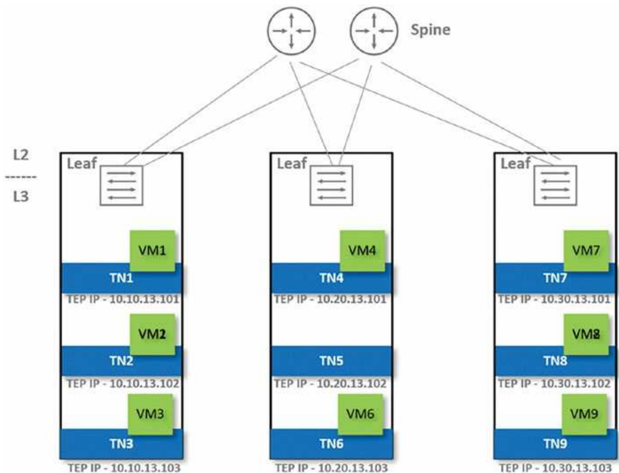
Figure 3.34: BUM traffic in the NSX environment
