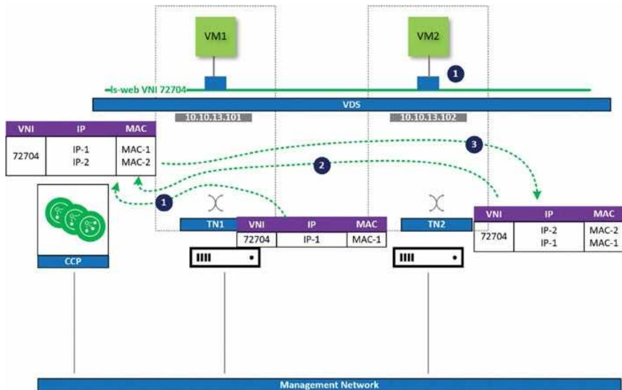
Figure 3.33: ARP table example entries on ESXi host
