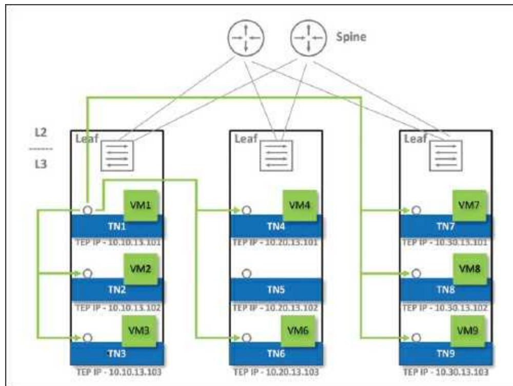
Figure 3.35: Head End Replication mode
