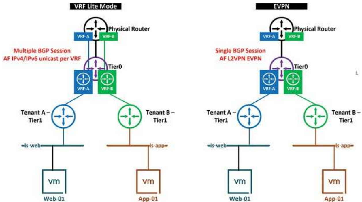
Figure 6.27: VRF Lite vs. EVPN
