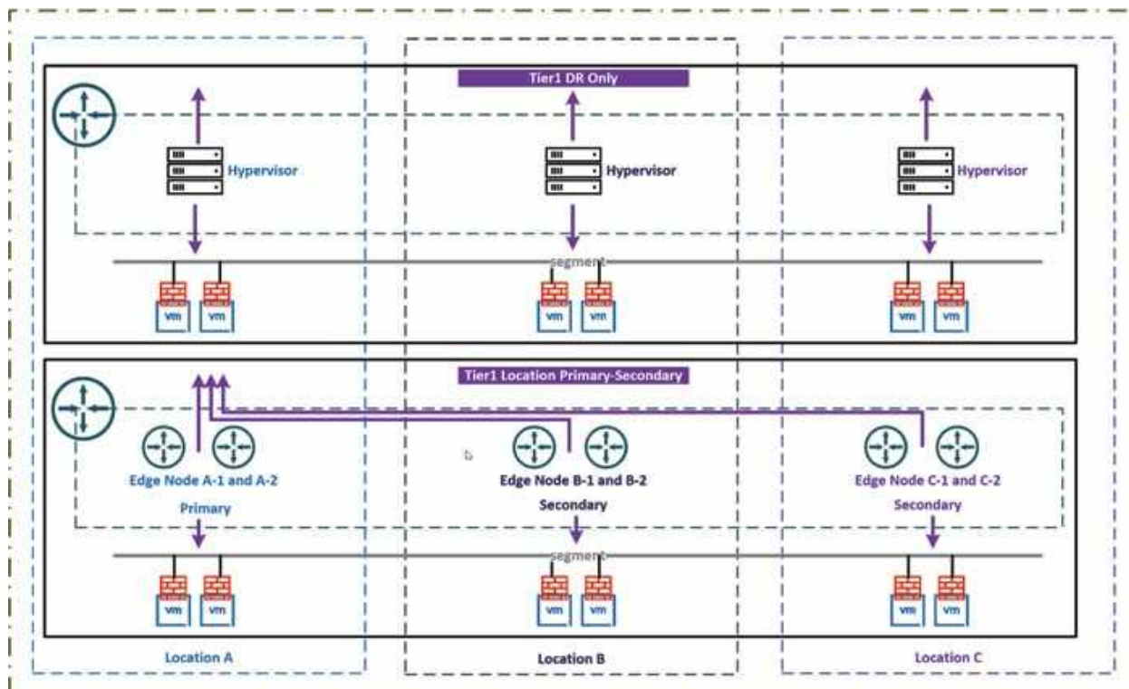
Figure 13.40: Multilocation stretched Tier1 location configuration
