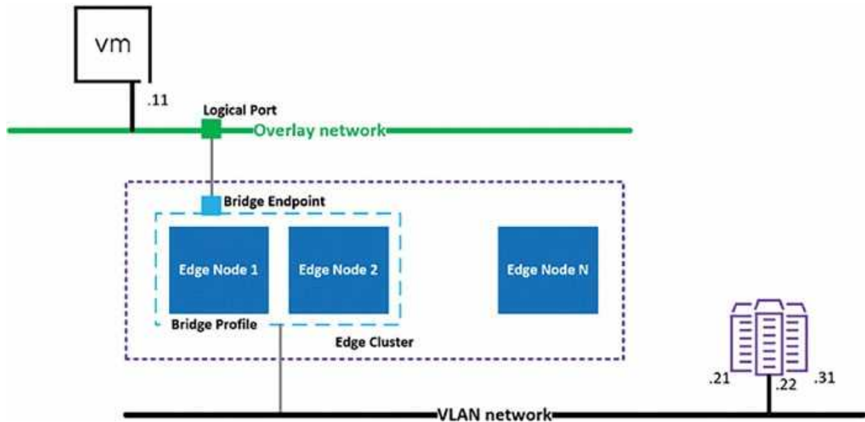
Figure 7.2: NSX Edge Bridge components
