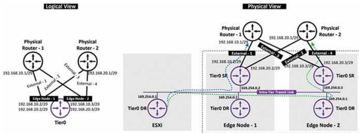
Figure 5.40: Tier0 gateway configured in Active-Active HA mode
