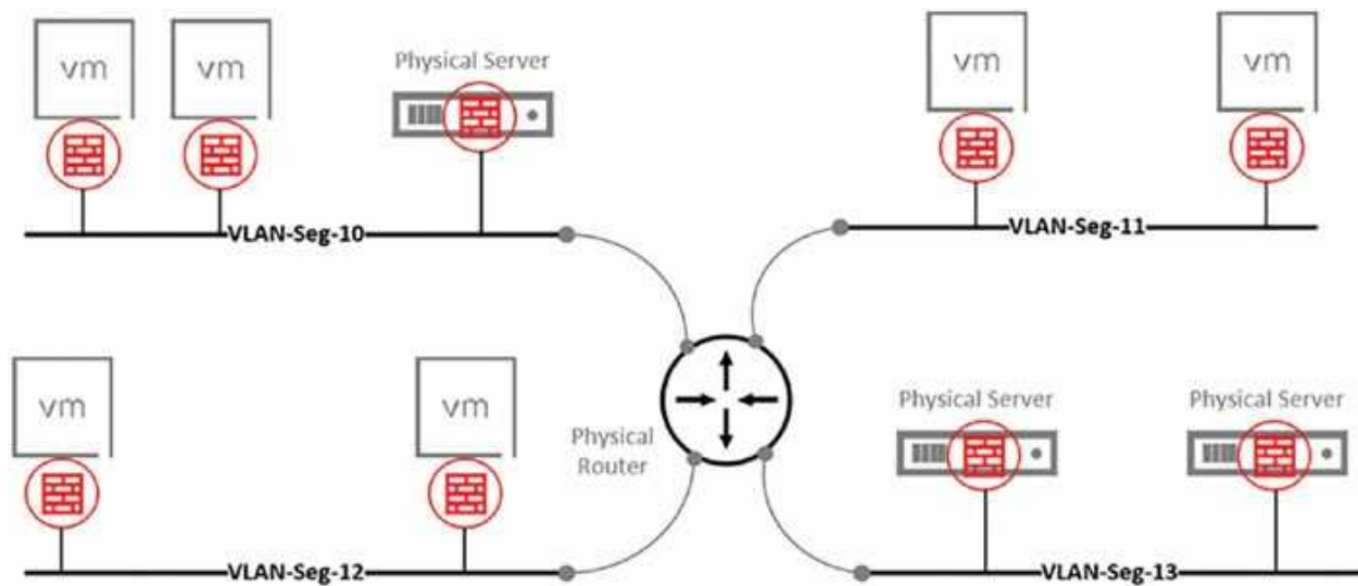
Figure 8.2: NSX distributed firewall applied to workloads
