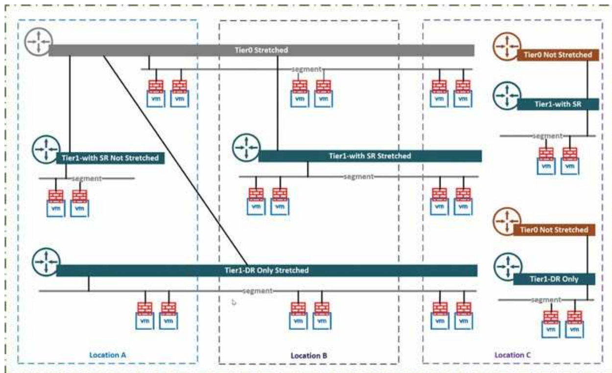
Figure 13.37: Different network topologies in NSX Federation
