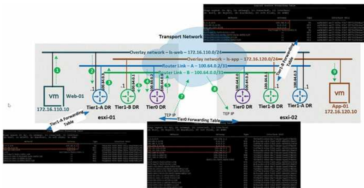
Figure 5.7: Multi-Tier routing topology packet walk with Tier1 in DR only
