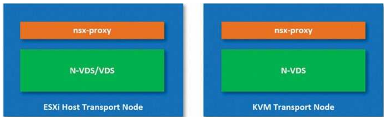
Figure 2.22: Transport Node architecture for ESXi host and KVM host
