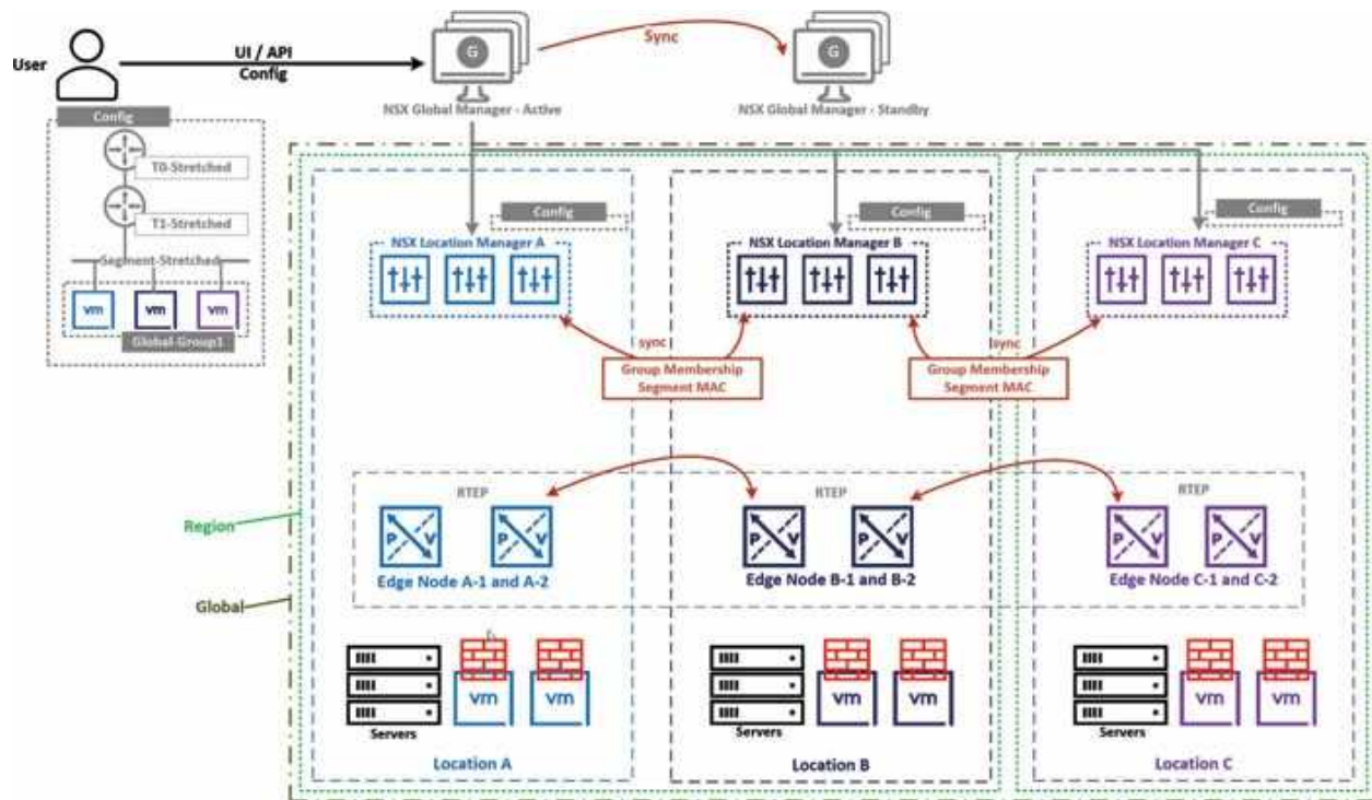
Figure 13.3: NSX Federation Architecture
