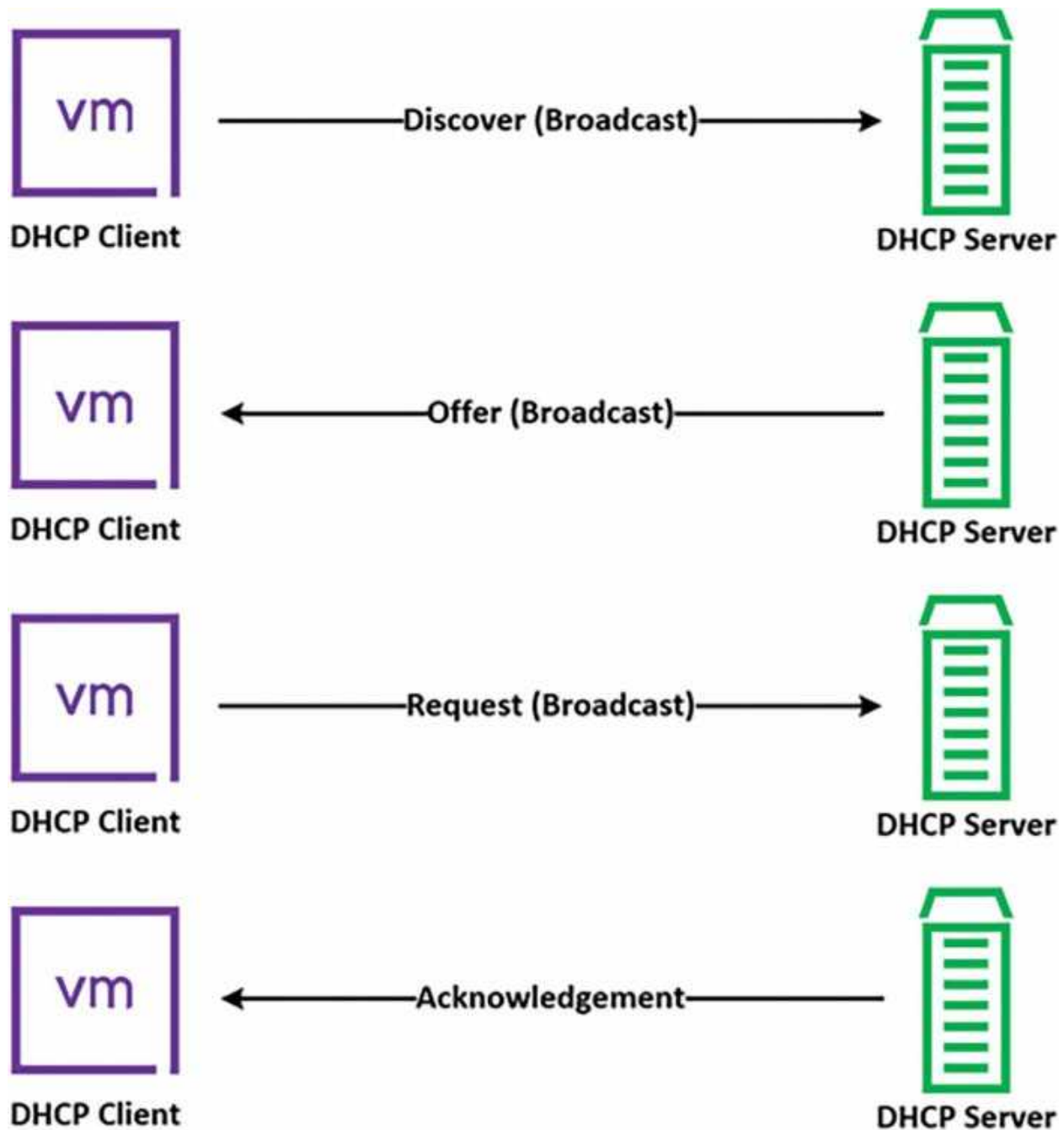
Figure 11.22: DHCP process to assign network configuration to DHCP client
