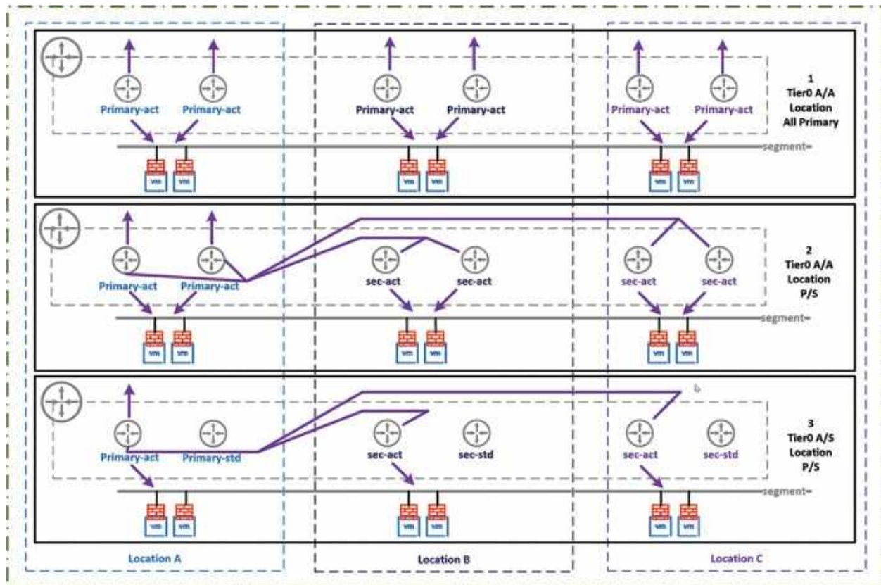
Figure 13.41: Tier0 HA configuration with multiple locations
