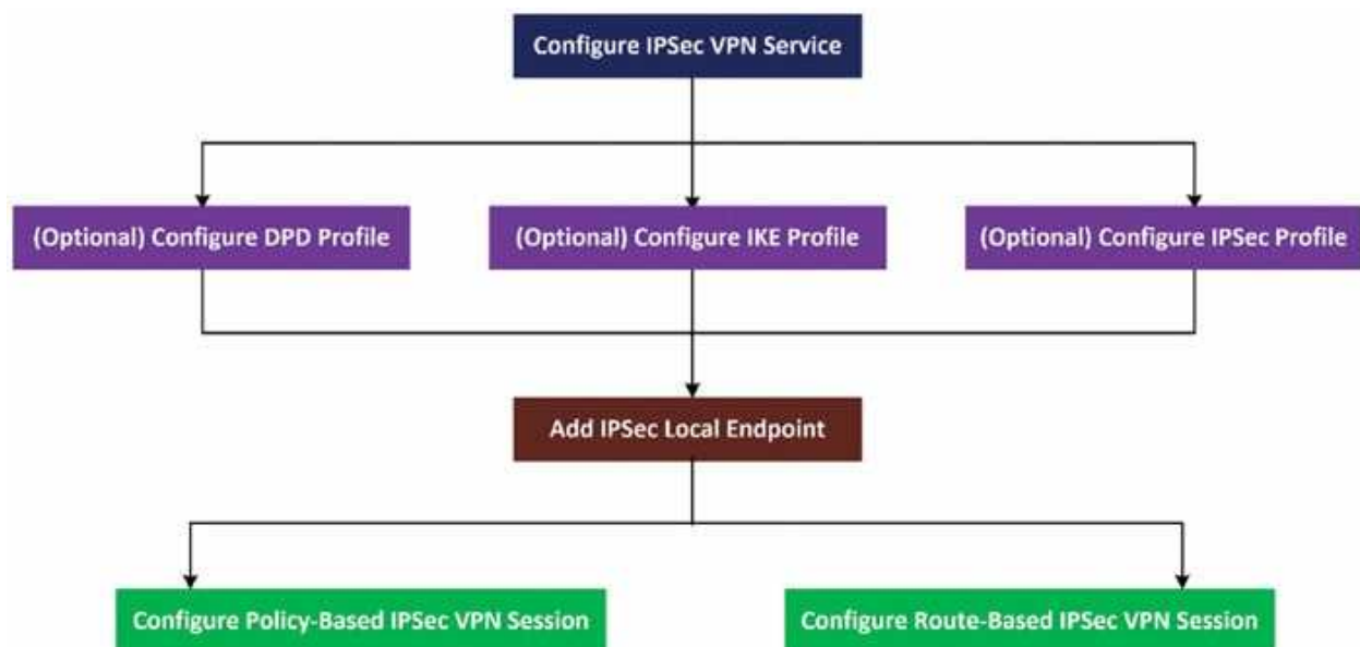
Figure 11.48: High-level workflow to configure IPsec VPN
