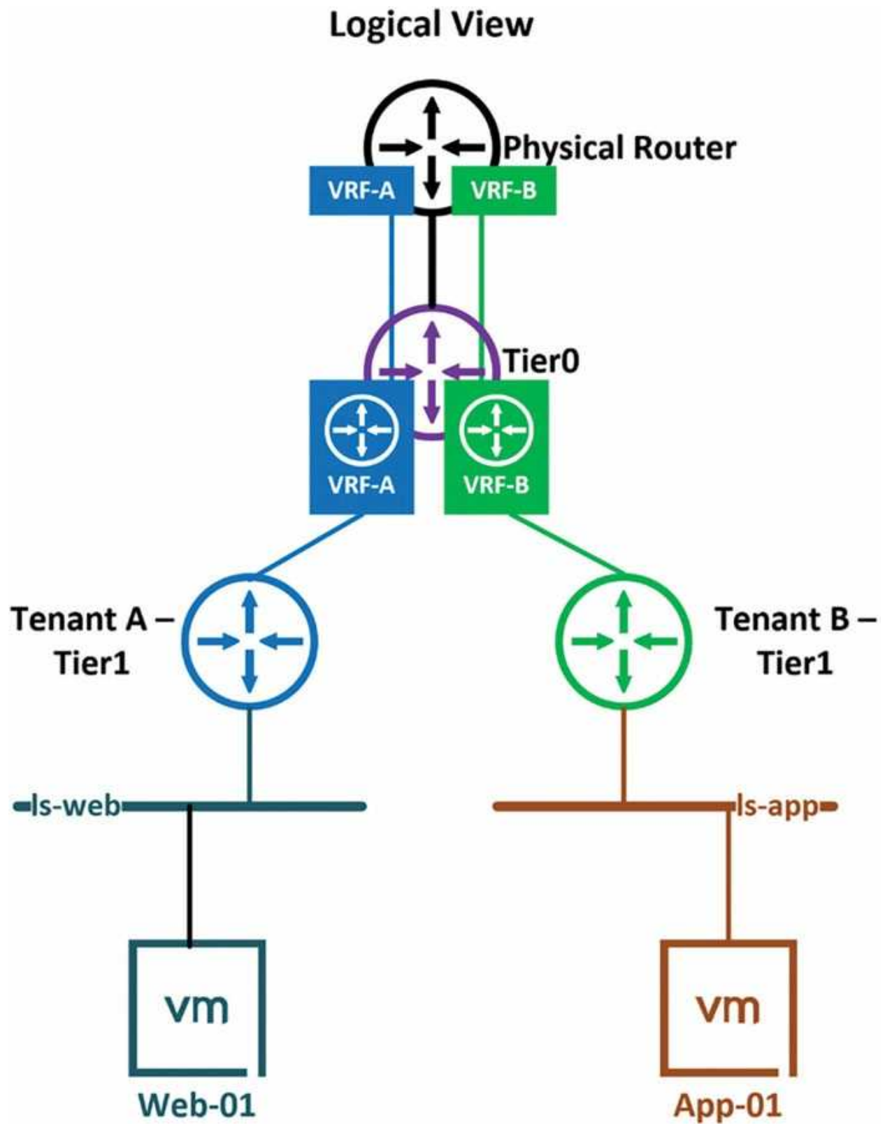
Figure 6.3: An example VRF topology
