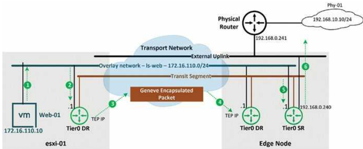
Figure 5.3: North-South Packet Walk in Single-Tier Routing
