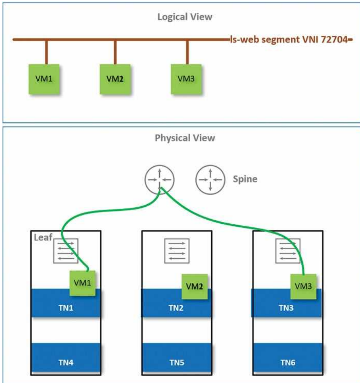
Figure 3.2: VMs belonging to the same overlay segment running on different Transport Nodes
