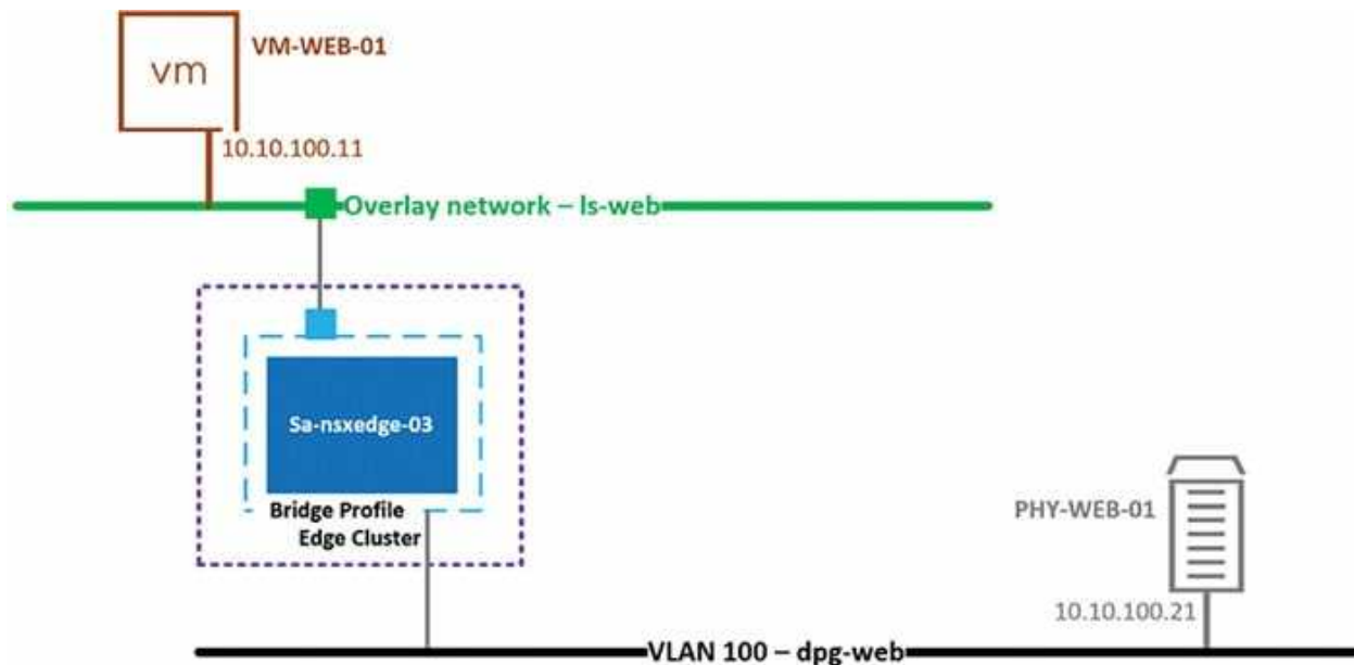
Figure 7.4: Setting up NSX Edge bridge between overlay and VLAN network
