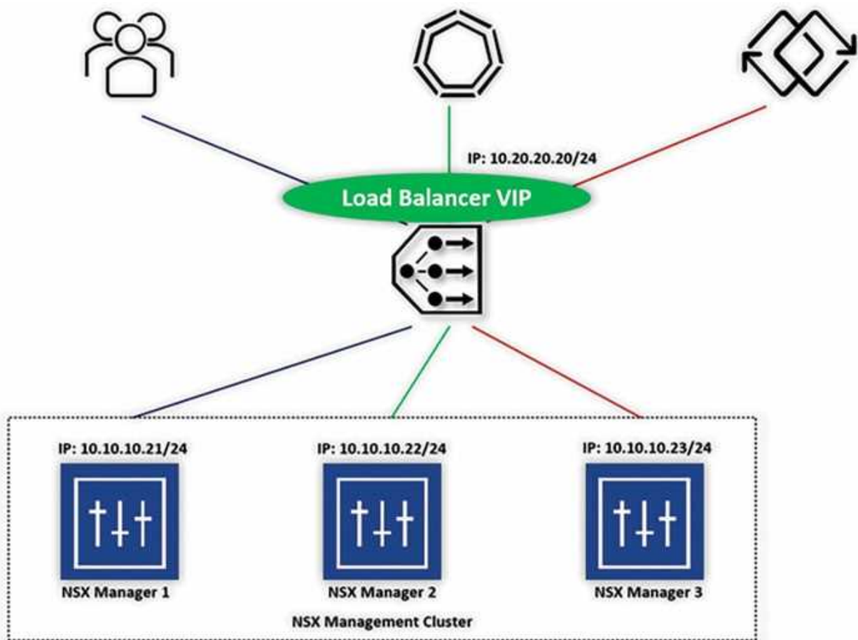
Figure 2.21: NSX Management cluster with an external Load balancer
