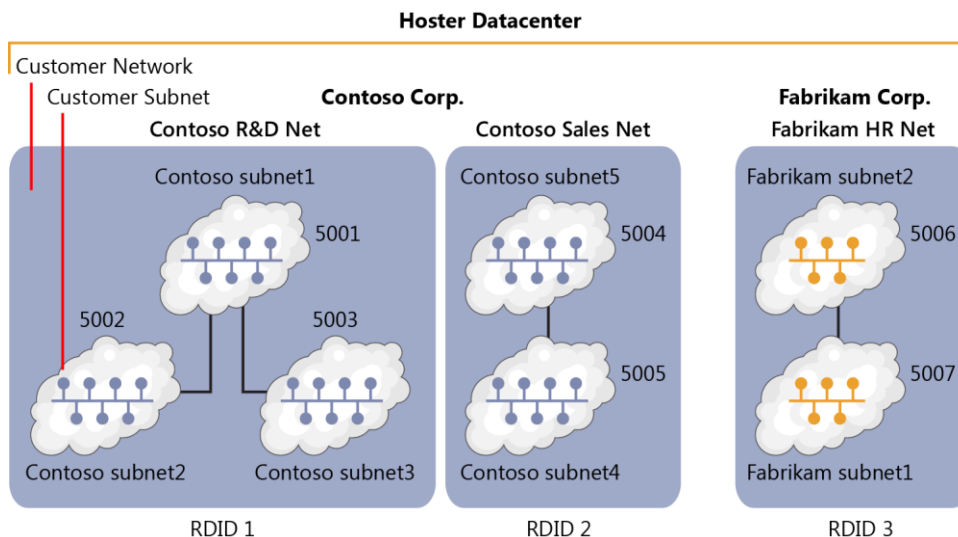
Figure 4-1 Network virtualization
