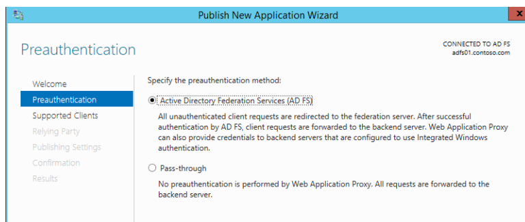
Figure 4-8: Preauthentication selection
