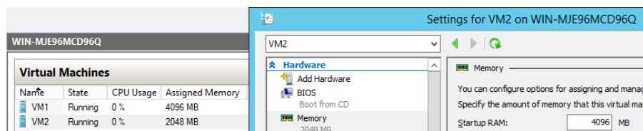
Figure 2-47: VM memory settings changing while running
